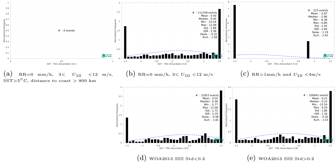
Figure 15: Normalized histogram of \Delta\text{SSS} (SMAP SSS L2 v5.3 - 40 km (RSS) - TSG (Amundsen)) for 5 different subdatasets corresponding to: RR=0 mm/h, 3 < U_{10} < 12 m/s, SST > 5^{\circ}\text{C} , distance to coast > 800 km (a), RR=0 mm/h, 3 < U_{10} < 12 m/s (b), RR > 1\text{mm/h} and U_{10} < 4\text{m/s} (c), WOA2013 SSS \text{Std} < 0.2 (d), WOA2013 SSS \text{Std} > 0.2 (e).
