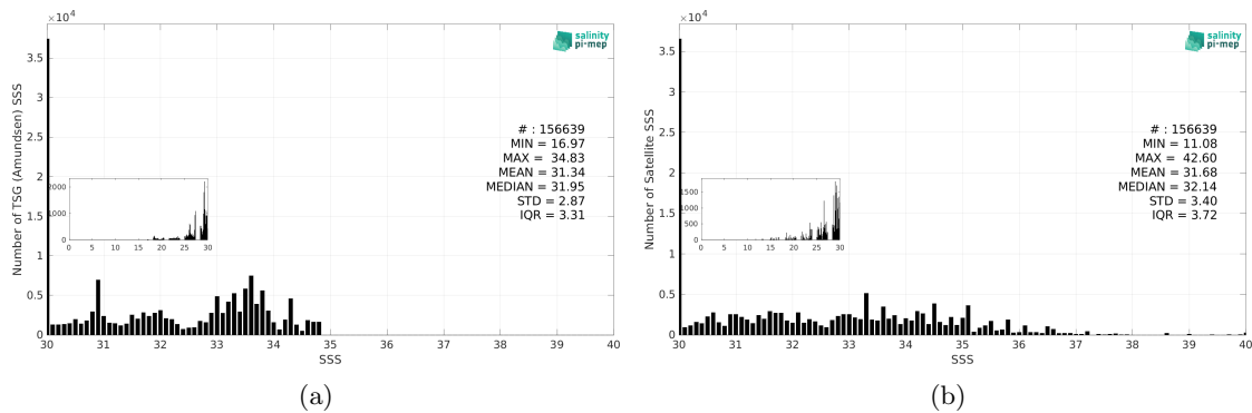
Figure 3: Histograms of SSS from TSG (Amundsen) (a) and SMAP SSS L2 v5.3 - 40 km (RSS) (b) considering all match-up pairs per bins of 0.1 over the Global Ocean Pi-MEP region and for the full satellite product period.
