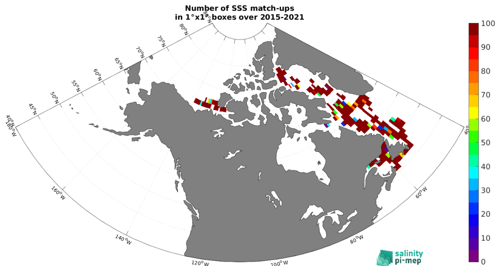
Figure 5: Number of SSS match-ups between TSG (Amundsen) SSS and the SMAP SSS L2 v5.3 - 40 km (RSS) SSS product for the Global Ocean Pi-MEP region over 1^\circ \times 1^\circ boxes and for the full satellite product period.
