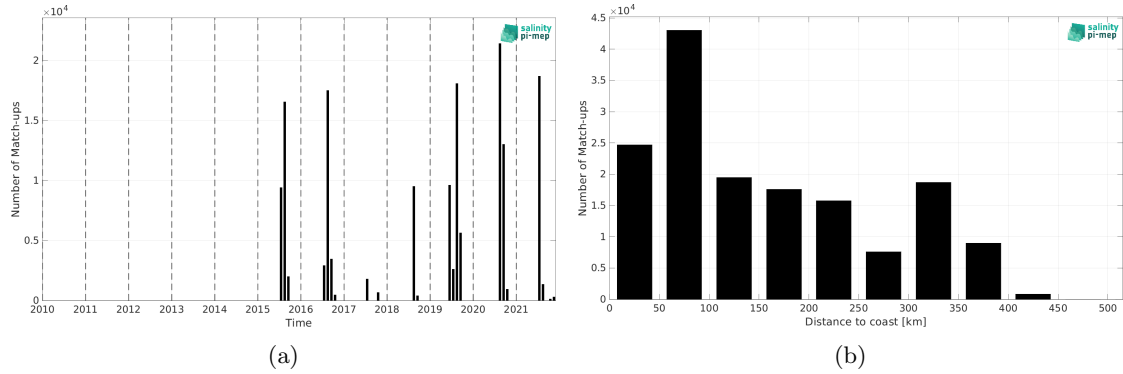
Figure 2: Number of match-ups between TSG (Amundsen) and SMAP SSS L2 v5.3 - 40 km (RSS) SSS as a function of time (a) and as function of the distance to coast (b) over the Global Ocean Pi-MEP region and for the full satellite product period.
