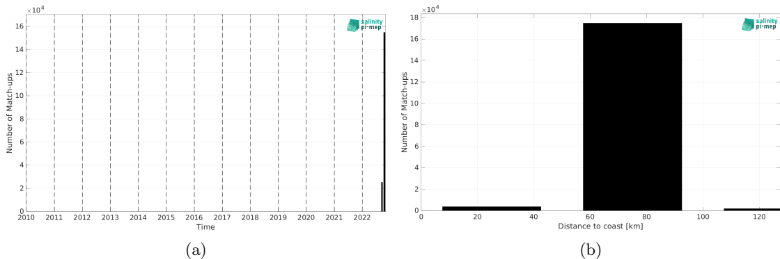
Figure 2: Number of match-ups between SASSIE and SMAP SSS L2 v5.3 - 40 km (RSS) SSS as a function of time (a) and as function of the distance to coast (b) over the Global Ocean Pi-MEP region and for the full satellite product period.
