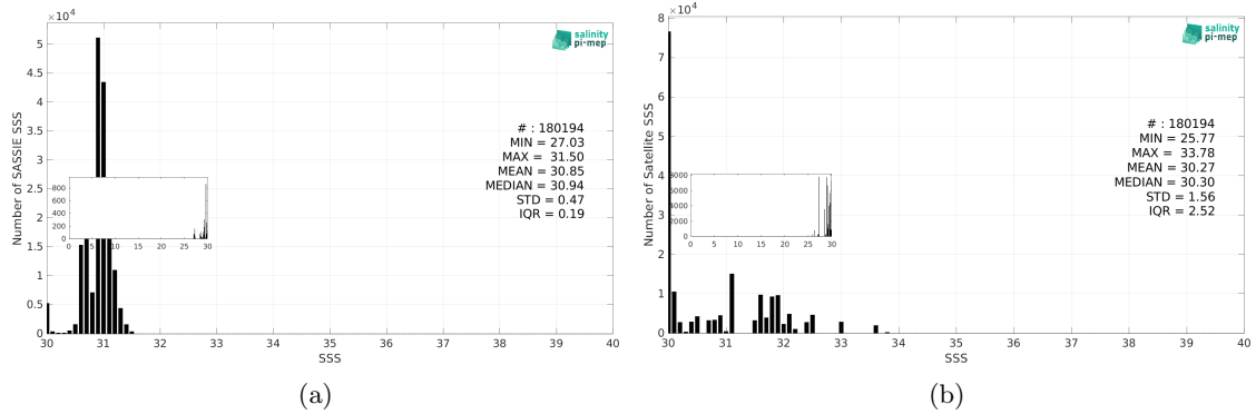
Figure 3: Histograms of SSS from SASSIE (a) and SMAP SSS L2 v5.3 - 40 km (RSS) (b) considering all match-up pairs per bins of 0.1 over the Global Ocean Pi-MEP region and for the full satellite product period.
