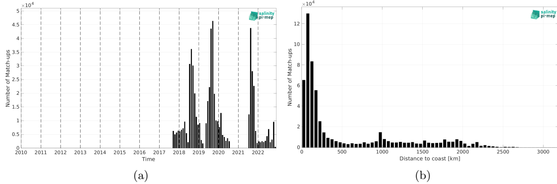
Figure 2: Number of match-ups between Sailldrone and SMAP SSS L2 v5.3 - 40 km (RSS) SSS as a function of time (a) and as function of the distance to coast (b) over the Global Ocean Pi-MEP region and for the full satellite product period.
