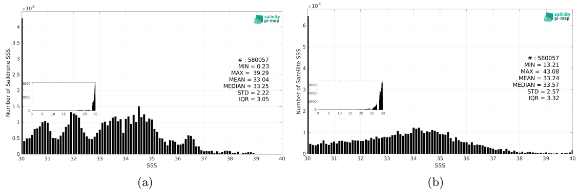
Figure 3: Histograms of SSS from Sailldrone (a) and SMAP SSS L2 v5.3 - 40 km (RSS) (b) considering all match-up pairs per bins of 0.1 over the Global Ocean Pi-MEP region and for the full satellite product period.
