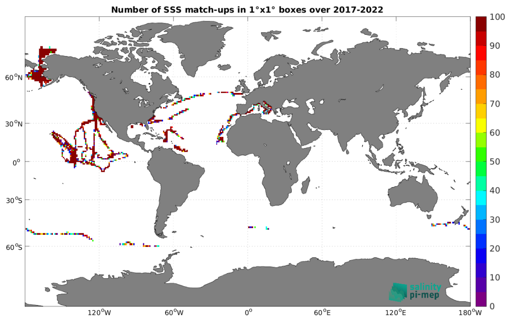
Figure 5: Number of SSS match-ups between Saildrone SSS and the SMAP SSS L2 v5.3 - 40 km (RSS) SSS product for the Global Ocean Pi-MEP region over 1^\circ \times 1^\circ boxes and for the full satellite product period.
