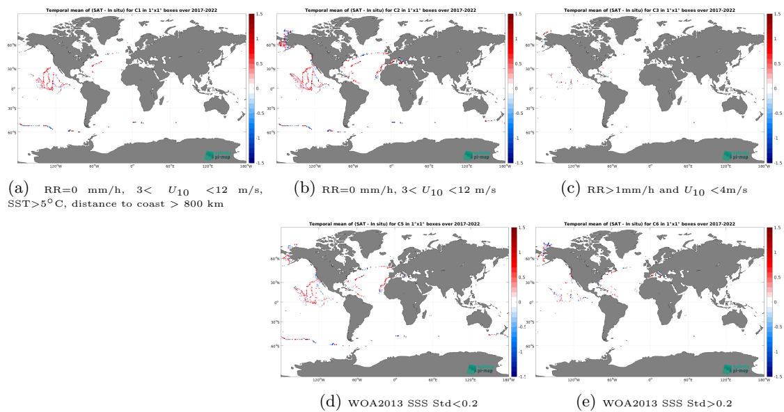
Figure 14: Temporal mean gridded over spatial boxes of size 1^\circ \times 1^\circ of \Delta SSS (SMAP SSS L2 v5.3 - 40 km (RSS) - Saildrone) for 5 different subdatasets corresponding to:RR=0 mm/h, 3 < U_{10} < 12 m/s, SST > 5^\circ\text{C} , distance to coast > 800 km (a), RR=0 mm/h, 3 < U_{10} < 12 m/s (b), RR > 1 mm/h and U_{10} < 4 m/s (c), WOA2013 SSS Std < 0.2 (d), WOA2013 SSS Std > 0.2 (e).
