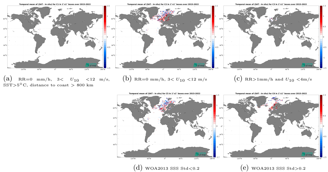
Figure 14: Temporal mean gridded over spatial boxes of size 1^\circ \times 1^\circ of \Delta SSS (SMAP SSS L2 v5.3 - 40 km (RSS) - ICES) for 5 different subdatasets corresponding to:RR=0 mm/h, 3 < U_{10} < 12 m/s, SST > 5°C, distance to coast > 800 km (a), RR=0 mm/h, 3 < U_{10} < 12 m/s (b), RR > 1mm/h and U_{10} < 4 m/s (c), WOA2013 SSS Std < 0.2 (d), WOA2013 SSS Std > 0.2 (e).
