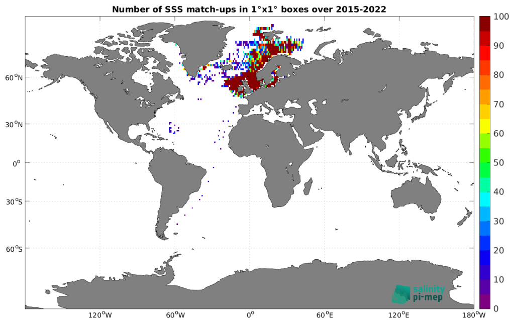
Figure 5: Number of SSS match-ups between ICES SSS and the SMAP SSS L2 v5.3 - 40 km (RSS) SSS product for the Global Ocean Pi-MEP region over 1^\circ \times 1^\circ boxes and for the full satellite product period.
