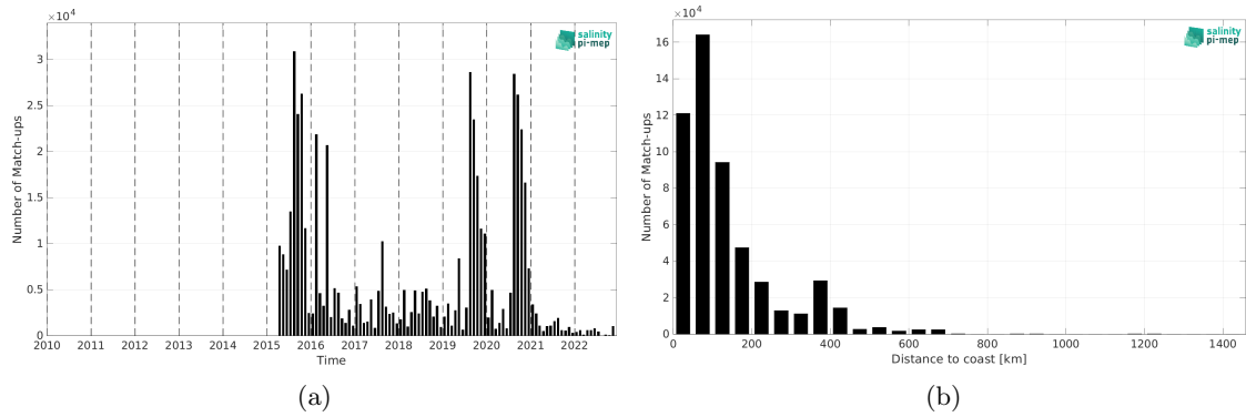
Figure 2: Number of match-ups between ICES and SMAP SSS L2 v5.3 - 40 km (RSS) SSS as a function of time (a) and as function of the distance to coast (b) over the Global Ocean Pi-MEP region and for the full satellite product period.
