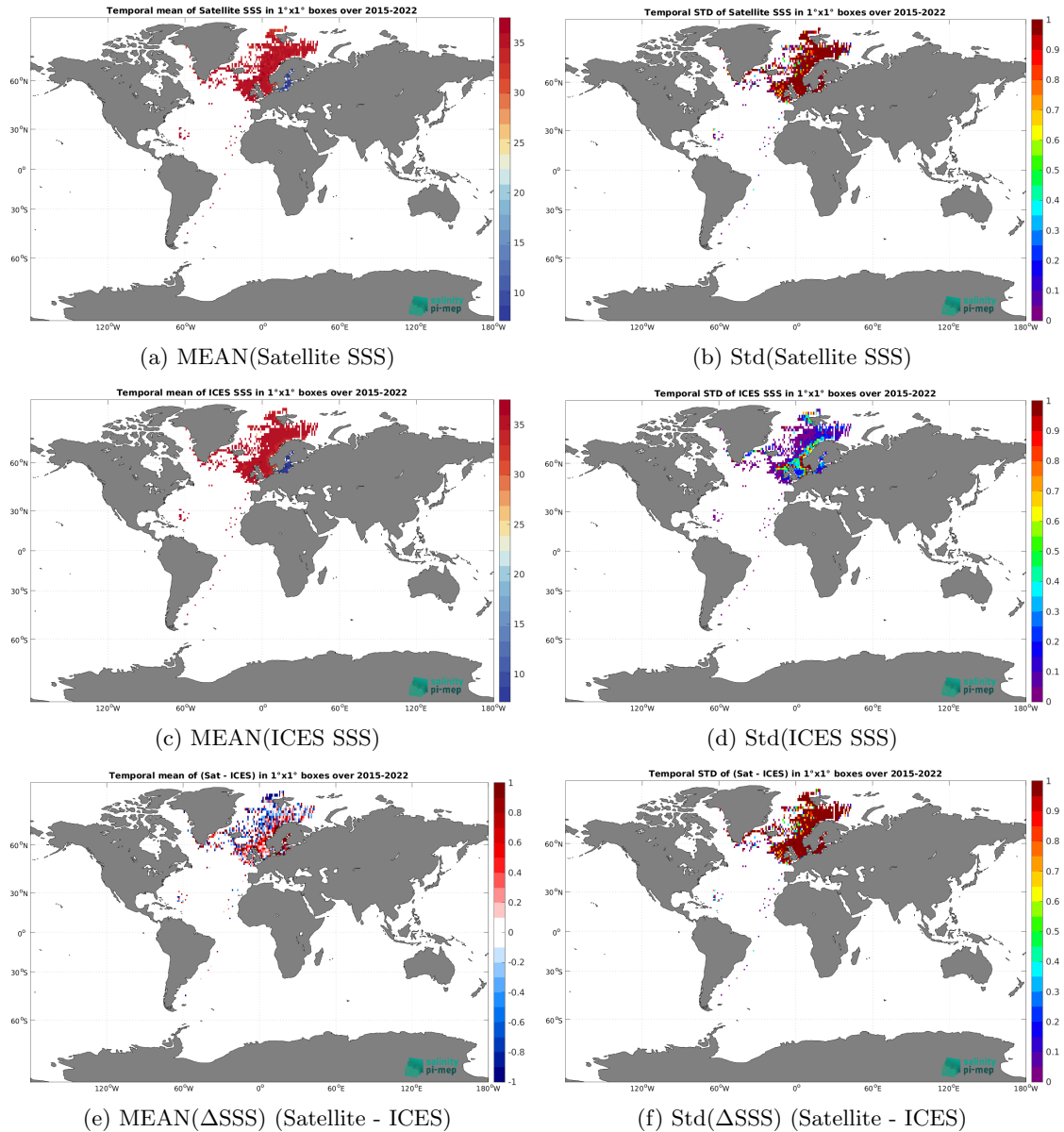
Figure 7: Temporal mean (left) and Std (right) of SSS from SMAP SSS L2 v5.3 - 40 km (RSS) (top), ICES (middle), and of \Delta SSS (Satellite - ICES). Only match-up pairs are used to generate these maps.
