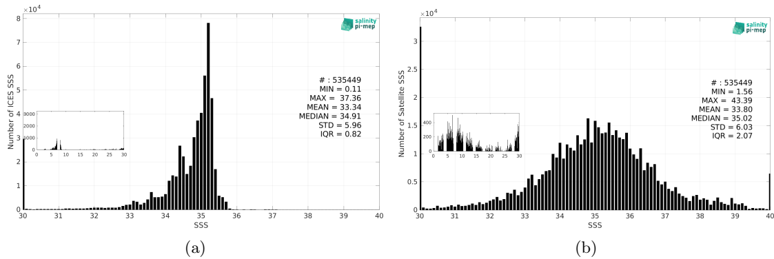
Figure 3: Histograms of SSS from ICES (a) and SMAP SSS L2 v5.3 - 40 km (RSS) (b) considering all match-up pairs per bins of 0.1 over the Global Ocean Pi-MEP region and for the full satellite product period.
