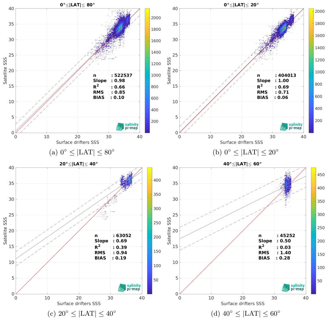
Figure 9: Contour maps of the concentration of SMAP SSS L2 v5.3 - 40 km (RSS) SSS (y-axis) versus Surface drifters SSS (x-axis) at match-up pairs for different latitude bands. For each plot, the red line shows x=y . The black thin and dashed lines indicate a linear fit through the data cloud and the \pm 95\% confidence levels, respectively. The number match-up pairs n , the slope and R^2 coefficient of the linear fit, the root mean square (RMS) and the mean bias between satellite and in situ data are indicated for each latitude band in each plots.
