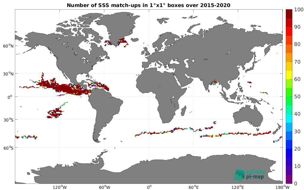
Figure 4: Number of SSS match-ups between Surface drifters SSS and the SMAP SSS L2 v5.3 - 40 km (RSS) SSS product for the Global Ocean Pi-MEP region over 1^\circ \times 1^\circ boxes and for the full satellite product period.
