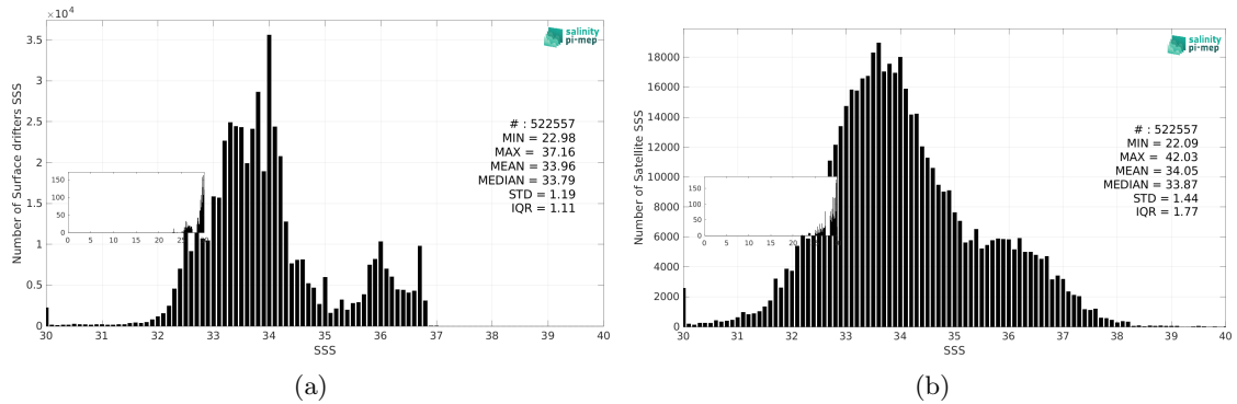
Figure 3: Histograms of SSS from Surface drifters (a) and SMAP SSS L2 v5.3 - 40 km (RSS) (b) considering all match-up pairs per bins of 0.1 over the Global Ocean Pi-MEP region and for the full satellite product period.
