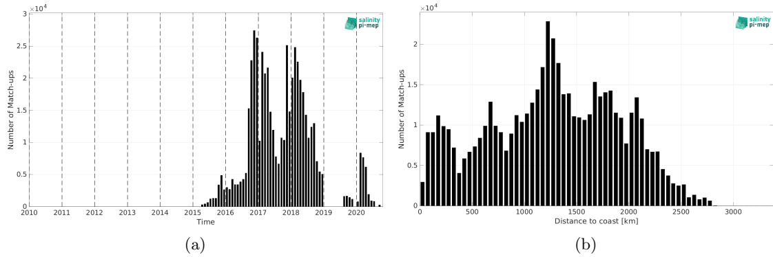
Figure 2: Number of match-ups between Surface drifters and SMAP SSS L2 v5.3 - 40 km (RSS) SSS as a function of time (a) and as function of the distance to coast (b) over the Global Ocean Pi-MEP region and for the full satellite product period.
