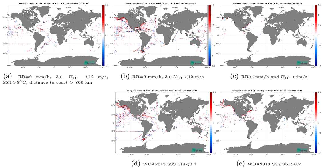
Figure 12: Temporal mean gridded over spatial boxes of size 1^\circ \times 1^\circ of \Delta SSS (SMAP SSS L2 v5 - 40 km (RSS) - TSG (SAMOS)) for 5 different subdatasets corresponding to:RR=0 mm/h, 3 < U_{10} < 12 m/s, SST > 5^\circ\text{C} , distance to coast > 800 km (a), RR=0 mm/h, 3 < U_{10} < 12 m/s (b), RR > 1 mm/h and U_{10} < 4 m/s (c), WOA2013 SSS Std < 0.2 (d), WOA2013 SSS Std > 0.2 (e).
