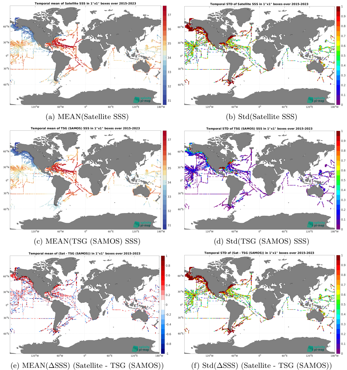
Figure 6: Temporal mean (left) and Std (right) of SSS from SMAP SSS L2 v5 - 40 km (RSS) (top), TSG (SAMOS) (middle), and of \Delta SSS (Satellite - TSG (SAMOS)). Only match-up pairs are used to generate these maps.
