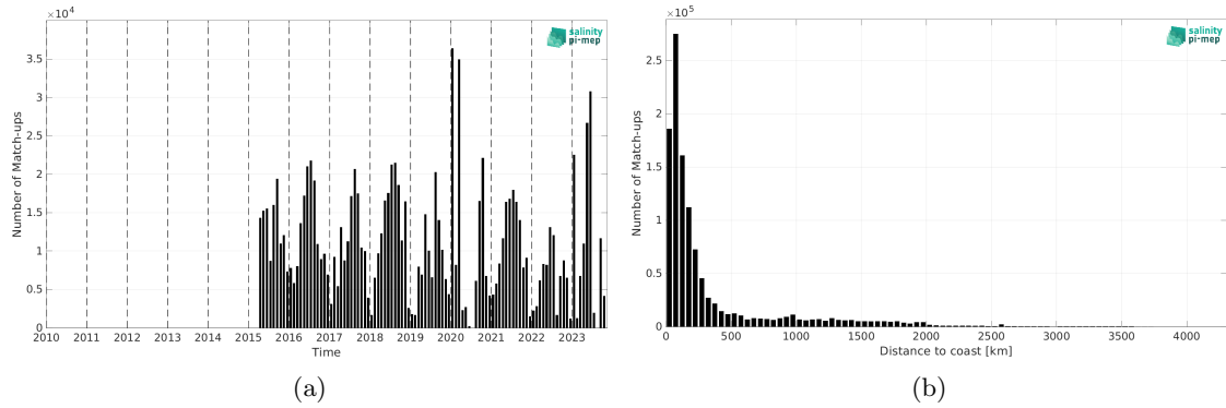
Figure 1: Number of match-ups between TSG (SAMOS) and SMAP SSS L2 v5 - 40 km (RSS) SSS as a function of time (a) and as function of the distance to coast (b) over the Global Ocean Pi-MEP region and for the full satellite product period.
