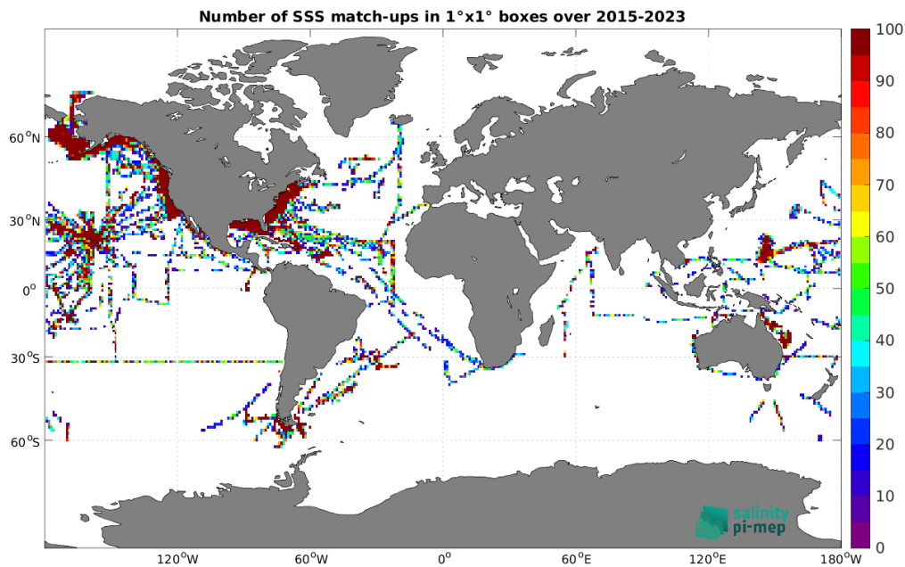
Figure 4: Number of SSS match-ups between TSG (SAMOS) SSS and the SMAP SSS L2 v5 - 40 km (RSS) SSS product for the Global Ocean Pi-MEP region over 1^\circ \times 1^\circ boxes and for the full satellite product period.
