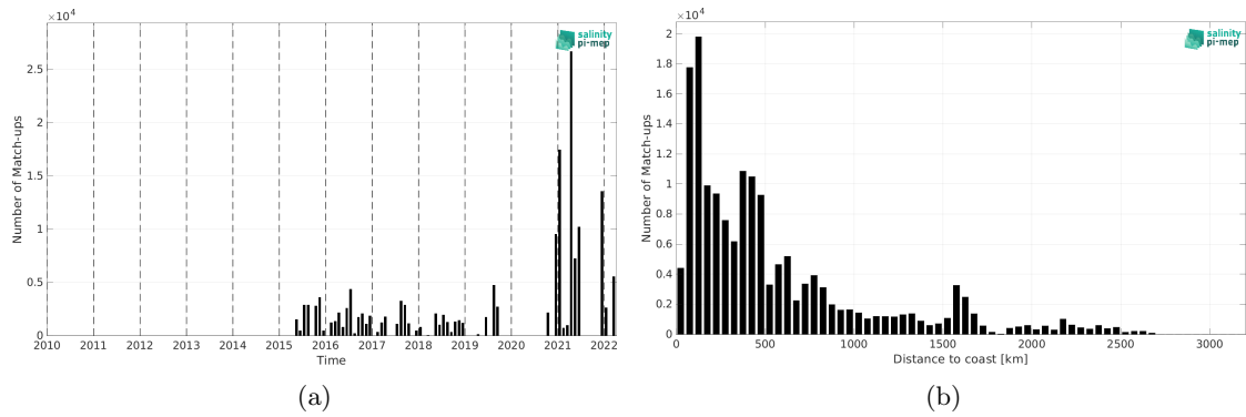
Figure 1: Number of match-ups between TSG (Polarstern) and SMAP SSS L2 v5 - 40 km (RSS) SSS as a function of time (a) and as function of the distance to coast (b) over the Global Ocean Pi-MEP region and for the full satellite product period.
