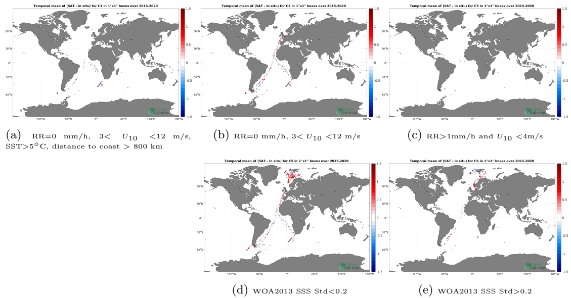
Figure 12: Temporal mean gridded over spatial boxes of size 1^\circ \times 1^\circ of \Delta SSS (SMAP SSS L2 v5 - 40 km (RSS) - TSG (Polarstern)) for 5 different subdatasets corresponding to:RR=0 mm/h, 3 < U_{10} < 12 m/s, SST >5^\circ C, distance to coast > 800 km (a), RR=0 mm/h, 3 < U_{10} < 12 m/s (b), RR >1 mm/h and U_{10} < 4 m/s (c), WOA2013 SSS Std <0.2 (d), WOA2013 SSS Std >0.2 (e).
