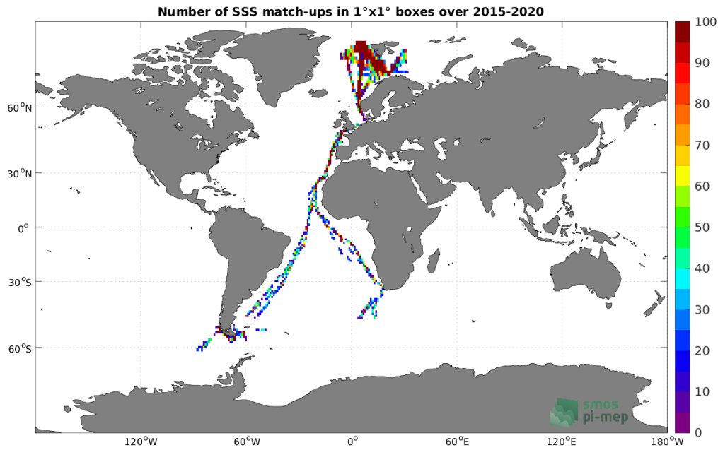
Figure 4: Number of SSS match-ups between TSG (Polarstern) SSS and the SMAP SSS L2 v5 - 40 km (RSS) SSS product for the Global Ocean Pi-MEP region over 1^\circ \times 1^\circ boxes and for the full satellite product period.
