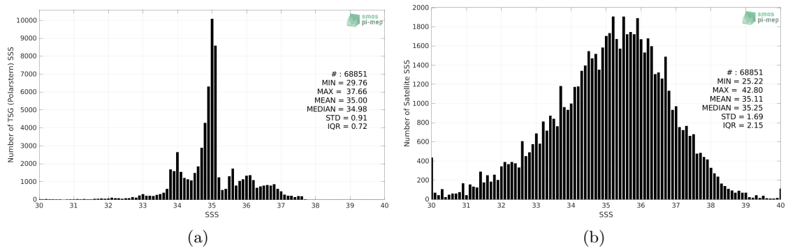
Figure 2: Histograms of SSS from TSG (Polarstern) (a) and SMAP SSS L2 v5 - 40 km (RSS) (b) considering all match-up pairs per bins of 0.1 over the Global Ocean Pi-MEP region and for the full satellite product period.
