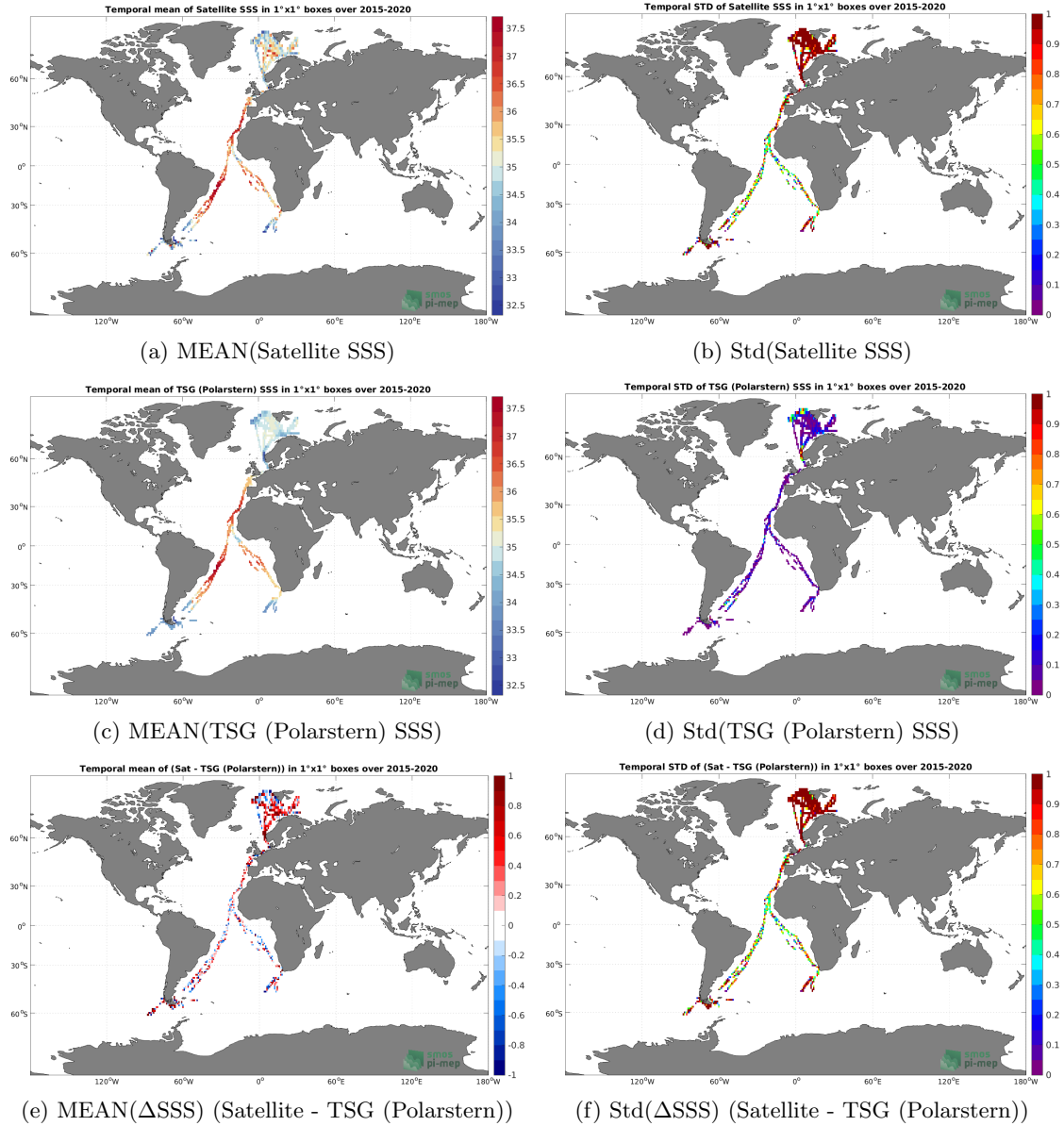
Figure 6: Temporal mean (left) and Std (right) of SSS from SMAP SSS L2 v5 - 40 km (RSS) (top), TSG (Polarstern) (middle), and of \Delta SSS (Satellite - TSG (Polarstern)). Only match-up pairs are used to generate these maps.
