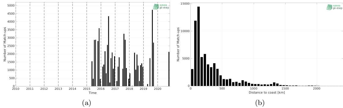
Figure 1: Number of match-ups between TSG (Polarstern) and SMAP SSS L2 v5 - 40 km (RSS) SSS as a function of time (a) and as function of the distance to coast (b) over the Global Ocean Pi-MEP region and for the full satellite product period.
