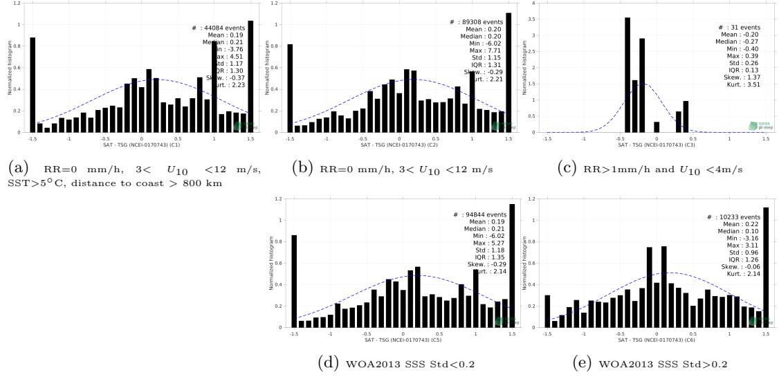
Figure 13: Normalized histogram of \Delta SSS (SMAP SSS L2 v5 - 40 km (RSS) - TSG (NCEI-0170743)) for 5 different subdatasets corresponding to: RR=0 mm/h, 3 < U_{10} < 12 m/s, SST > 5°C, distance to coast > 800 km (a), RR=0 mm/h, 3 < U_{10} < 12 m/s (b), RR > 1mm/h and U_{10} < 4 m/s (c), WOA2013 SSS Std < 0.2 (d), WOA2013 SSS Std > 0.2 (e).
