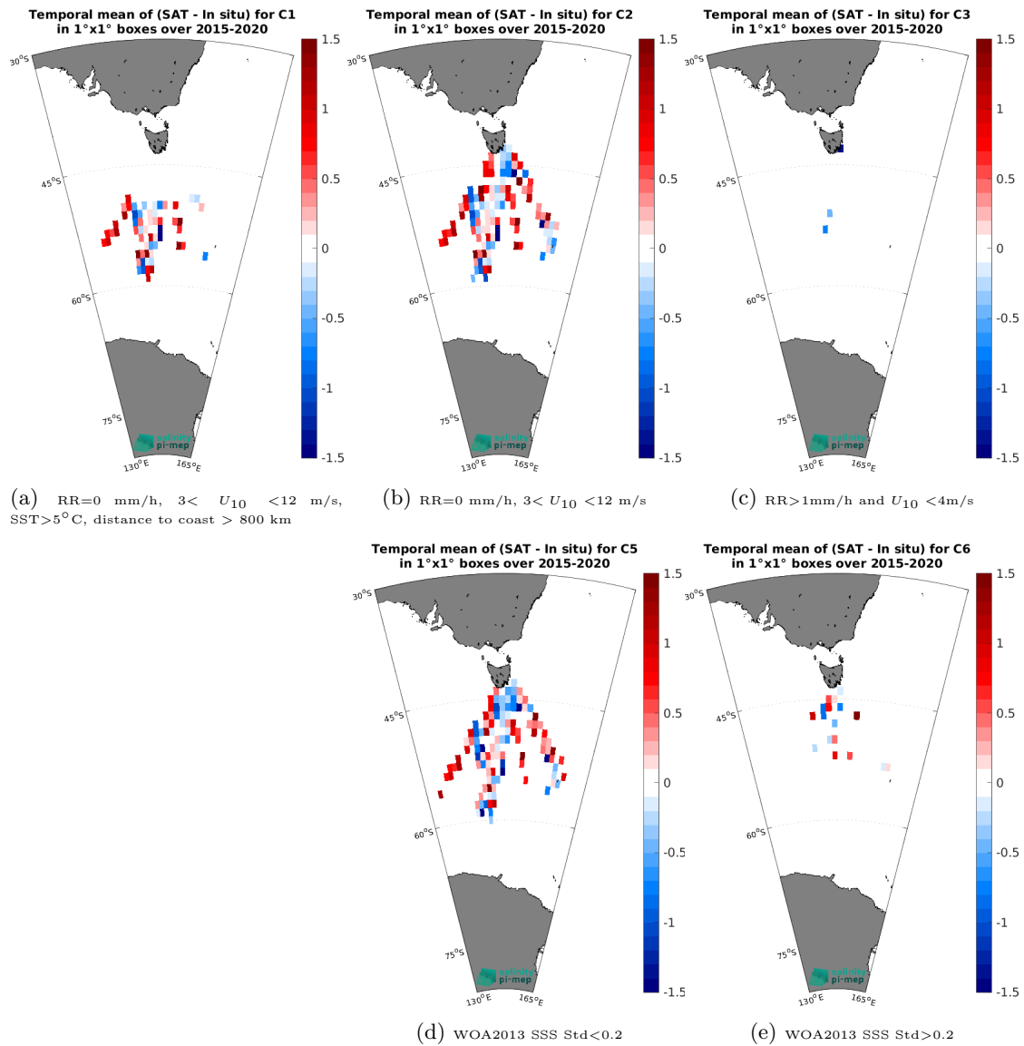
Figure 12: Temporal mean gridded over spatial boxes of size 1^\circ \times 1^\circ of \Delta\text{SSS} (SMAP SSS L2 v5 - 40 km (RSS) - TSG (LEGOS-Survostral)) for 5 different subdatasets corresponding to: RR=0 mm/h, 3 < U_{10} < 12 m/s, SST > 5^\circ\text{C} , distance to coast > 800 km (a), RR=0 mm/h, 3 < U_{10} < 12 m/s (b), RR > 1\text{mm/h} and U_{10} < 4\text{m/s} (c), WOA2013 SSS Std < 0.2 (d), WOA2013 SSS Std > 0.2 (e).
