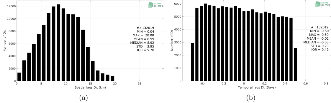
Figure 5: Histograms of the spatial (a) and temporal (b) lags between the location/time of the TSG (LEGOS-Survostral) measurement and the date of the corresponding SMAP SSS L2 v5 - 40 km (RSS) SSS pixel.
