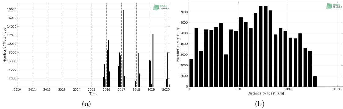
Figure 1: Number of match-ups between TSG (LEGOS-Survostral) and SMAP SSS L2 v5 - 40 km (RSS) SSS as a function of time (a) and as function of the distance to coast (b) over the Global Ocean Pi-MEP region and for the full satellite product period.
