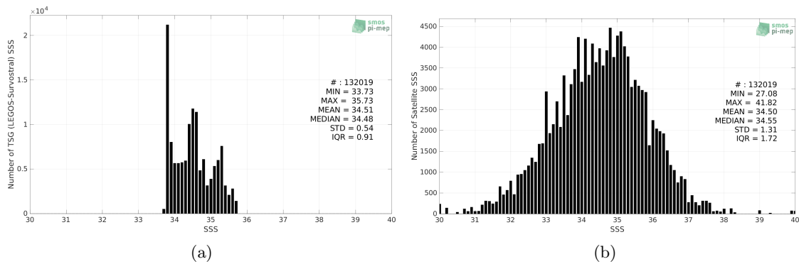
Figure 2: Histograms of SSS from TSG (LEGOS-Survostral) (a) and SMAP SSS L2 v5 - 40 km (RSS) (b) considering all match-up pairs per bins of 0.1 over the Global Ocean Pi-MEP region and for the full satellite product period.
