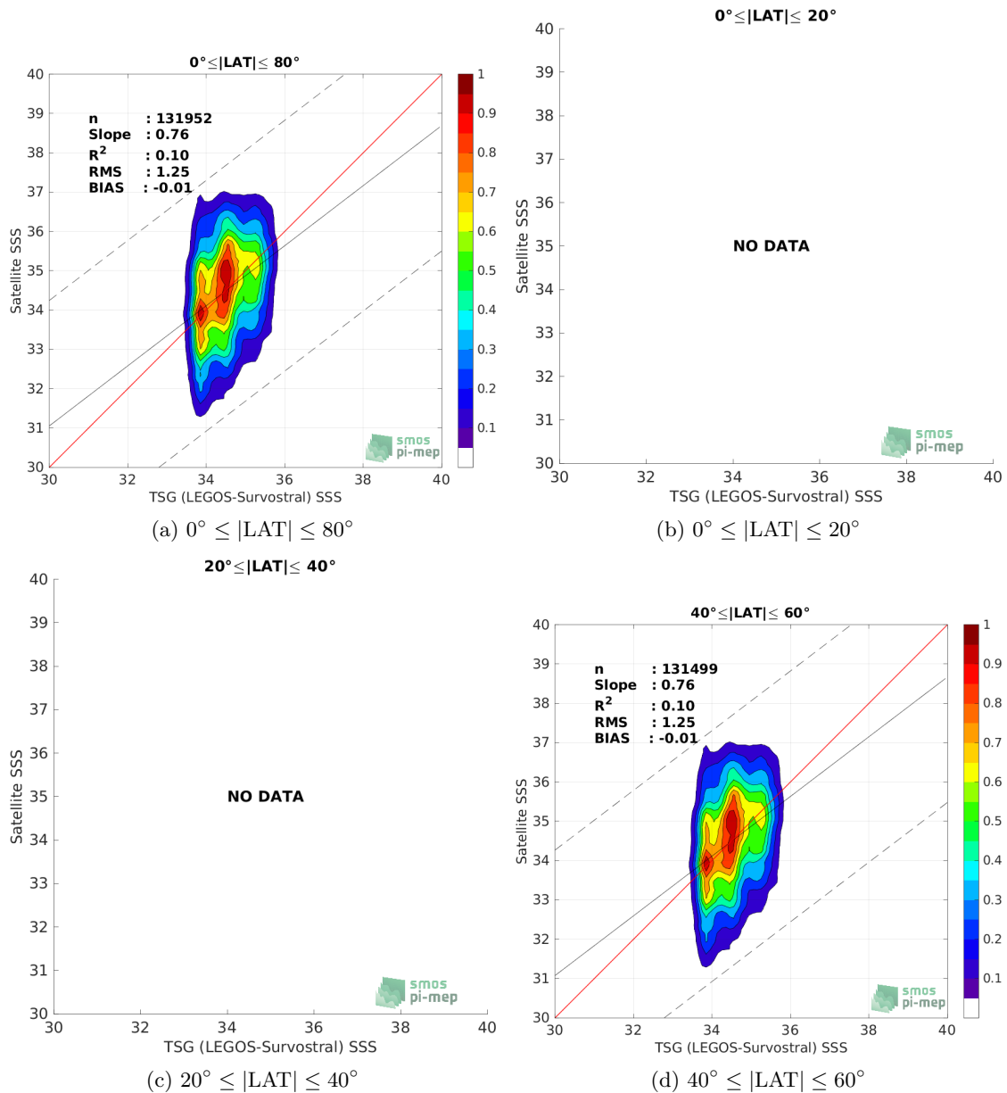
Figure 9: Contour maps of the concentration of SMAP SSS L2 v5 - 40 km (RSS) SSS (y-axis) versus TSG (LEGOS-Survostral) SSS (x-axis) at match-up pairs for different latitude bands. For each plot, the red line shows x=y . The black thin and dashed lines indicate a linear fit through the data cloud and the \pm 95\% confidence levels, respectively. The number match-up pairs n , the slope and R^2 coefficient of the linear fit, the root mean square (RMS) and the mean bias between satellite and in situ data are indicated for each latitude band in each plots.
