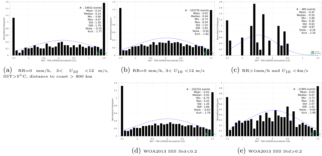
Figure 13: Normalized histogram of \Delta SSS (SMAP SSS L2 v5 - 40 km (RSS) - TSG (LEGOs-Survostral)) for 5 different subdatasets corresponding to: RR=0 mm/h, 3 < U_{10} < 12 m/s, SST > 5°C, distance to coast > 800 km (a), RR=0 mm/h, 3 < U_{10} < 12 m/s (b), RR > 1mm/h and U_{10} < 4 m/s (c), WOA2013 SSS Std < 0.2 (d), WOA2013 SSS Std > 0.2 (e).
