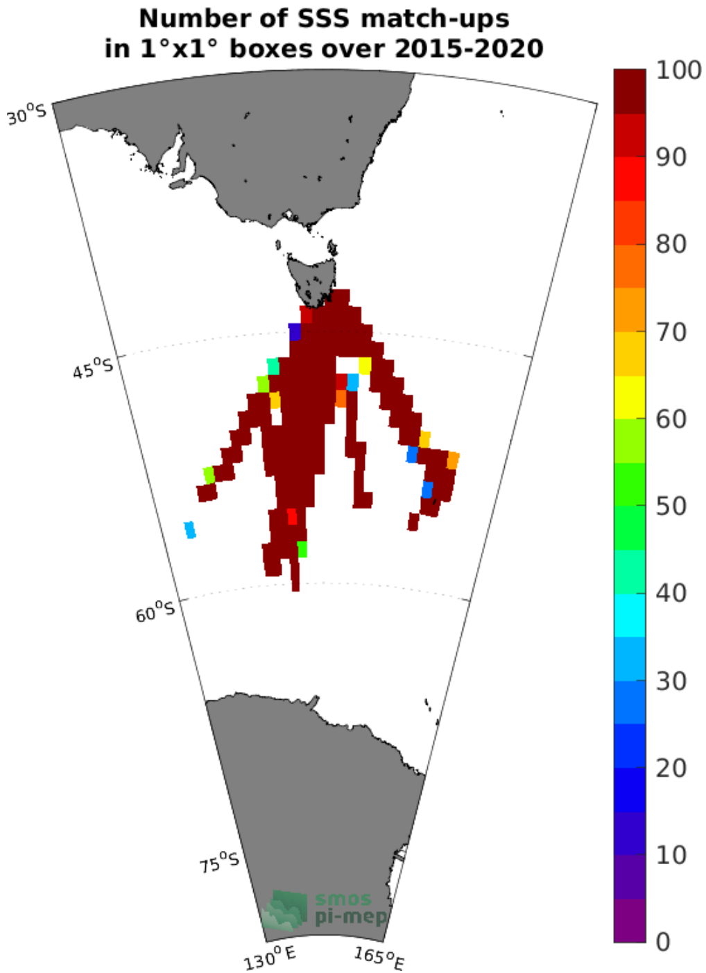
Figure 4: Number of SSS match-ups between TSG (LEGOS-Survostral) SSS and the SMAP SSS L2 v5 - 40 km (RSS) SSS product for the Global Ocean Pi-MEP region over 1°x1° boxes and for the full satellite product period.
