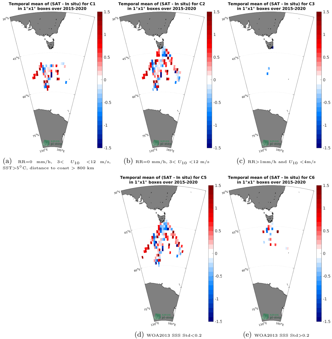
Figure 12: Temporal mean gridded over spatial boxes of size 1^\circ \times 1^\circ of \Delta SSS (SMAP SSS L2 v5 - 40 km (RSS) - TSG (LEGOS-Survostral)) for 5 different subdatasets corresponding to:RR=0 mm/h, 3 < U_{10} < 12 m/s, SST>5°C, distance to coast > 800 km (a), RR=0 mm/h, 3 < U_{10} < 12 m/s (b), RR>1mm/h and U_{10} < 4 m/s (c), WOA2013 SSS Std<0.2 (d), WOA2013 SSS Std>0.2 (e).
