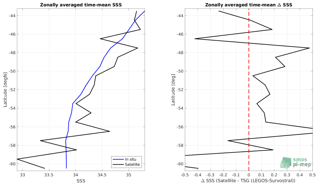
Figure 8: Left panel: Zonal mean SSS from SMAP SSS L2 v5 - 40 km (RSS) satellite product (black) and from TSG (LEGOS-Survostral) (blue). Right panel: Zonal mean of \Delta SSS (Satellite - TSG (LEGOS-Survostral)) for all the collected Pi-MEP match-up pairs estimated over the full satellite product period.
