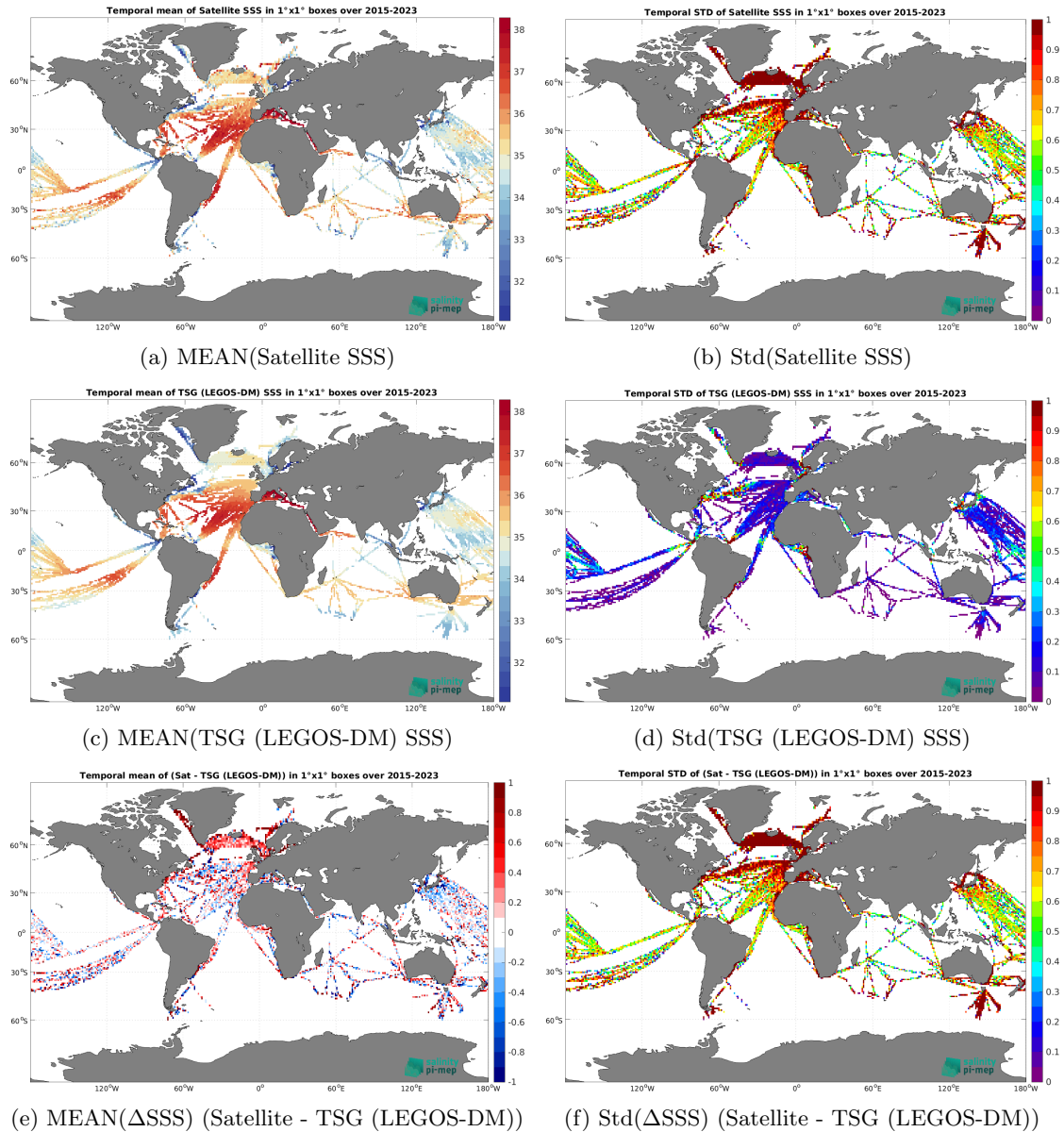
Figure 6: Temporal mean (left) and Std (right) of SSS from SMAP SSS L2 v5 - 40 km (RSS) (top), TSG (LEGOS-DM) (middle), and of \Delta SSS (Satellite - TSG (LEGOS-DM)). Only match-pair pairs are used to generate these maps.
