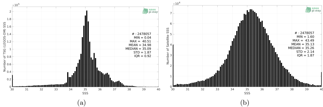
Figure 2: Histograms of SSS from TSG (LEGOS-DM) (a) and SMAP SSS L2 v5 - 40 km (RSS) (b) considering all match-up pairs per bins of 0.1 over the Global Ocean Pi-MEP region and for the full satellite product period.
