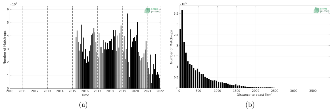
Figure 1: Number of match-ups between TSG (LEGOS-DM) and SMAP SSS L2 v5 - 40 km (RSS) SSS as a function of time (a) and as function of the distance to coast (b) over the Global Ocean Pi-MEP region and for the full satellite product period.
