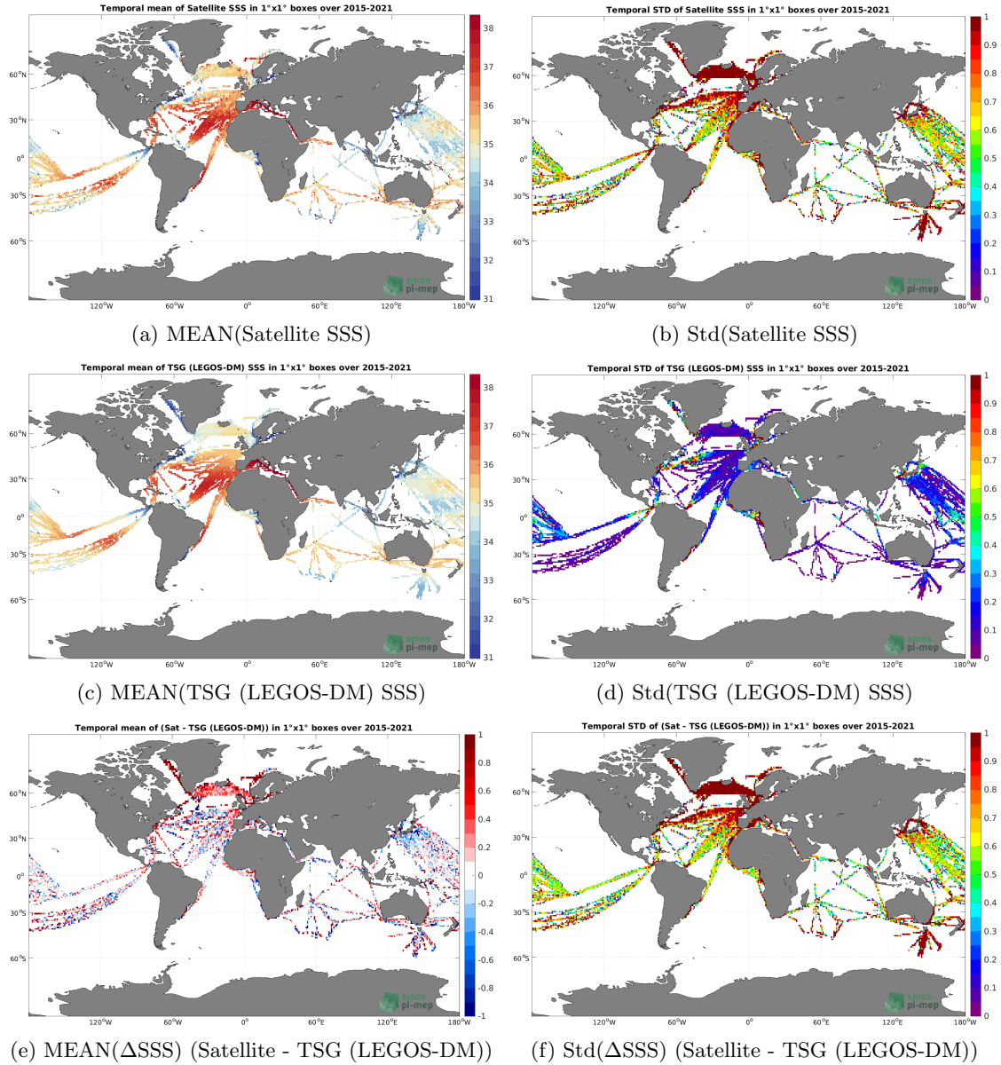
Figure 6: Temporal mean (left) and Std (right) of SSS from SMAP SSS L2 v5 - 40 km (RSS) (top), TSG (LEGOS-DM) (middle), and of \Delta SSS (Satellite - TSG (LEGOS-DM)). Only match-pairs are used to generate these maps.
