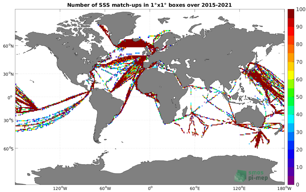
Figure 4: Number of SSS match-ups between TSG (LEGOS-DM) SSS and the SMAP SSS L2 v5 - 40 km (RSS) SSS product for the Global Ocean Pi-MEP region over 1^\circ \times 1^\circ boxes and for the full satellite product period.
