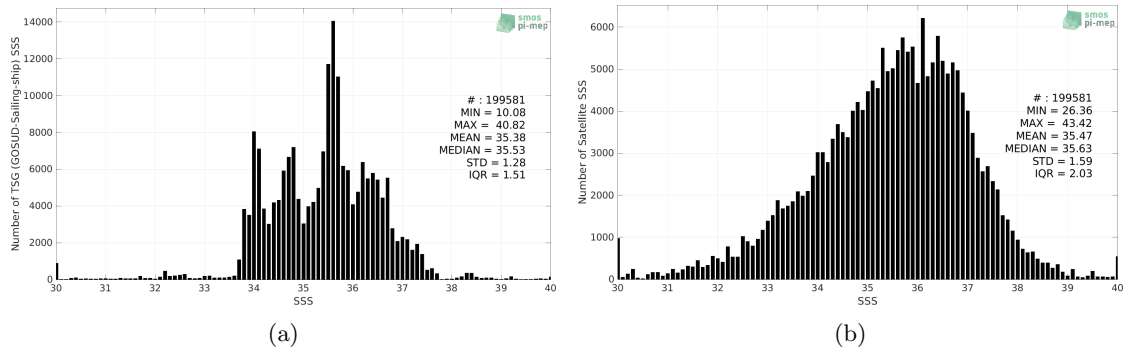
Figure 2: Histograms of SSS from TSG (GOSUD-Sailing-ship) (a) and SMAP SSS L2 v5 - 40 km (RSS) (b) considering all match-up pairs per bins of 0.1 over the Global Ocean Pi-MEP region and for the full satellite product period.
