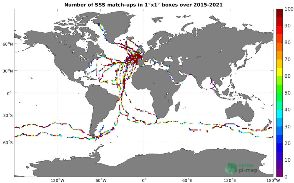
Figure 4: Number of SSS match-ups between TSG (GOSUD-Sailing-ship) SSS and the SMAP SSS L2 v5 - 40 km (RSS) SSS product for the Global Ocean Pi-MEP region over 1^\circ \times 1^\circ boxes and for the full satellite product period.
