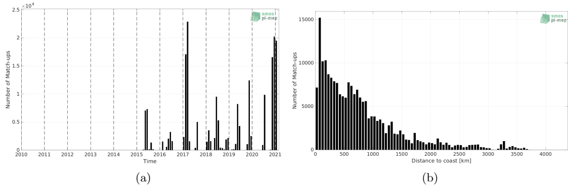
Figure 1: Number of match-ups between TSG (GOSUD-Sailing-ship) and SMAP SSS L2 v5 - 40 km (RSS) SSS as a function of time (a) and as function of the distance to coast (b) over the Global Ocean Pi-MEP region and for the full satellite product period.
