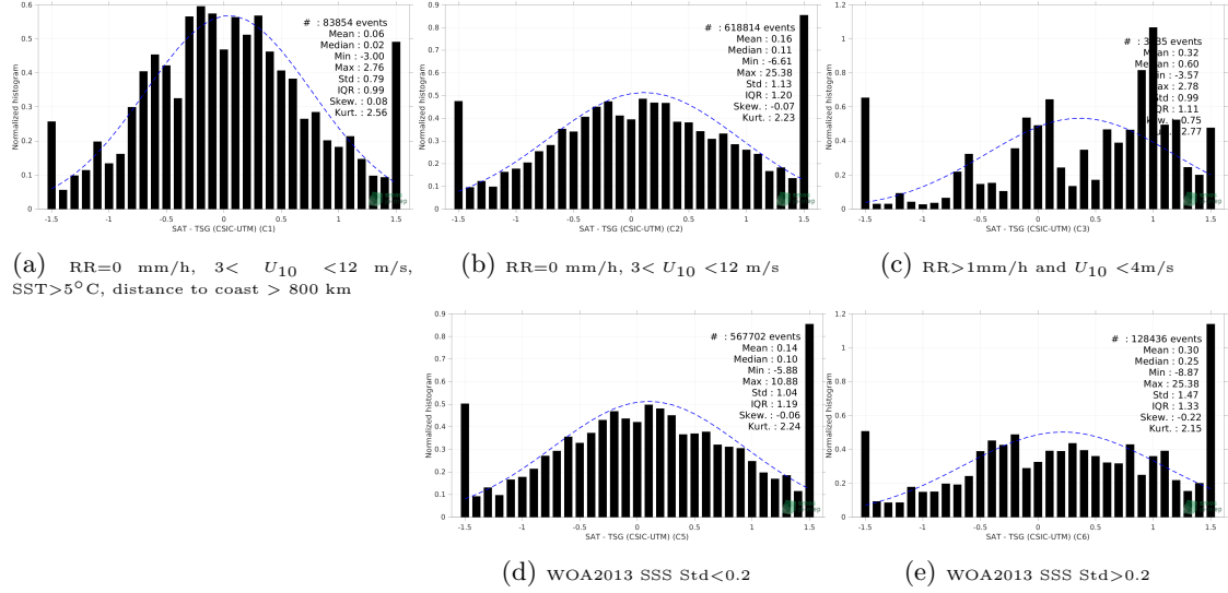
Figure 13: Normalized histogram of \Delta SSS (SMAP SSS L2 v5 - 40 km (RSS) - TSG (CSIC-UTM)) for 5 different subdatasets corresponding to: RR=0 mm/h, 3 < U_{10} < 12 m/s, SST > 5°C, distance to coast > 800 km (a), RR=0 mm/h, 3 < U_{10} < 12 m/s (b), RR > 1mm/h and U_{10} < 4 m/s (c), WOA2013 SSS Std < 0.2 (d), WOA2013 SSS Std > 0.2 (e).
