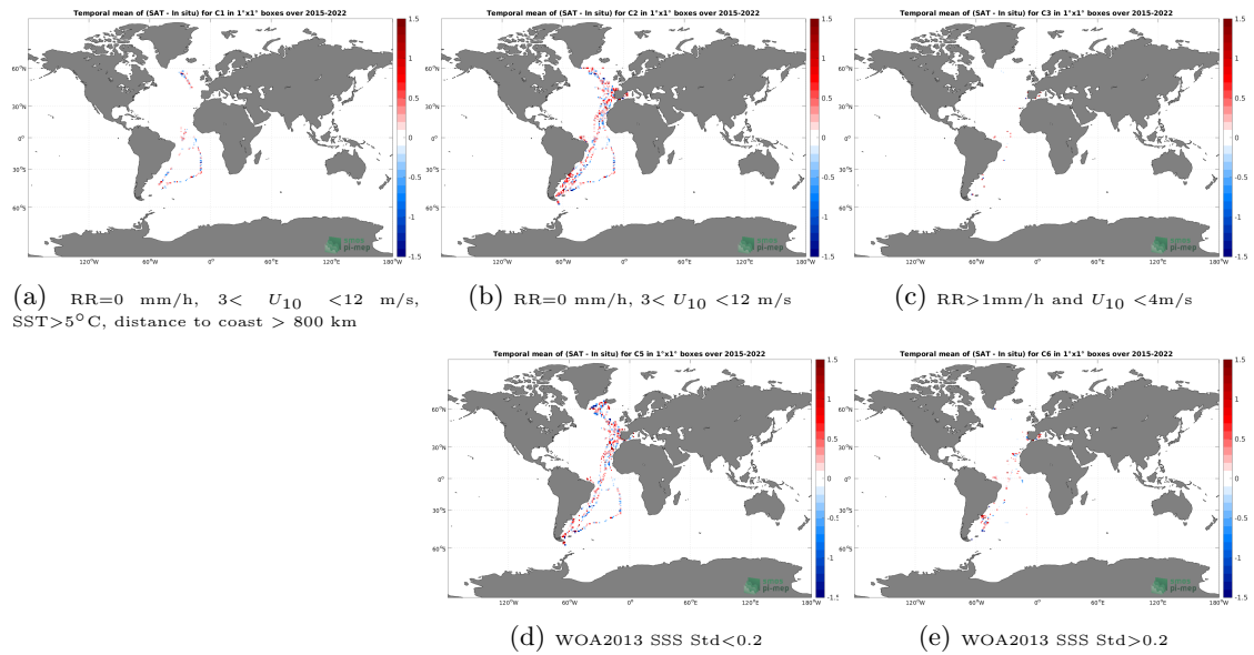
Figure 12: Temporal mean gridded over spatial boxes of size 1^\circ \times 1^\circ of \Delta SSS (SMAP SSS L2 v5 - 40 km (RSS) - TSG (CSIC-UTM)) for 5 different subdatasets corresponding to:RR=0 mm/h, 3 < U_{10} < 12 m/s, SST >5^\circ C, distance to coast > 800 km (a), RR=0 mm/h, 3 < U_{10} < 12 m/s (b), RR >1 mm/h and U_{10} < 4 m/s (c), WOA2013 SSS Std <0.2 (d), WOA2013 SSS Std >0.2 (e).
