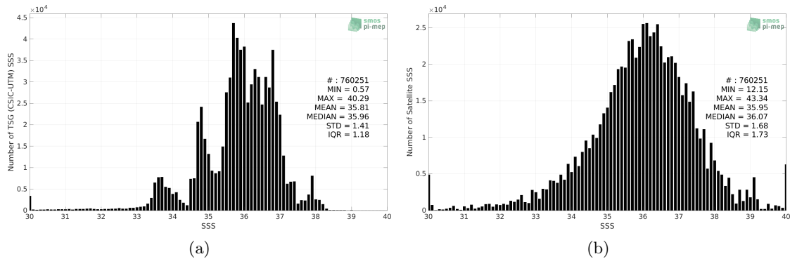
Figure 2: Histograms of SSS from TSG (CSIC-UTM) (a) and SMAP SSS L2 v5 - 40 km (RSS) (b) considering all match-up pairs per bins of 0.1 over the Global Ocean Pi-MEP region and for the full satellite product period.
