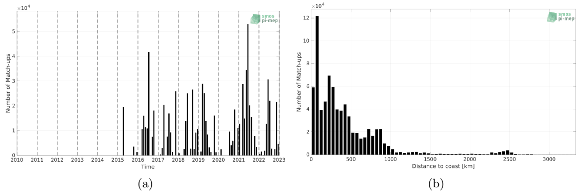
Figure 1: Number of match-ups between TSG (CSIC-UTM) and SMAP SSS L2 v5 - 40 km (RSS) SSS as a function of time (a) and as function of the distance to coast (b) over the Global Ocean Pi-MEP region and for the full satellite product period.
