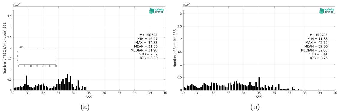
Figure 2: Histograms of SSS from TSG (Amundsen) (a) and SMAP SSS L2 v5 - 40 km (RSS) (b) considering all match-up pairs per bins of 0.1 over the Global Ocean Pi-MEP region and for the full satellite product period.
