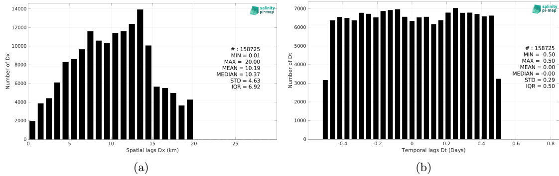
Figure 5: Histograms of the spatial (a) and temporal (b) lags between the location/time of the TSG (Amundsen) measurement and the date of the corresponding SMAP SSS L2 v5 - 40 km (RSS) SSS pixel.
