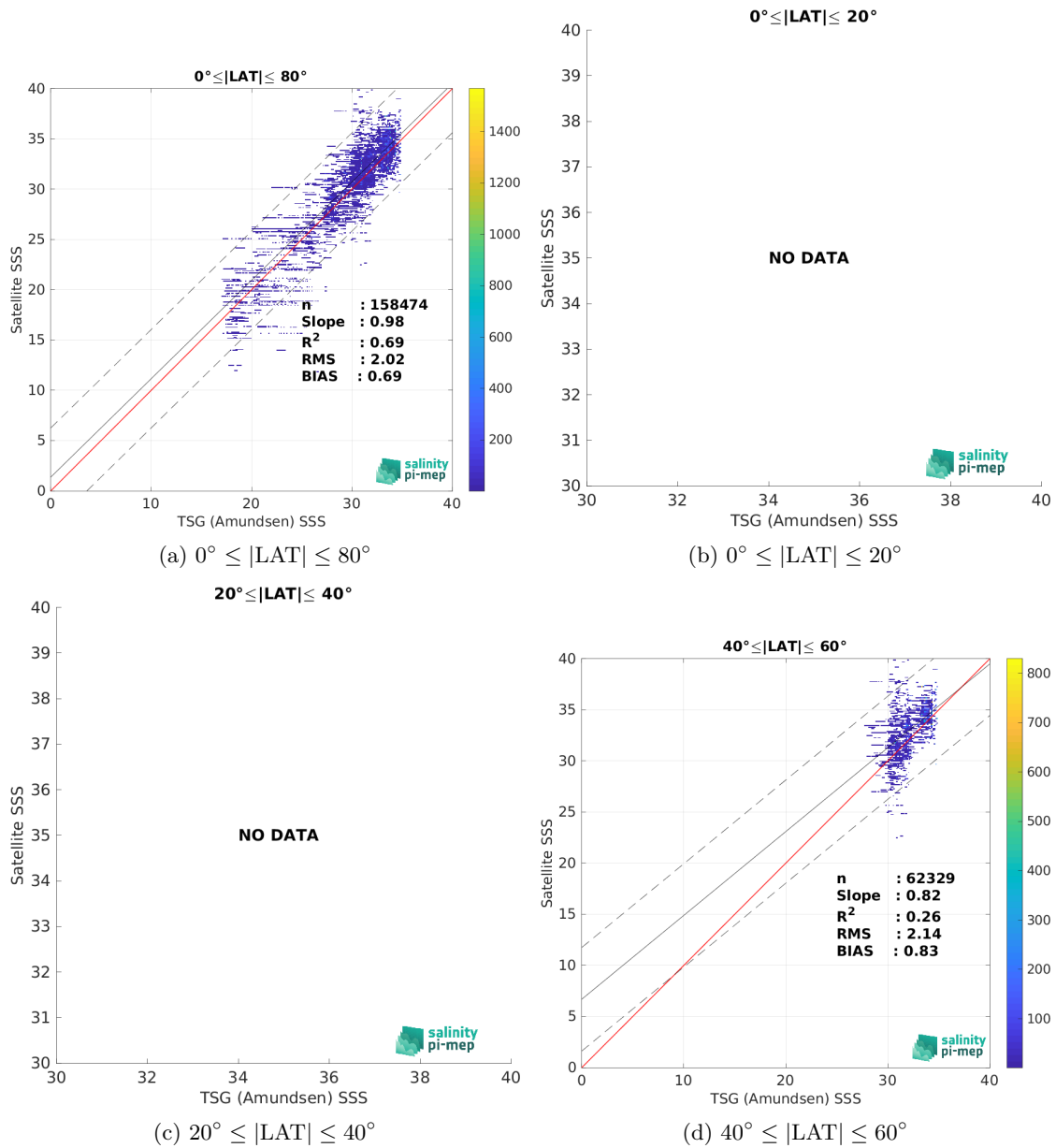
Figure 9: Contour maps of the concentration of SMAP SSS L2 v5 - 40 km (RSS) SSS (y-axis) versus TSG (Amundsen) SSS (x-axis) at match-up pairs for different latitude bands. For each plot, the red line shows x=y . The black thin and dashed lines indicate a linear fit through the data cloud and the \pm 95\% confidence levels, respectively. The number match-up pairs n , the slope and R^2 coefficient of the linear fit, the root mean square (RMS) and the mean bias between satellite and in situ data are indicated for each latitude band in each plots.
