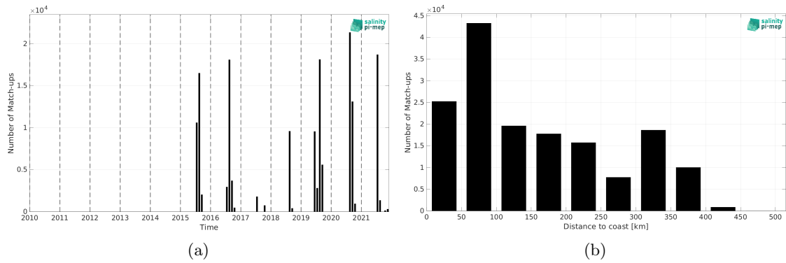
Figure 1: Number of match-ups between TSG (Amundsen) and SMAP SSS L2 v5 - 40 km (RSS) SSS as a function of time (a) and as function of the distance to coast (b) over the Global Ocean Pi-MEP region and for the full satellite product period.
