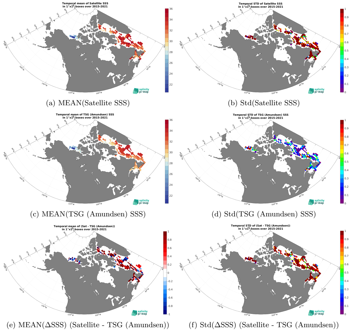
Figure 6: Temporal mean (left) and Std (right) of SSS from SMAP SSS L2 v5 - 40 km (RSS) (top), TSG (Amundsen) (middle), and of \Delta SSS (Satellite - TSG (Amundsen)). Only match-up pairs are used to generate these maps.
