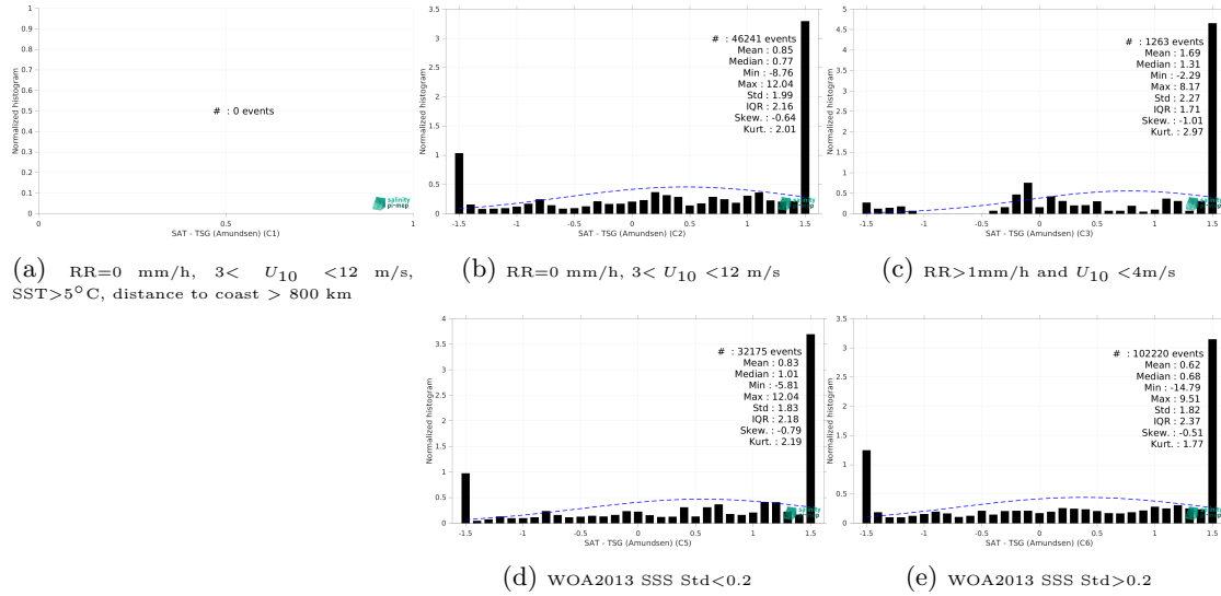
Figure 13: Normalized histogram of \Delta SSS (SMAP SSS L2 v5 - 40 km (RSS) - TSG (Amundsen)) for 5 different subdatasets corresponding to: RR=0 mm/h, 3 < U_{10} < 12 m/s, SST > 5°C, distance to coast > 800 km (a), RR=0 mm/h, 3 < U_{10} < 12 m/s (b), RR > 1mm/h and U_{10} < 4 m/s (c), WOA2013 SSS Std < 0.2 (d), WOA2013 SSS Std > 0.2 (e).
