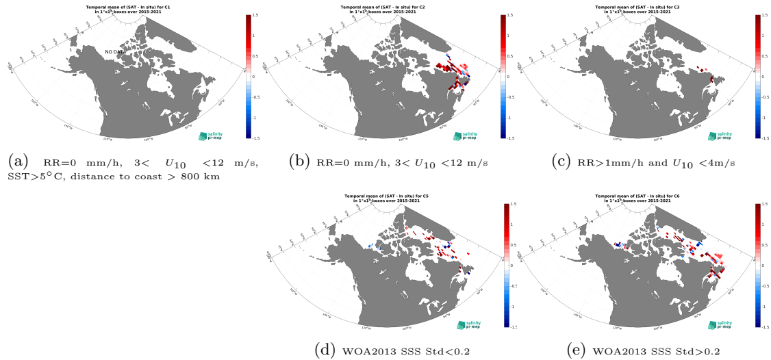
Figure 12: Temporal mean gridded over spatial boxes of size 1^{\circ}\times 1^{\circ} of \Delta\text{SSS} (SMAP SSS L2 v5 - 40 km (RSS) - TSG (Amundsen)) for 5 different subdatasets corresponding to:RR=0 mm/h, 3 < U_{10} < 12 m/s, SST > 5^{\circ}\text{C} , distance to coast > 800 km (a), RR=0 mm/h, 3 < U_{10} < 12 m/s (b), RR > 1 mm/h and U_{10} < 4 m/s (c), WOA2013 SSS Std < 0.2 (d), WOA2013 SSS Std > 0.2 (e).
