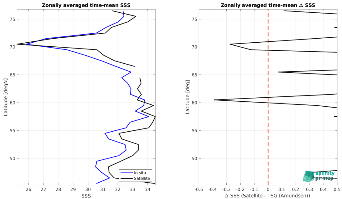
Figure 8: Left panel: Zonal mean SSS from SMAP SSS L2 v5 - 40 km (RSS) satellite product (black) and from TSG (Amundsen) (blue). Right panel: Zonal mean of \Delta SSS (Satellite - TSG (Amundsen)) for all the collected Pi-MEP match-up pairs estimated over the full satellite product period.
