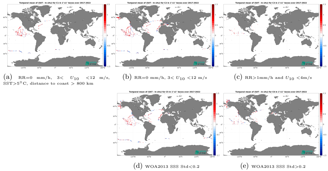
Figure 12: Temporal mean gridded over spatial boxes of size 1^\circ \times 1^\circ of \Delta SSS (SMAP SSS L2 v5 - 40 km (RSS) - Saildrone) for 5 different subdatasets corresponding to:RR=0 mm/h, 3 < U_{10} < 12 m/s, SST > 5^\circ\text{C} , distance to coast > 800 km (a), RR=0 mm/h, 3 < U_{10} < 12 m/s (b), RR > 1 mm/h and U_{10} < 4 m/s (c), WOA2013 SSS Std < 0.2 (d), WOA2013 SSS Std > 0.2 (e).
