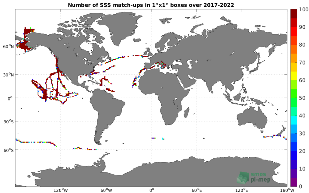
Figure 4: Number of SSS match-ups between Saildrone SSS and the SMAP SSS L2 v5 - 40 km (RSS) SSS product for the Global Ocean Pi-MEP region over 1^\circ \times 1^\circ boxes and for the full satellite product period.
