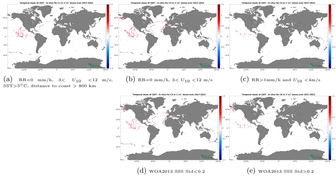
Figure 12: Temporal mean gridded over spatial boxes of size 1^\circ \times 1^\circ of \Delta SSS (SMAP SSS L2 v5 - 40 km (RSS) - Sairdrone) for 5 different subdatasets corresponding to:RR=0 mm/h, 3 < U_{10} < 12 m/s, SST >5^\circ\text{C} , distance to coast > 800 km (a), RR=0 mm/h, 3 < U_{10} < 12 m/s (b), RR >1 mm/h and U_{10} < 4 m/s (c), WOA2013 SSS Std <0.2 (d), WOA2013 SSS Std >0.2 (e).
