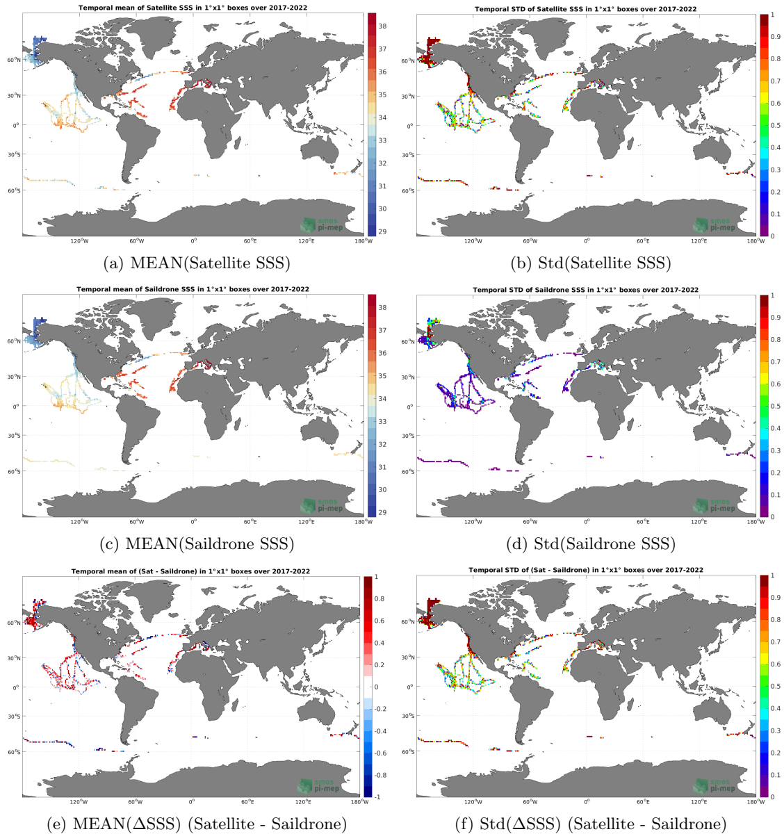
Figure 6: Temporal mean (left) and Std (right) of SSS from SMAP SSS L2 v5 - 40 km (RSS) (top), Saildrone (middle), and of \Delta SSS (Satellite - Saildrone). Only match-up pairs are used to generate these maps.
