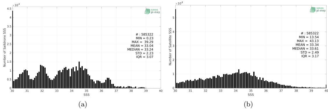
Figure 2: Histograms of SSS from Saildrone (a) and SMAP SSS L2 v5 - 40 km (RSS) (b) considering all match-up pairs per bins of 0.1 over the Global Ocean Pi-MEP region and for the full satellite product period.
