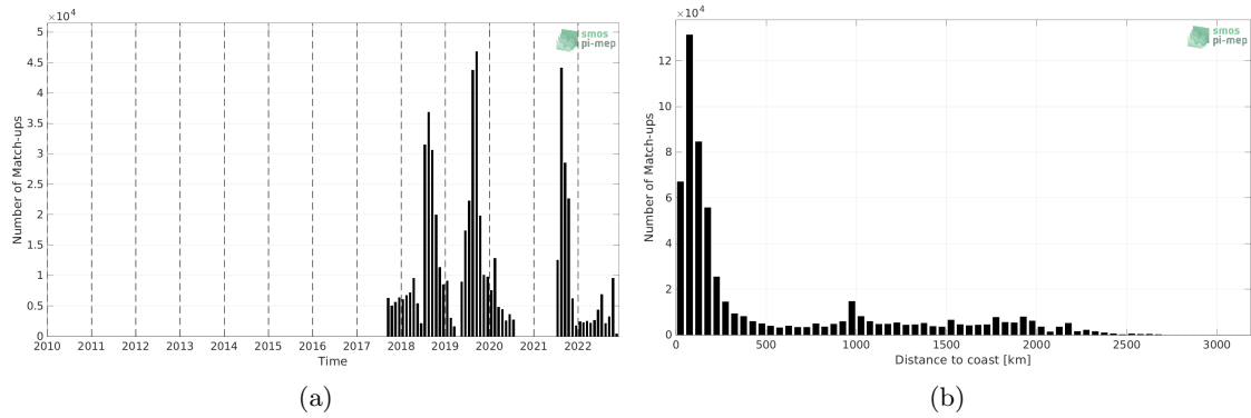
Figure 1: Number of match-ups between Saildrone and SMAP SSS L2 v5 - 40 km (RSS) SSS as a function of time (a) and as function of the distance to coast (b) over the Global Ocean Pi-MEP region and for the full satellite product period.
