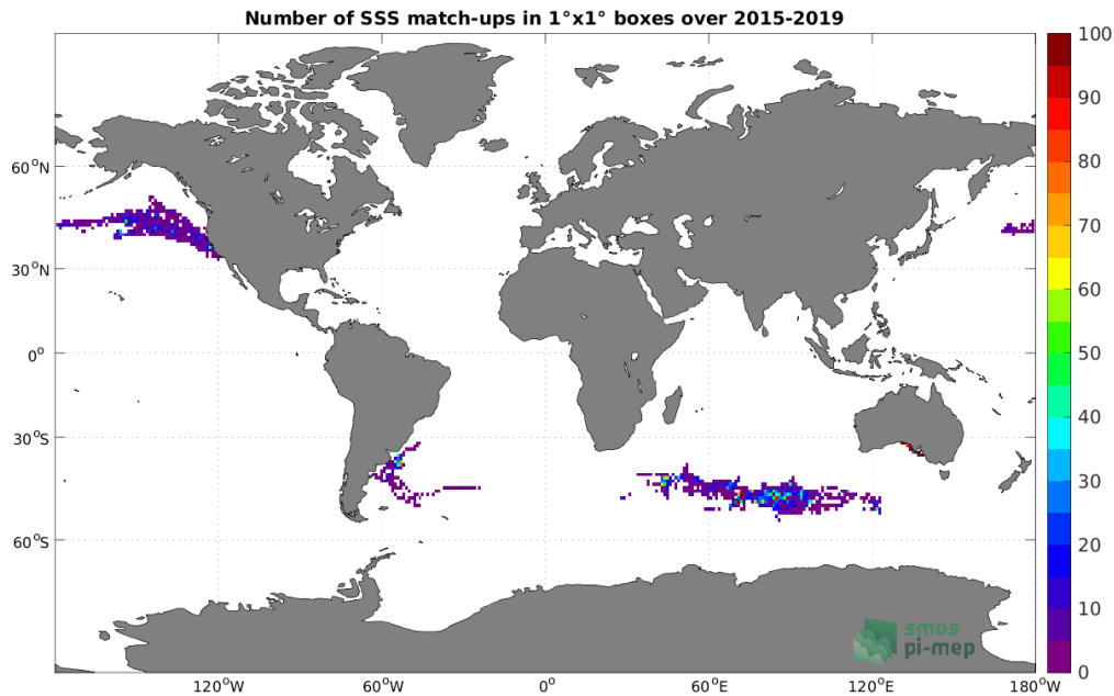
Figure 4: Number of SSS match-ups between Marine mammals SSS and the SMAP SSS L2 v5 - 40 km (RSS) SSS product for the Global Ocean Pi-MEP region over 1^\circ \times 1^\circ boxes and for the full satellite product period.
