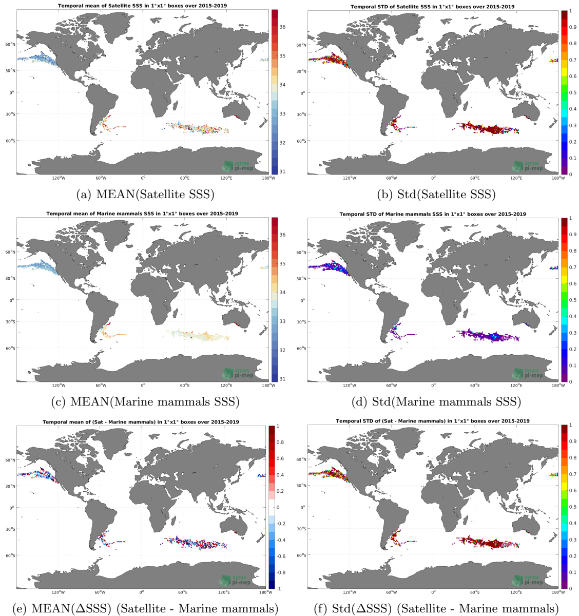
Figure 6: Temporal mean (left) and Std (right) of SSS from SMAP SSS L2 v5 - 40 km (RSS) (top), Marine mammals (middle), and of \Delta SSS (Satellite - Marine mammals). Only match-up pairs are used to generate these maps.
