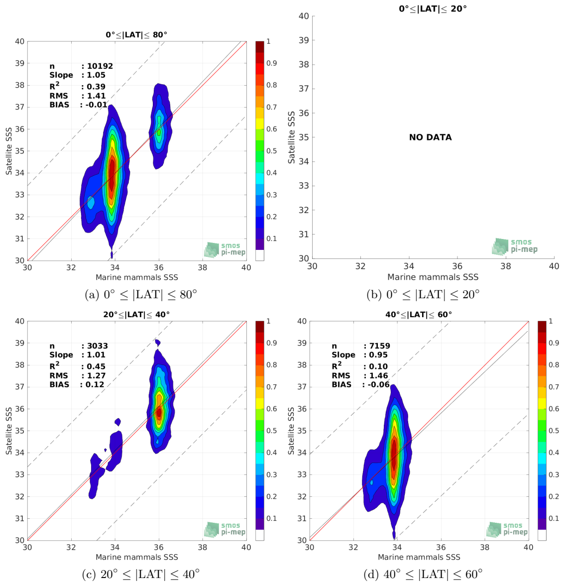
Figure 9: Contour maps of the concentration of SMAP SSS L2 v5 - 40 km (RSS) SSS (y-axis) versus Marine mammals SSS (x-axis) at match-up pairs for different latitude bands. For each plot, the red line shows x=y . The black thin and dashed lines indicate a linear fit through the data cloud and the \pm 95\% confidence levels, respectively. The number match-up pairs n , the slope and R^2 coefficient of the linear fit, the root mean square (RMS) and the mean bias between satellite and in situ data are indicated for each latitude band in each plots.
