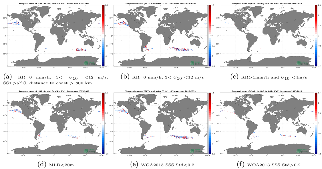
Figure 12: Temporal mean gridded over spatial boxes of size 1^\circ \times 1^\circ of \Delta SSS (SMAP SSS L2 v5 - 40 km (RSS) - Marine mammals) for 6 different subdatasets corresponding to:RR=0 mm/h, 3 < U_{10} < 12 m/s, SST >5^\circ C, distance to coast > 800 km (a), RR=0 mm/h, 3 < U_{10} < 12 m/s (b), RR >1 mm/h and U_{10} < 4 m/s (c),MLD <20 m (d),WOA2013 SSS Std <0.2 (e),WOA2013 SSS Std >0.2 (f).
