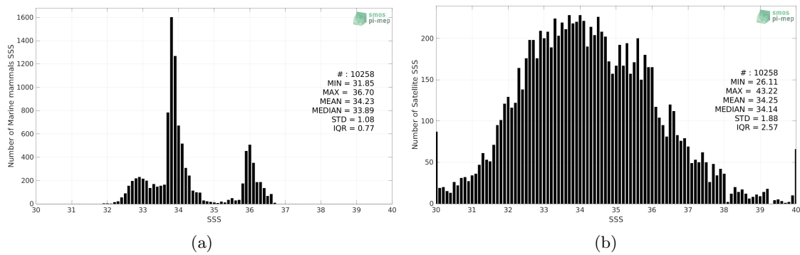
Figure 2: Histograms of SSS from Marine mammals (a) and SMAP SSS L2 v5 - 40 km (RSS) (b) considering all match-up pairs per bins of 0.1 over the Global Ocean Pi-MEP region and for the full satellite product period.
