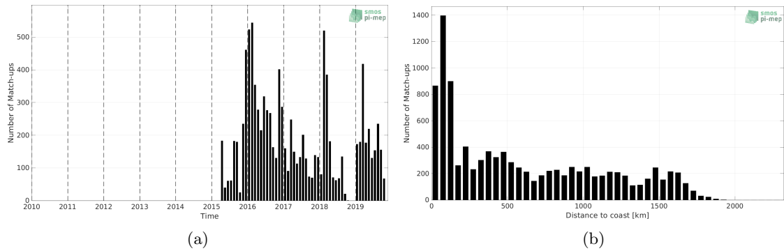
Figure 1: Number of match-ups between Marine mammals and SMAP SSS L2 v5 - 40 km (RSS) SSS as a function of time (a) and as function of the distance to coast (b) over the Global Ocean Pi-MEP region and for the full satellite product period.
