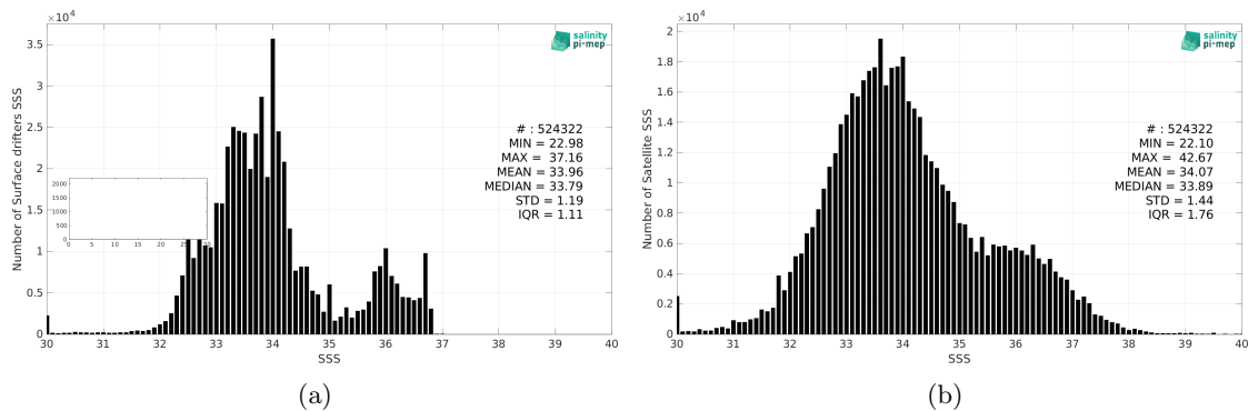
Figure 2: Histograms of SSS from Surface drifters (a) and SMAP SSS L2 v5 - 40 km (RSS) (b) considering all match-up pairs per bins of 0.1 over the Global Ocean Pi-MEP region and for the full satellite product period.
