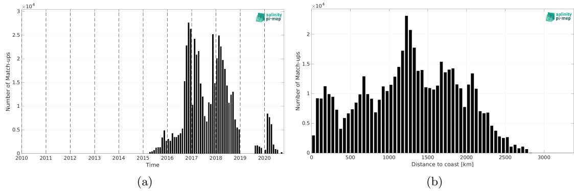
Figure 1: Number of match-ups between Surface drifters and SMAP SSS L2 v5 - 40 km (RSS) SSS as a function of time (a) and as function of the distance to coast (b) over the Global Ocean Pi-MEP region and for the full satellite product period.
