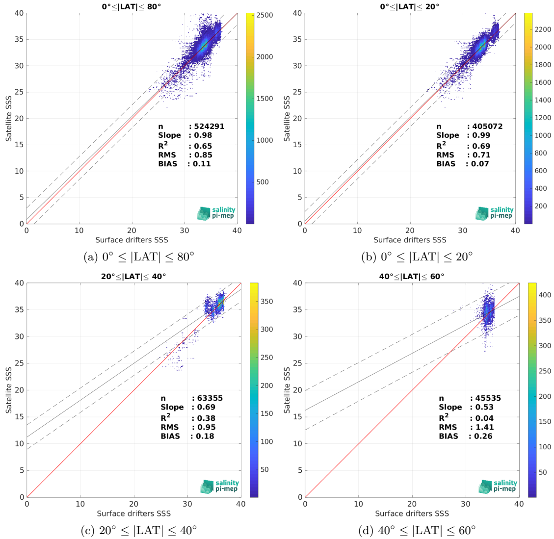
Figure 8: Contour maps of the concentration of SMAP SSS L2 v5 - 40 km (RSS) SSS (y-axis) versus Surface drifters SSS (x-axis) at match-up pairs for different latitude bands. For each plot, the red line shows x=y . The black thin and dashed lines indicate a linear fit through the data cloud and the \pm 95\% confidence levels, respectively. The number match-up pairs n , the slope and R^2 coefficient of the linear fit, the root mean square (RMS) and the mean bias between satellite and in situ data are indicated for each latitude band in each plots.
