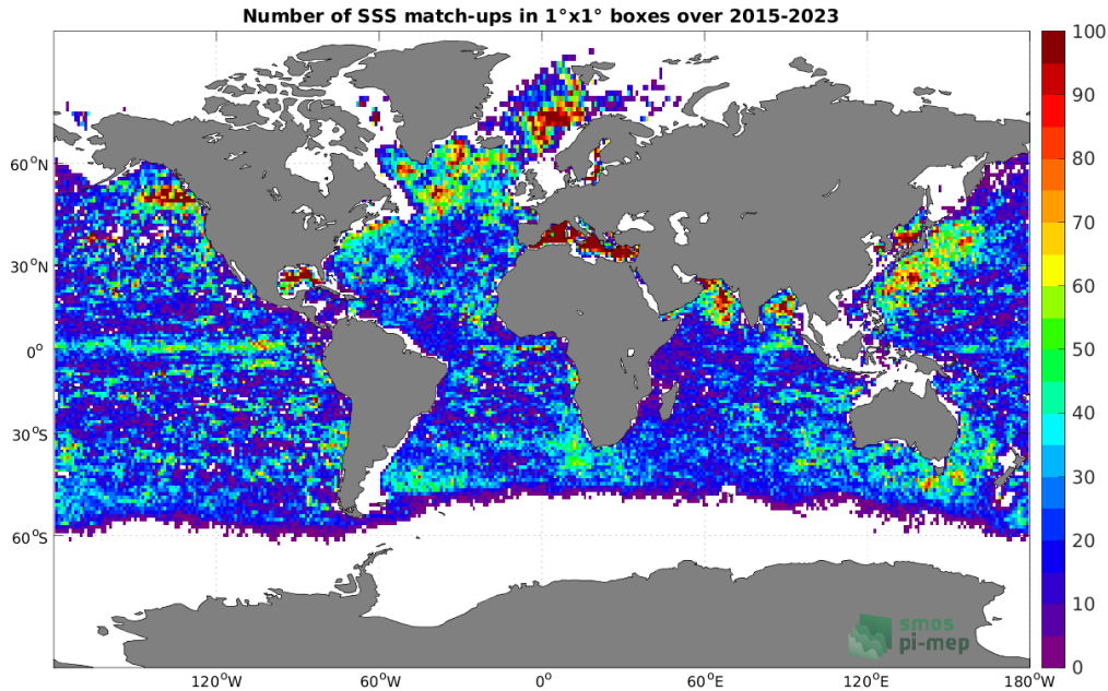
Figure 4: Number of SSS match-ups between Argo SSS and the SMAP SSS L2 v5 - 40 km (RSS) SSS product for the Global Ocean Pi-MEP region over 1^\circ \times 1^\circ boxes and for the full satellite product period.
