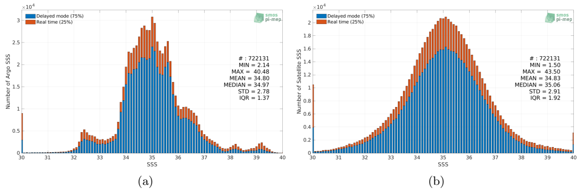
Figure 2: Histograms of SSS from Argo (a) and SMAP SSS L2 v5 - 40 km (RSS) (b) considering all match-up pairs per bins of 0.1 over the Global Ocean Pi-MEP region and for the full satellite product period.
