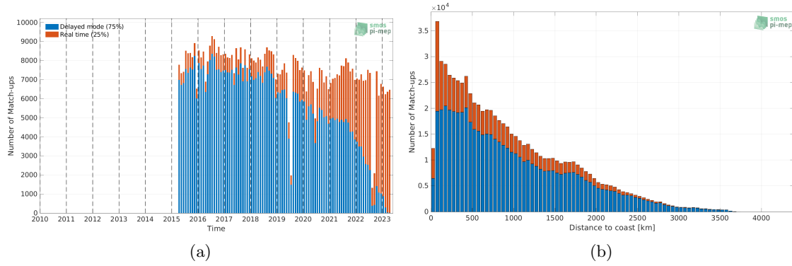
Figure 1: Number of match-ups between Argo and SMAP SSS L2 v5 - 40 km (RSS) SSS as a function of time (a) and as function of the distance to coast (b) over the Global Ocean Pi-MEP region and for the full satellite product period.
