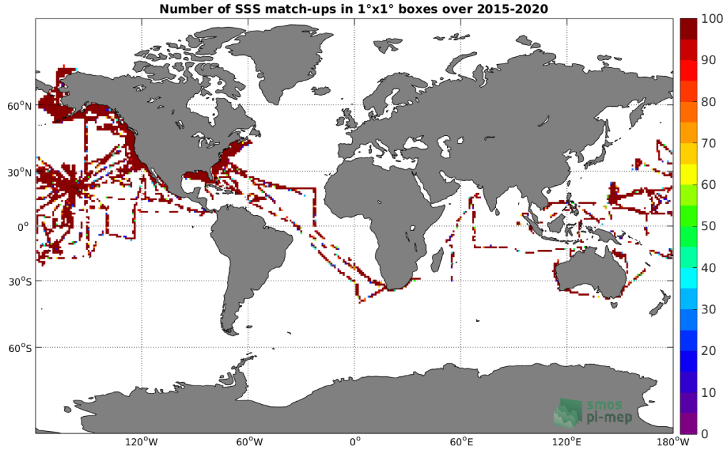
Figure 4: Number of SSS match-ups between TSG (SAMOS) SSS and the SMAP SSS L2 v4 (RSS) SSS product for the Global Ocean Pi-MEP region over 1^\circ \times 1^\circ boxes and for the full satellite product period.
