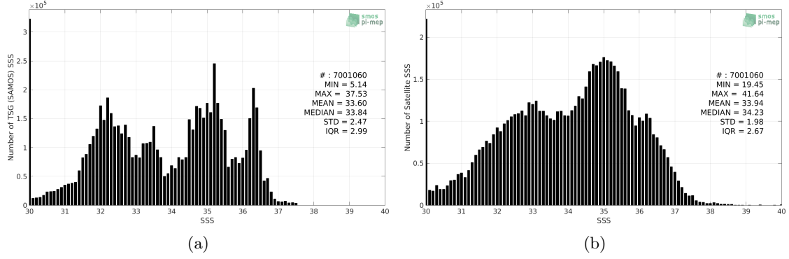
Figure 2: Histograms of SSS from TSG (SAMOS) (a) and SMAP SSS L2 v4 (RSS) (b) considering all match-up pairs per bins of 0.1 over the Global Ocean Pi-MEP region and for the full satellite product period.
