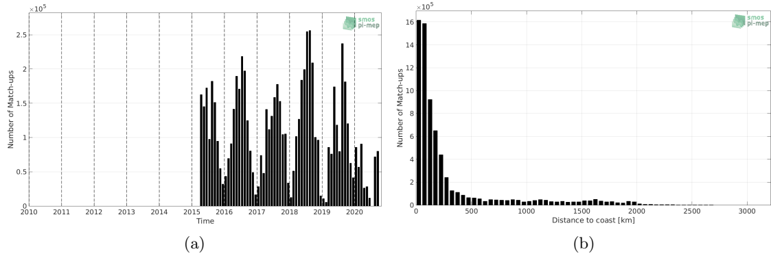
Figure 1: Number of match-ups between TSG (SAMOS) and SMAP SSS L2 v4 (RSS) SSS as a function of time (a) and as function of the distance to coast (b) over the Global Ocean Pi-MEP region and for the full satellite product period.
