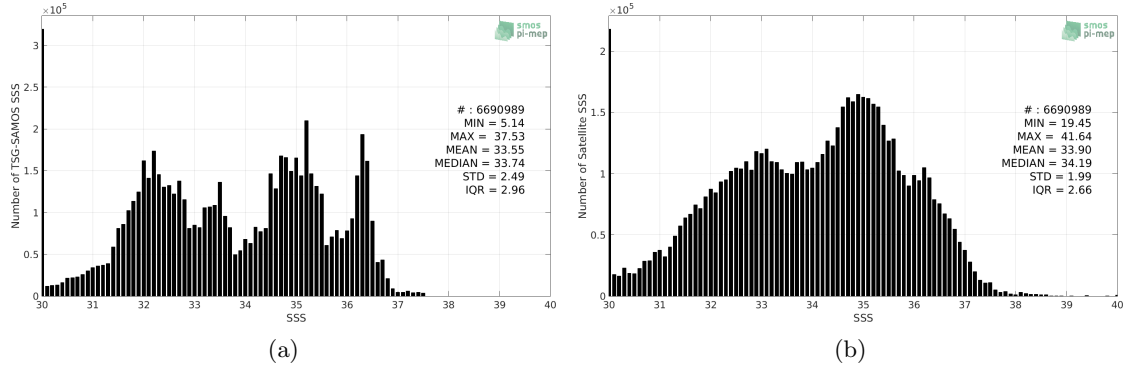
Figure 2: Histograms of SSS from TSG-SAMOS (a) and SMAP-L2-RSS-V4 (b) considering all match-up pairs per bins of 0.1 over the Global Ocean Pi-MEP region and for the full satellite product period.
