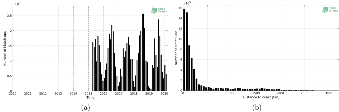
Figure 1: Number of match-ups between TSG-SAMOS and SMAP-L2-RSS-V4 SSS as a function of time (a) and as function of the distance to coast (b) over the Global Ocean Pi-MEP region and for the full satellite product period.
