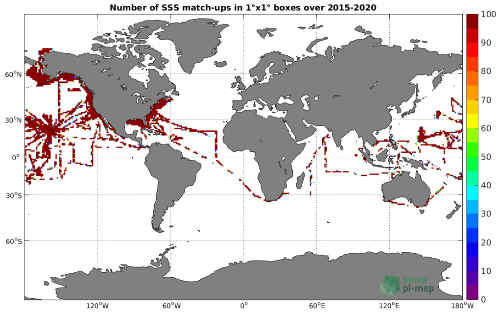
Figure 4: Number of SSS match-ups between TSG-SAMOS SSS and the SMAP-L2-RSS-V4 SSS product for the Global Ocean Pi-MEP region over 1^\circ \times 1^\circ boxes and for the full satellite product period.
