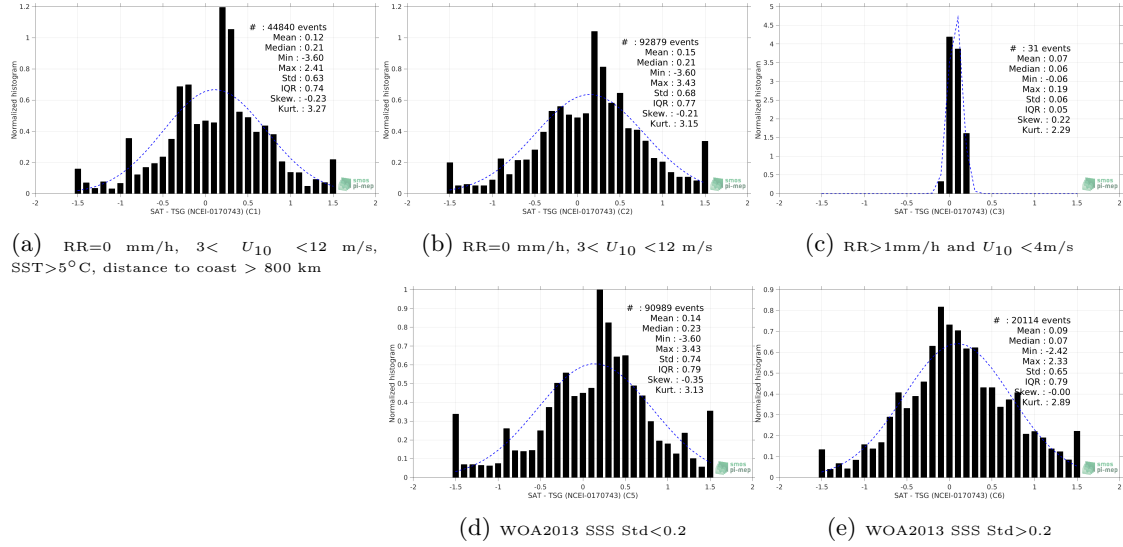
Figure 13: Normalized histogram of \Delta SSS (SMAP SSS L2 v4 (RSS) - TSG (NCEI-0170743)) for 5 different subdatasets corresponding to: RR=0 mm/h, 3 < U_{10} < 12 m/s, SST>5°C, distance to coast > 800 km (a), RR=0 mm/h, 3 < U_{10} < 12 m/s (b), RR>1mm/h and U_{10} < 4 m/s (c), WOA2013 SSS Std<0.2 (d), WOA2013 SSS Std>0.2 (e).
