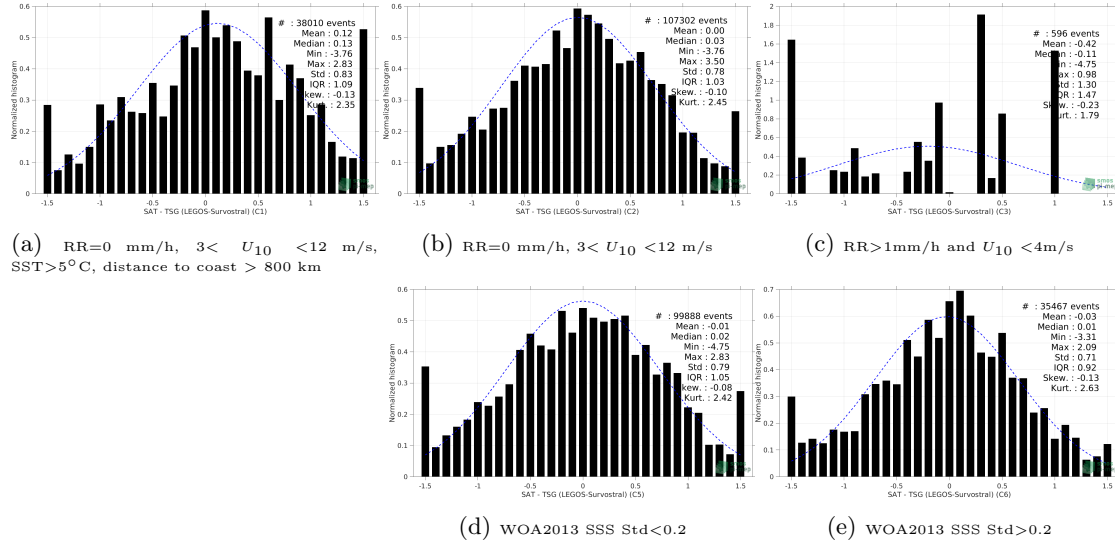
Figure 13: Normalized histogram of \Delta SSS (SMAP SSS L2 v4 (RSS) - TSG (LEGOS-Survostral)) for 5 different subdatasets corresponding to: RR=0 mm/h, 3 < U_{10} < 12 m/s, SST > 5°C, distance to coast > 800 km (a), RR=0 mm/h, 3 < U_{10} < 12 m/s (b), RR > 1mm/h and U_{10} < 4 m/s (c), WOA2013 SSS Std < 0.2 (d), WOA2013 SSS Std > 0.2 (e).
