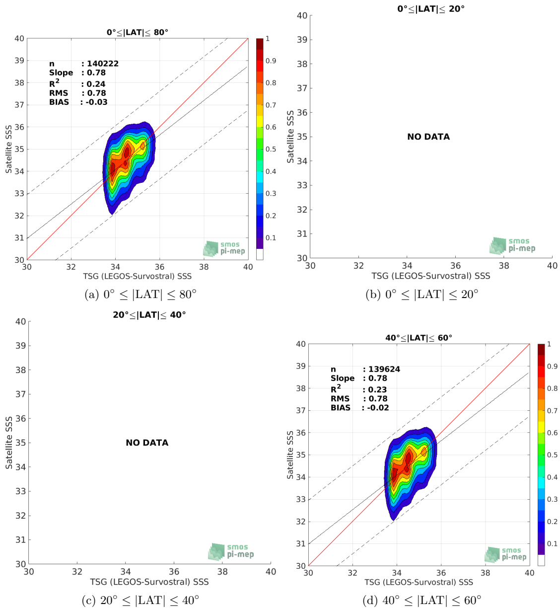
Figure 9: Contour maps of the concentration of SMAP SSS L2 v4 (RSS) SSS (y-axis) versus TSG (LEGOS-Survostral) SSS (x-axis) at match-up pairs for different latitude bands. For each plot, the red line shows x=y . The black thin and dashed lines indicate a linear fit through the data cloud and the \pm 95\% confidence levels, respectively. The number match-up pairs n , the slope and R^2 coefficient of the linear fit, the root mean square (RMS) and the mean bias between satellite and in situ data are indicated for each latitude band in each plots.
