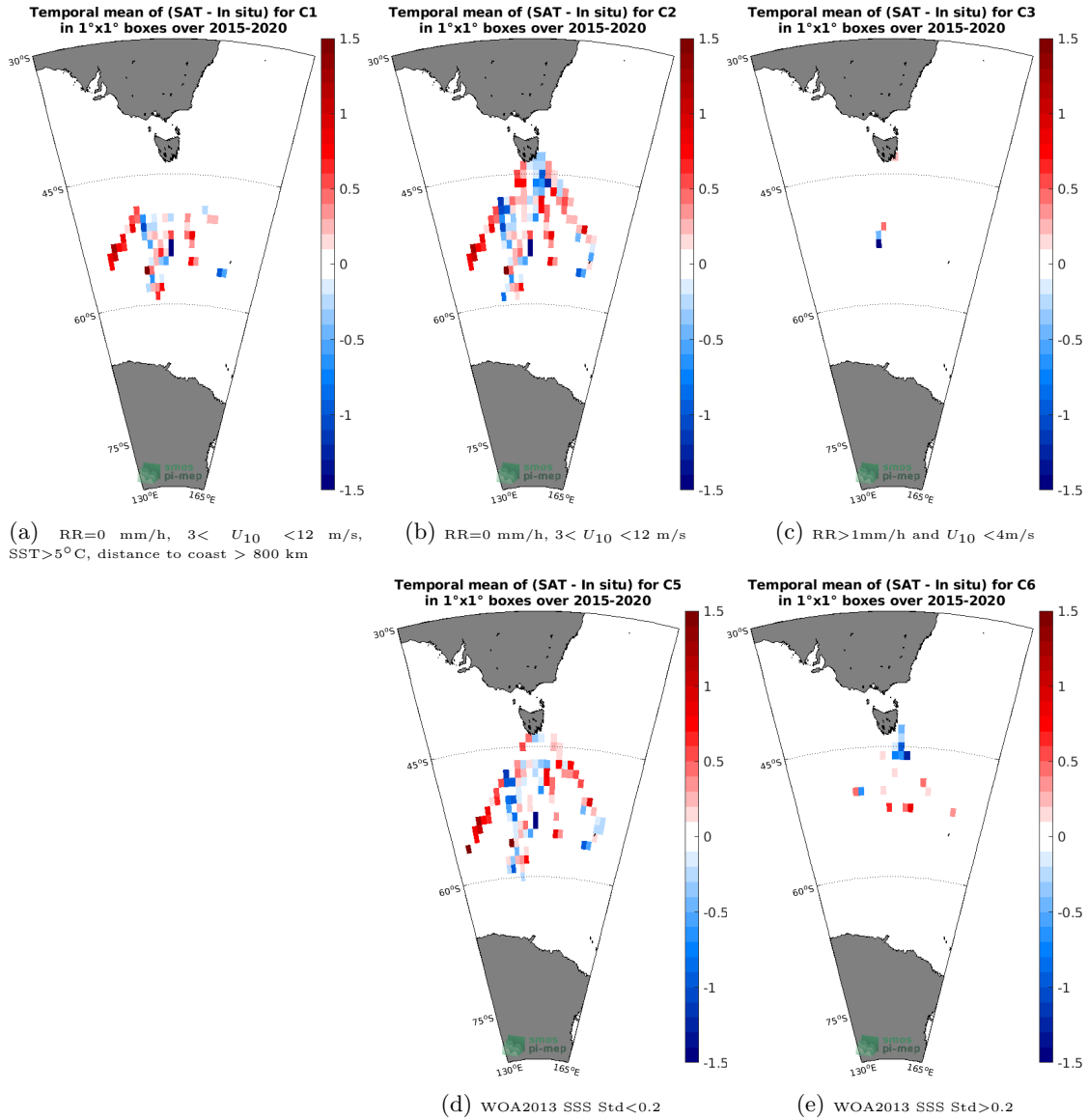
Figure 12: Temporal mean gridded over spatial boxes of size 1°x1° of \Delta SSS (SMAP SSS L2 v4 (RSS) - TSG (LEGOS-Survostral)) for 5 different subdatasets corresponding to:RR=0 mm/h, 3 < U_{10} < 12 m/s, SST>5°C, distance to coast > 800 km (a), RR=0 mm/h, 3 < U_{10} < 12 m/s (b), RR>1mm/h and U_{10} < 4 m/s (c), WOA2013 SSS Std<0.2 (d), WOA2013 SSS Std>0.2 (e).
