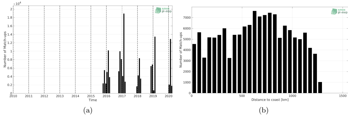
Figure 1: Number of match-ups between TSG (LEGOS-Survostral) and SMAP SSS L2 v4 (RSS) SSS as a function of time (a) and as function of the distance to coast (b) over the Global Ocean Pi-MEP region and for the full satellite product period.
