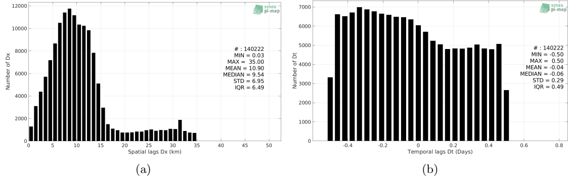
Figure 5: Histograms of the spatial (a) and temporal (b) lags between the location/time of the TSG (LEGOS-Survostral) measurement and the date of the corresponding SMAP SSS L2 v4 (RSS) SSS pixel.
