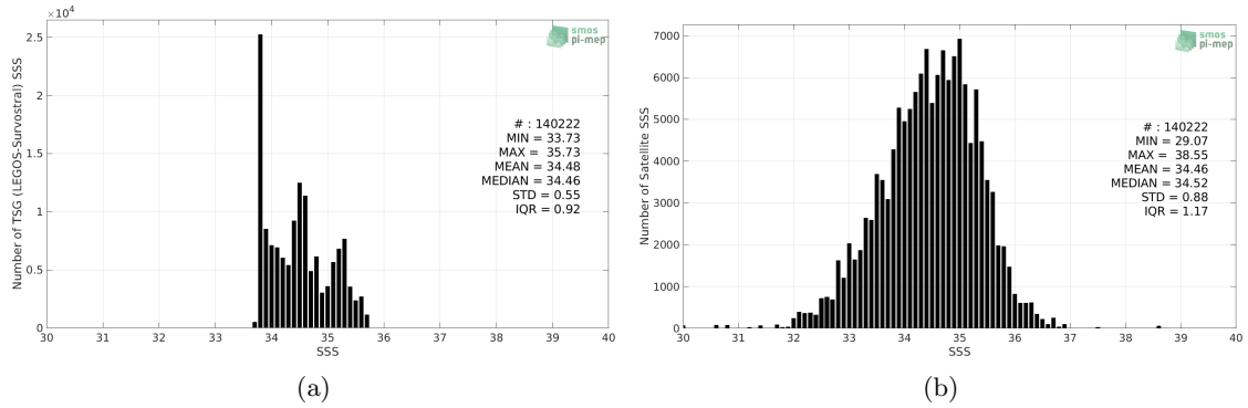
Figure 2: Histograms of SSS from TSG (LEGOS-Survostral) (a) and SMAP SSS L2 v4 (RSS) (b) considering all match-up pairs per bins of 0.1 over the Global Ocean Pi-MEP region and for the full satellite product period.
