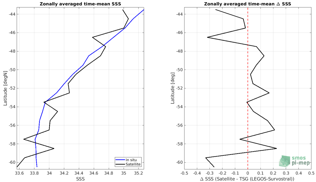
Figure 8: Left panel: Zonal mean SSS from SMAP SSS L2 v4 (RSS) satellite product (black) and from TSG (LEGOS-Survostral) (blue). Right panel: Zonal mean of \Delta SSS (Satellite - TSG (LEGOS-Survostral)) for all the collected Pi-MEP match-up pairs estimated over the full satellite product period.
