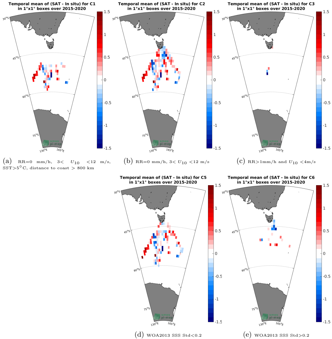
Figure 12: Temporal mean gridded over spatial boxes of size 1°x1° of \Delta SSS (SMAP SSS L2 v4 (RSS) - TSG (LEGOS-Survostral)) for 5 different subdatasets corresponding to:RR=0 mm/h, 3 < U_{10} < 12 m/s, SST>5°C, distance to coast > 800 km (a), RR=0 mm/h, 3 < U_{10} < 12 m/s (b), RR>1mm/h and U_{10} < 4 m/s (c), WOA2013 SSS Std<0.2 (d), WOA2013 SSS Std>0.2 (e).
