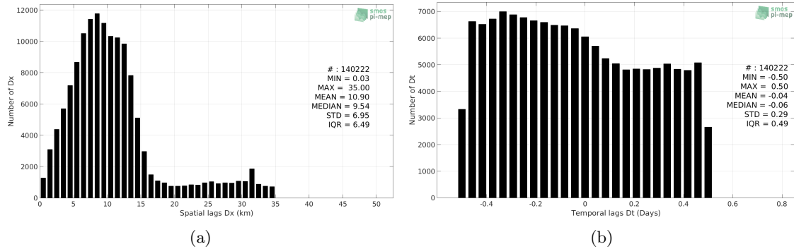
Figure 5: Histograms of the spatial (a) and temporal (b) lags between the time of the TSG (LEGOS-Survostral) measurements and the date of the corresponding SMAP SSS L2 v4 (RSS) SSS product.
