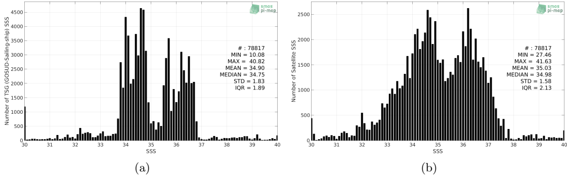
Figure 2: Histograms of SSS from TSG (GOSUD-Sailing-ship) (a) and SMAP SSS L2 v4 (RSS) (b) considering all match-up pairs per bins of 0.1 over the Global Ocean Pi-MEP region and for the full satellite product period.
