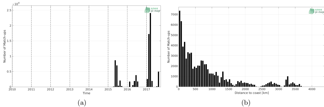
Figure 1: Number of match-ups between TSG (GOSUD-Sailing-ship) and SMAP SSS L2 v4 (RSS) SSS as a function of time (a) and as function of the distance to coast (b) over the Global Ocean Pi-MEP region and for the full satellite product period.
