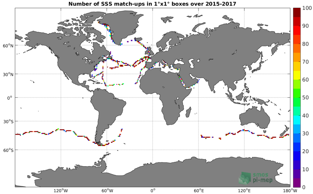
Figure 4: Number of SSS match-ups between TSG (GOSUD-Sailing-ship) SSS and the SMAP SSS L2 v4 (RSS) SSS product for the Global Ocean Pi-MEP region over 1°x1° boxes and for the full satellite product period.
