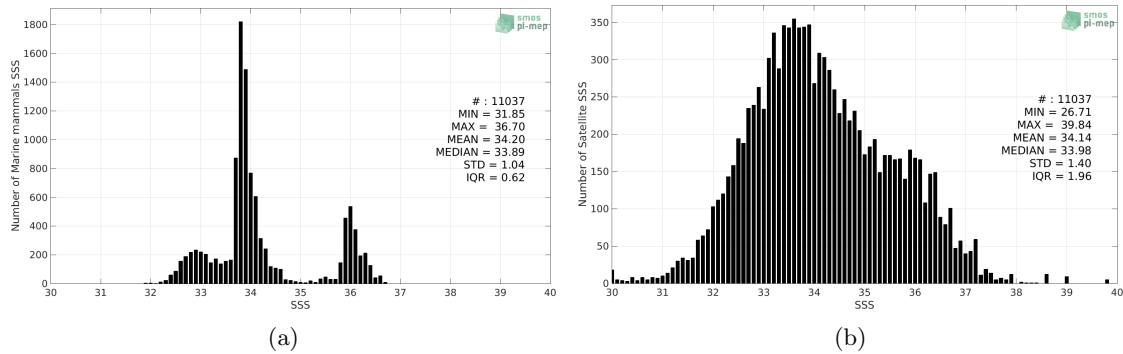
Figure 2: Histograms of SSS from Marine mammals (a) and SMAP SSS L2 v4 (RSS) (b) considering all match-up pairs per bins of 0.1 over the Global Ocean Pi-MEP region and for the full satellite product period.
