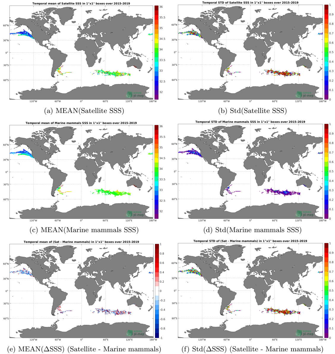
Figure 6: Temporal mean (left) and Std (right) of SSS from SMAP SSS L2 v4 (RSS) (top), Marine mammals (middle), and of \Delta SSS (Satellite - Marine mammals). Only match-up pairs are used to generate these maps.
