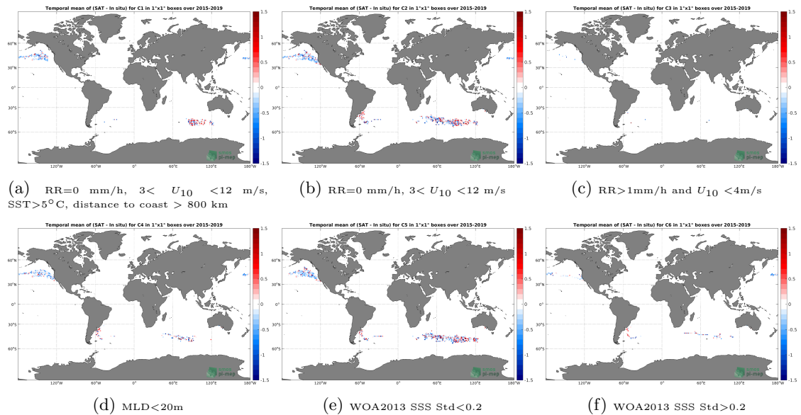
Figure 12: Temporal mean gridded over spatial boxes of size 1^\circ \times 1^\circ of \Delta SSS (SMAP SSS L2 v4 (RSS) - Marine mammals) for 6 different subdatasets corresponding to: RR=0 mm/h, 3 < U_{10} < 12 m/s, SST > 5°C, distance to coast > 800 km (a), RR=0 mm/h, 3 < U_{10} < 12 m/s (b), RR > 1mm/h and U_{10} < 4 m/s (c), MLD < 20m (d), WOA2013 SSS Std < 0.2 (e), WOA2013 SSS Std > 0.2 (f).
