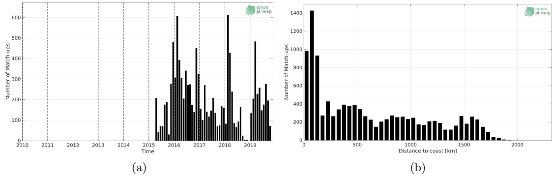
Figure 1: Number of match-ups between Marine mammals and SMAP SSS L2 v4 (RSS) SSS as a function of time (a) and as function of the distance to coast (b) over the Global Ocean Pi-MEP region and for the full satellite product period.
