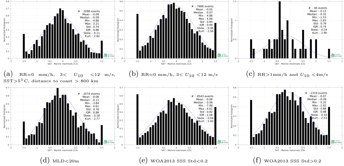
Figure 13: Normalized histogram of \Delta SSS (SMAP SSS L2 v4 (RSS) - Marine mammals) for 6 different subdatasets corresponding to: RR=0 mm/h, 3 < U_{10} < 12 m/s, SST>5°C, distance to coast > 800 km (a), RR=0 mm/h, 3 < U_{10} < 12 m/s (b), RR>1mm/h and U_{10} < 4 m/s (c), MLD<20m (d), WOA2013 SSS Std<0.2 (e), WOA2013 SSS Std>0.2 (f).
