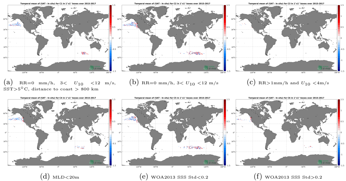
Figure 12: Temporal mean gridded over spatial boxes of size 1°x1° of \Delta SSS (SMAP SSS L2 v4 (RSS) - Sea mammals) for 6 different subdatasets corresponding to:RR=0 mm/h, 3 < U_{10} < 12 m/s, SST>5°C, distance to coast > 800 km (a), RR=0 mm/h, 3 < U_{10} < 12 m/s (b), RR>1mm/h and U_{10} <4m/s (c),MLD<20m (d),WOA2013 SSS Std<0.2 (e),WOA2013 SSS Std>0.2 (f).
