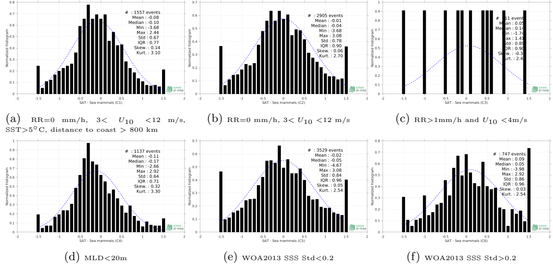
Figure 13: Normalized histogram of \Delta\text{SSS} (SMAP SSS L2 v4 (RSS) - Sea mammals) for 6 different subdatasets corresponding to: \text{RR}=0 \text{ mm/h} , 3 < U_{10} < 12 \text{ m/s} , \text{SST} > 5^\circ\text{C} , distance to coast > 800 \text{ km} (a), \text{RR}=0 \text{ mm/h} , 3 < U_{10} < 12 \text{ m/s} (b), \text{RR} > 1 \text{ mm/h} and U_{10} < 4 \text{ m/s} (c), \text{MLD} < 20 \text{ m} (d), \text{WOA2013 SSS Std} < 0.2 (e), \text{WOA2013 SSS Std} > 0.2 (f).
