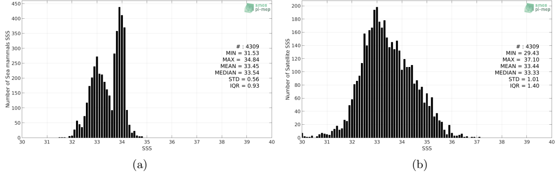
Figure 2: Histograms of SSS from Sea mammals (a) and SMAP SSS L2 v4 (RSS) (b) considering all match-up pairs per bins of 0.1 over the Global Ocean Pi-MEP region and for the full satellite product period.
