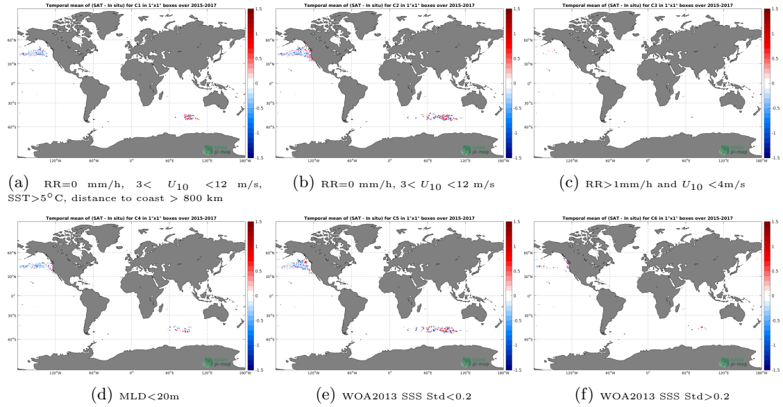
Figure 12: Temporal mean gridded over spatial boxes of size 1^\circ \times 1^\circ of \Delta SSS (SMAP SSS L2 v4 (RSS) - Sea mammals) for 6 different subdatasets corresponding to: RR=0 mm/h, 3 < U_{10} < 12 m/s, SST > 5^\circ C , distance to coast > 800 km (a), RR=0 mm/h, 3 < U_{10} < 12 m/s (b), RR > 1 mm/h and U_{10} < 4 m/s (c), MLD < 20 m (d), WOA2013 SSS Std < 0.2 (e), WOA2013 SSS Std > 0.2 (f).
