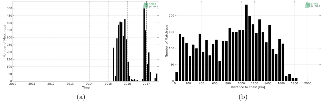
Figure 1: Number of match-ups between Sea mammals and SMAP SSS L2 v4 (RSS) SSS as a function of time (a) and as function of the distance to coast (b) over the Global Ocean Pi-MEP region and for the full satellite product period.
