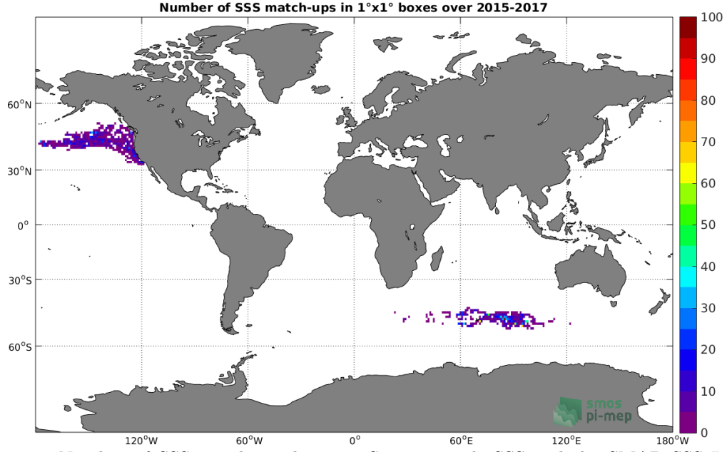
Figure 4: Number of SSS match-ups between Sea mammals SSS and the SMAP SSS L2 v4 (RSS) SSS product for the Global Ocean Pi-MEP region over 1°x1° boxes and for the full satellite product period.
