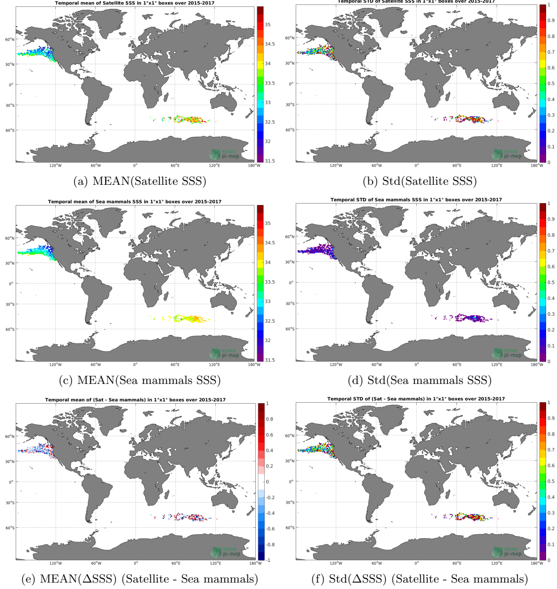
Figure 6: Temporal mean (left) and Std (right) of SSS from SMAP SSS L2 v4 (RSS) (top), Sea mammals (middle), and of \Delta SSS (Satellite - Sea mammals). Only match-up pairs are used to generate these maps.
