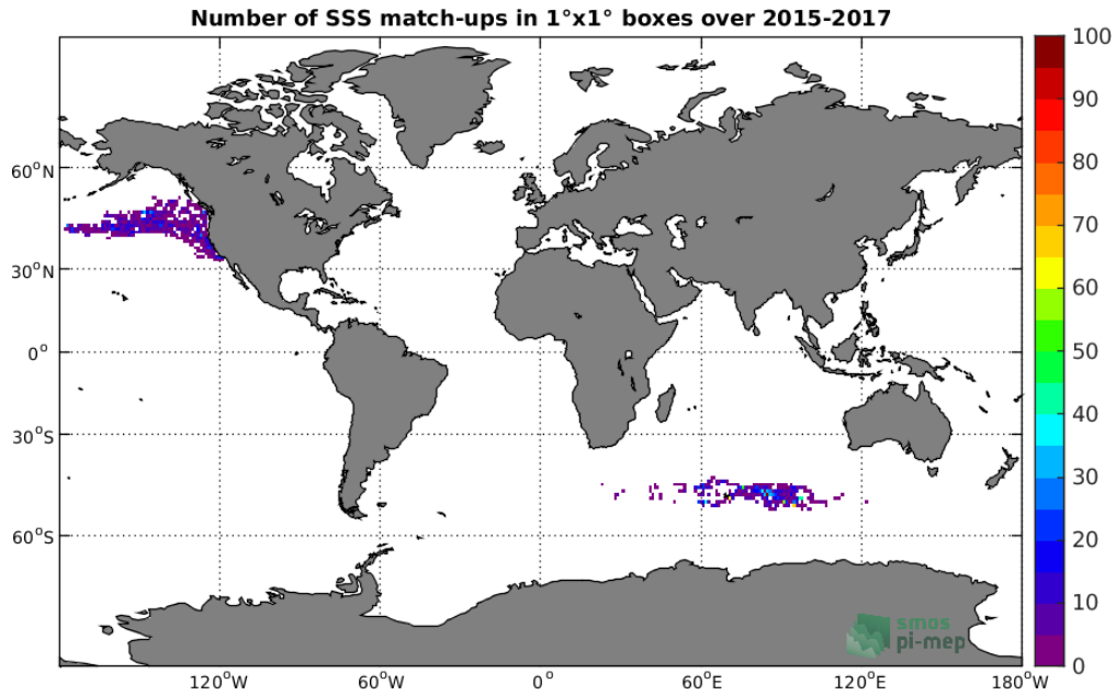
Figure 4: Number of SSS match-ups between Sea mammals SSS and the SMAP-L2-RSS-V4 SSS product for the Global Ocean Pi-MEP region over 1°x1° boxes and for the full satellite product period.
