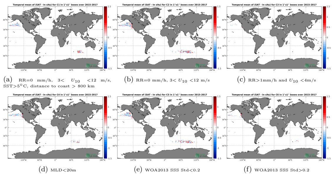
Figure 12: Temporal mean gridded over spatial boxes of size 1^\circ \times 1^\circ of \Delta SSS (SMAP-L2-RSS-V4 - Sea mammals) for 6 different subdatasets corresponding to:RR=0 mm/h, 3 < U_{10} < 12 m/s, SST >5^\circ C, distance to coast > 800 km (a), RR=0 mm/h, 3 < U_{10} < 12 m/s (b), RR >1 mm/h and U_{10} < 4 m/s (c),MLD <20 m (d),WOA2013 SSS Std <0.2 (e),WOA2013 SSS Std >0.2 (f).
