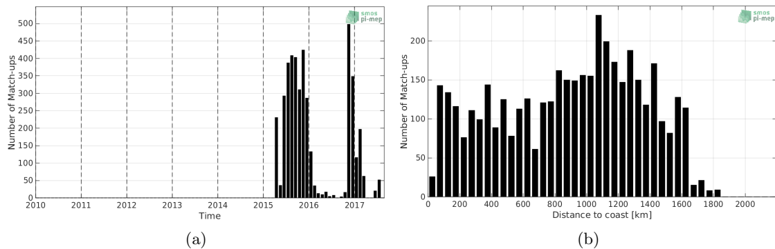
Figure 1: Number of match-ups between Sea mammals and SMAP-L2-RSS-V4 SSS as a function of time (a) and as function of the distance to coast (b) over the Global Ocean Pi-MEP region and for the full satellite product period.
