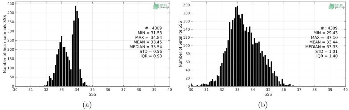
Figure 2: Histograms of SSS from Sea mammals (a) and SMAP-L2-RSS-V4 (b) considering all match-up pairs per bins of 0.1 over the Global Ocean Pi-MEP region and for the full satellite product period.
