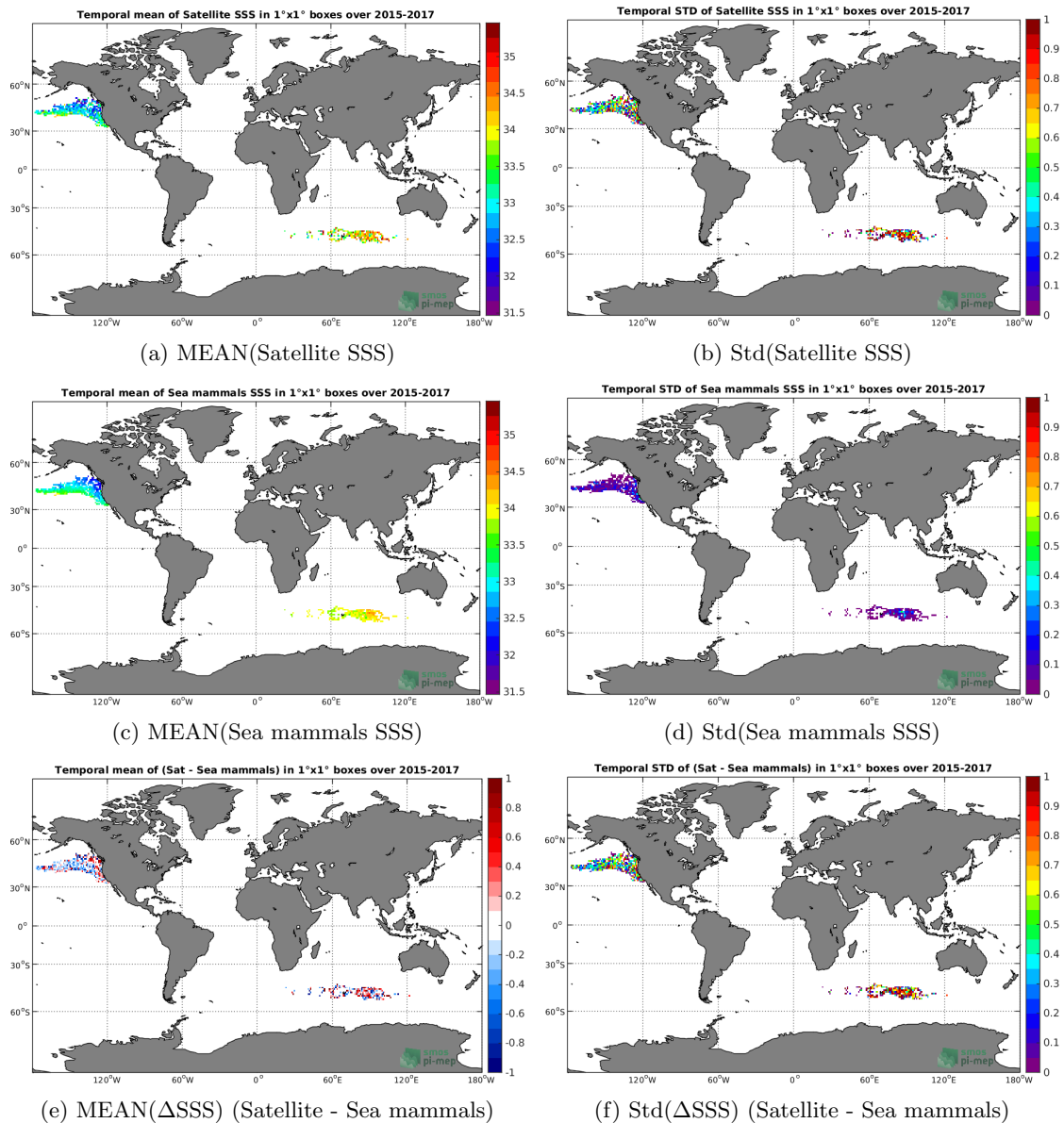
Figure 6: Temporal mean (left) and Std (right) of SSS from SMAP-L2-RSS-V4 (top), Sea mammals (middle), and of \Delta SSS (Satellite - Sea mammals). Only match-up pairs are used to generate these maps.
