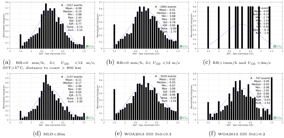
Figure 13: Normalized histogram of \Delta\text{SSS} (SMAP-L2-RSS-V4 - Sea mammals) for 6 different subdatasets corresponding to: RR=0 mm/h, 3 < U_{10} < 12 m/s, SST>5°C, distance to coast > 800 km (a), RR=0 mm/h, 3 < U_{10} < 12 m/s (b), RR>1mm/h and U_{10} < 4 m/s (c), MLD<20m (d), WOA2013 SSS Std<0.2 (e), WOA2013 SSS Std>0.2 (f).
