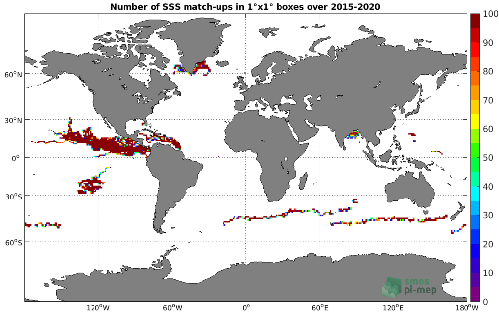
Figure 3: Number of SSS match-ups between Surface drifters SSS and the SMAP SSS L2 v4 (RSS) SSS product for the Global Ocean Pi-MEP region over 1^\circ \times 1^\circ boxes and for the full satellite product period.
