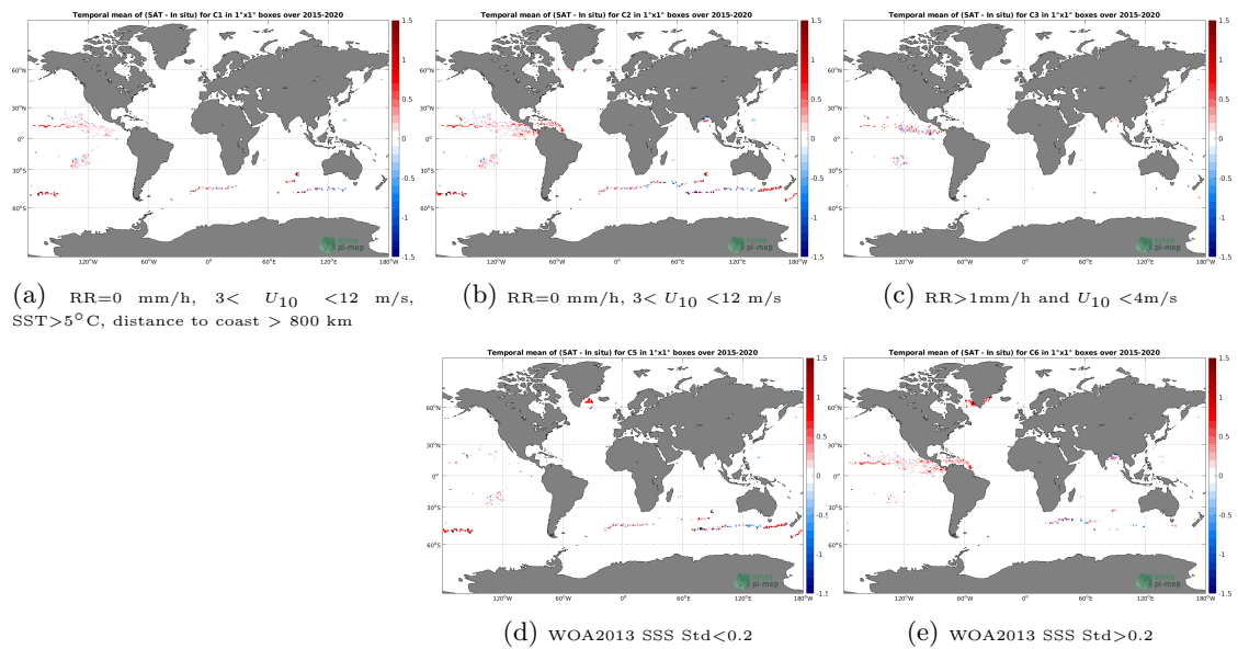
Figure 11: Temporal mean gridded over spatial boxes of size 1^\circ \times 1^\circ of \Delta SSS (SMAP SSS L2 v4 (RSS) - Surface drifters) for 5 different subdatasets corresponding to:RR=0 mm/h, 3 < U_{10} < 12 m/s, SST>5°C, distance to coast > 800 km (a), RR=0 mm/h, 3 < U_{10} < 12 m/s (b), RR>1mm/h and U_{10} < 4 m/s (c), WOA2013 SSS Std<0.2 (d), WOA2013 SSS Std>0.2 (e).
