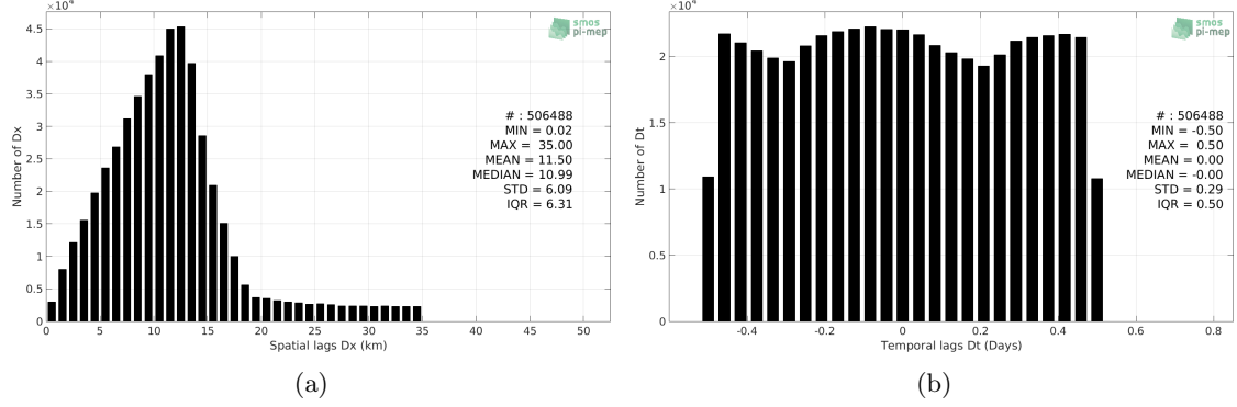
Figure 4: Histograms of the spatial (a) and temporal (b) lags between the time of the Surface drifters measurements and the date of the corresponding SMAP SSS L2 v4 (RSS) SSS product.
