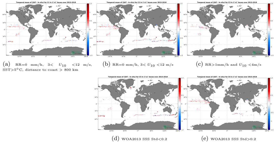
Figure 11: Temporal mean gridded over spatial boxes of size 1^\circ \times 1^\circ of \Delta SSS (SMAP SSS L2 v4 (RSS) - Surface drifters) for 5 different subdatasets corresponding to: RR=0 mm/h, 3 < U_{10} < 12 m/s, SST > 5^\circ\text{C} , distance to coast > 800 km (a), RR=0 mm/h, 3 < U_{10} < 12 m/s (b), RR > 1 mm/h and U_{10} < 4 m/s (c), WOA2013 SSS Std < 0.2 (d), WOA2013 SSS Std > 0.2 (e).
