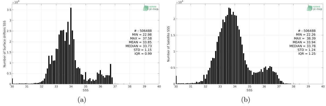
Figure 2: Histograms of SSS from Surface drifters (a) and SMAP SSS L2 v4 (RSS) (b) considering all match-up pairs per bins of 0.1 over the Global Ocean Pi-MEP region and for the full satellite product period.
