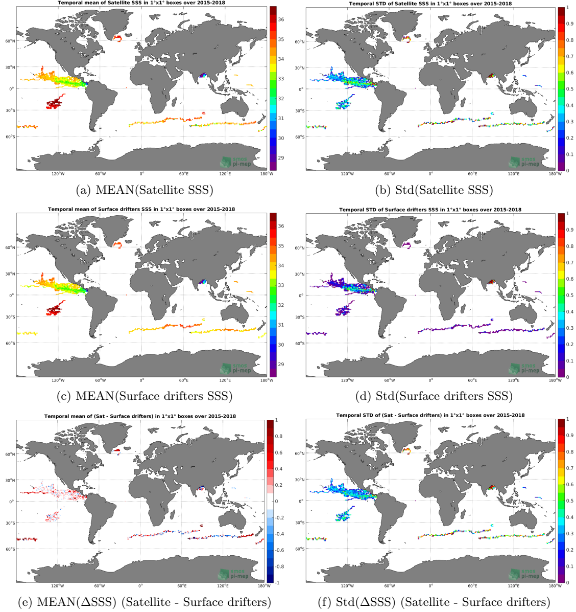
Figure 5: Temporal mean (left) and Std (right) of SSS from SMAP SSS L2 v4 (RSS) (top), Surface drifters (middle), and of \Delta SSS (Satellite - Surface drifters). Only match-up pairs are used to generate these maps.
