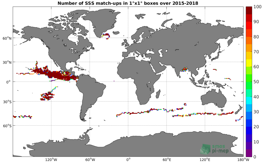
Figure 3: Number of SSS match-ups between Surface drifters SSS and the SMAP SSS L2 v4 (RSS) SSS product for the Global Ocean Pi-MEP region over 1°x1° boxes and for the full satellite product period.
