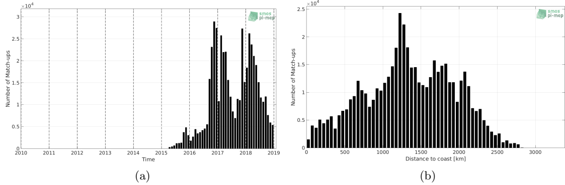
Figure 1: Number of match-ups between Surface drifters and SMAP SSS L2 v4 (RSS) SSS as a function of time (a) and as function of the distance to coast (b) over the Global Ocean Pi-MEP region and for the full satellite product period.
