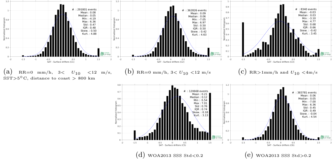
Figure 12: Normalized histogram of \Delta SSS (SMAP SSS L2 v4 (RSS) - Surface drifters) for 5 different subdatasets corresponding to: RR=0 mm/h, 3 < U_{10} < 12 m/s, SST>5°C, distance to coast > 800 km (a), RR=0 mm/h, 3 < U_{10} < 12 m/s (b), RR>1mm/h and U_{10} < 4 m/s (c), WOA2013 SSS Std<0.2 (d), WOA2013 SSS Std>0.2 (e).
