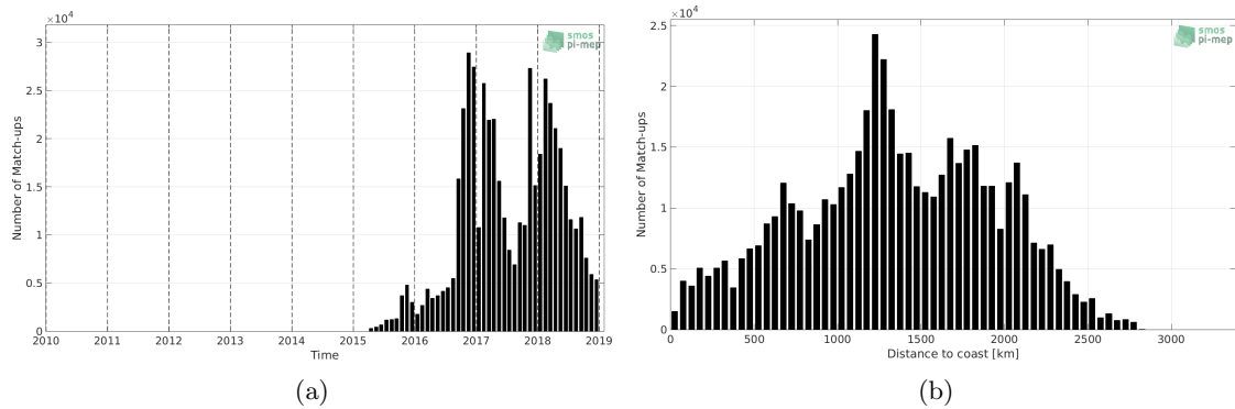
Figure 1: Number of match-ups between Surface drifters and SMAP-L2-RSS-V4 SSS as a function of time (a) and as function of the distance to coast (b) over the Global Ocean Pi-MEP region and for the full satellite product period.
