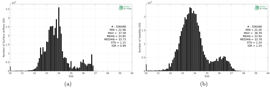
Figure 2: Histograms of SSS from Surface drifters (a) and SMAP-L2-RSS-V4 (b) considering all match-up pairs per bins of 0.1 over the Global Ocean Pi-MEP region and for the full satellite product period.
