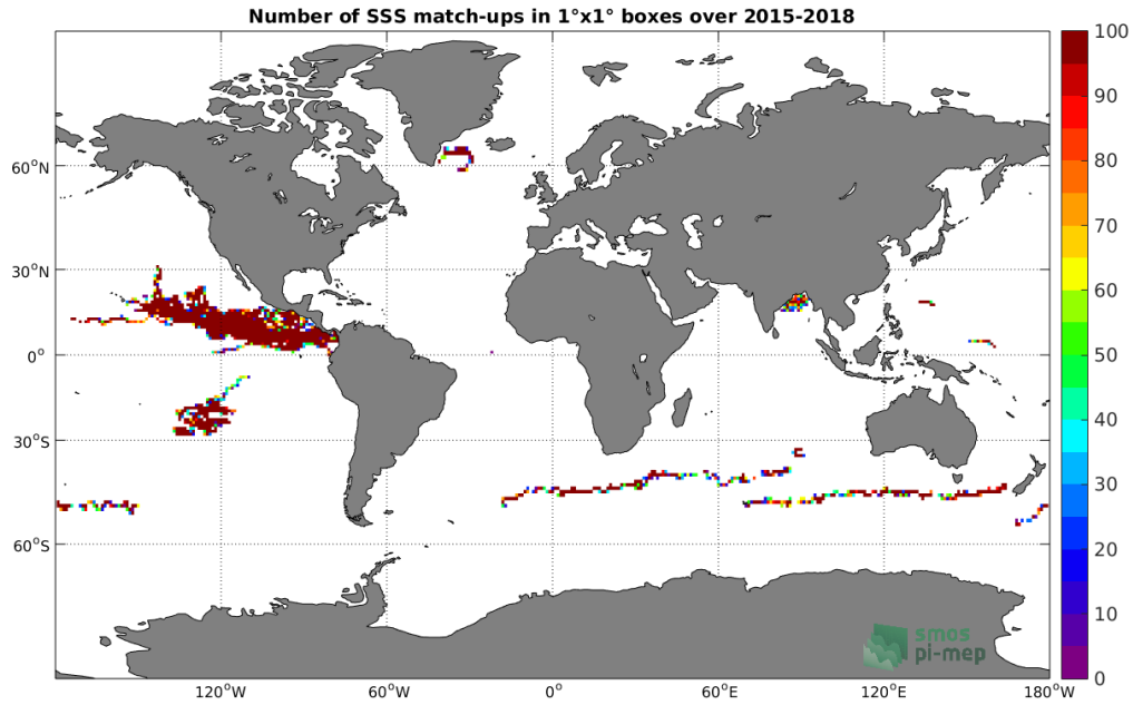
Figure 3: Number of SSS match-ups between Surface drifters SSS and the SMAP-L2-RSS-V4 SSS product for the Global Ocean Pi-MEP region over 1°x1° boxes and for the full satellite product period.
