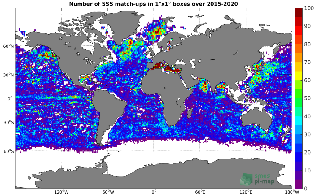
Figure 4: Number of SSS match-ups between Argo SSS and the SMAP SSS L2 v4 (RSS) SSS product for the Global Ocean Pi-MEP region over 1^\circ \times 1^\circ boxes and for the full satellite product period.
