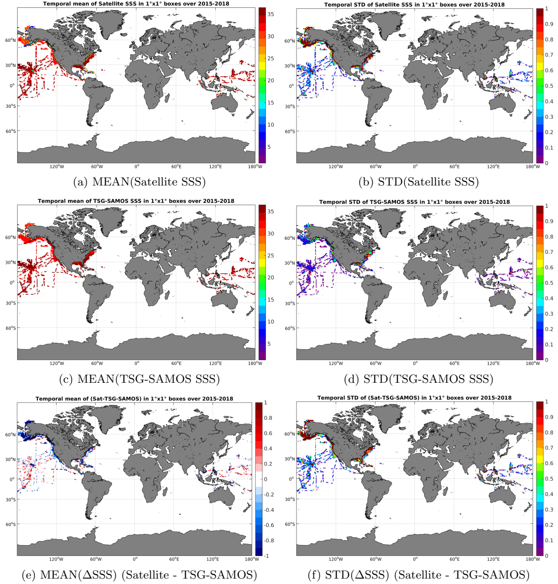
Figure 6: Temporal mean (left) and STD (right) of SSS from SMAP-L2-RSS-V2 (top), TSG-SAMOS (middle), and of \Delta SSS (Satellite - TSG-SAMOS). Only match-up pairs are used to generate these maps.
