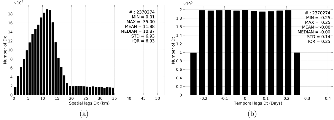
Figure 5: Histograms of the spatial (a) and temporal (b) lags between the time of the TSG-SAMOS measurements and the date of the corresponding SMAP-L2-RSS-V2 SSS product.
