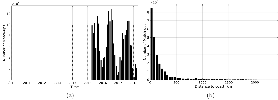
Figure 1: Number of match-ups between TSG-SAMOS and SMAP-L2-RSS-V2 SSS as a function of time (a) and as function of the distance to coast (b) over the Global Ocean Pi-MEP region and for the full satellite product period.
