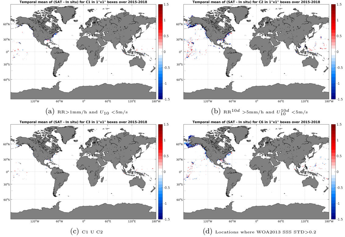
Figure 12: Temporal mean gridded over spatial boxes of size 1^\circ \times 1^\circ of \Delta SSS (SMAP-L2-RSS-V2 - TSG-SAMOS) for 4 different subdatasets corresponding to: RR > 1mm/h and U_{10} < 5 m/s (a), RR^{10d} > 5 mm/h and U_{10}^{10d} < 5 m/s (b), C1 U C2 (c), Locations where WOA2013 SSS STD > 0.2 (d).
