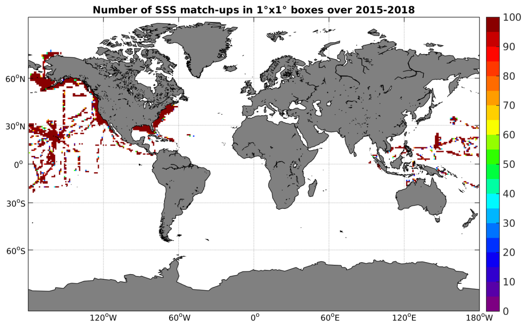
Figure 4: Number of SSS match-ups between TSG-SAMOS SSS and the SMAP-L2-RSS-V2 SSS product for the Global Ocean Pi-MEP region over 1^\circ \times 1^\circ boxes and for the full satellite product period.
