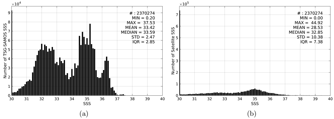
Figure 2: Histograms of SSS from TSG-SAMOS (a) and SMAP-L2-RSS-V2 (b) considering all match-up pairs per bins of 0.1 over the Global Ocean Pi-MEP region and for the full satellite product period.
