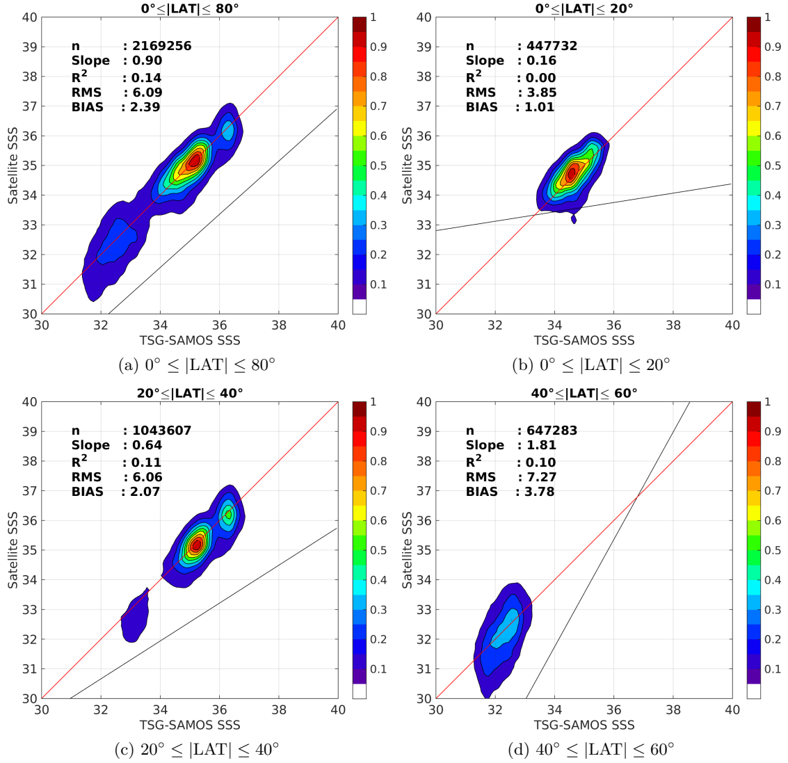
Figure 9: Contour maps of the concentration of SMAP-L2-RSS-V2 SSS (y-axis) versus TSG-SAMOS SSS (x-axis) at match-up pairs for different latitude bands. For each plot, the red line shows x=y . The black thin and dashed lines indicate a linear fit through the data cloud and the \pm 95\% confidence levels, respectively. The number match-up pairs n , the slope and R^2 coefficient of the linear fit, the root mean square (RMS) and the mean bias between satellite and in situ data are indicated for each latitude band in each plots.
