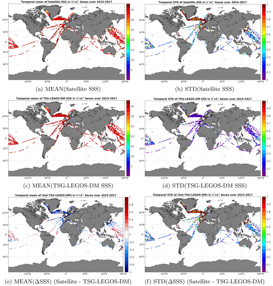
Figure 6: Temporal mean (left) and STD (right) of SSS from SMAP-L2-RSS-V2 (top), TSG-LEGOS-DM (middle), and of \Delta SSS (Satellite - TSG-LEGOS-DM). Only match-up pairs are used to generate these maps.
