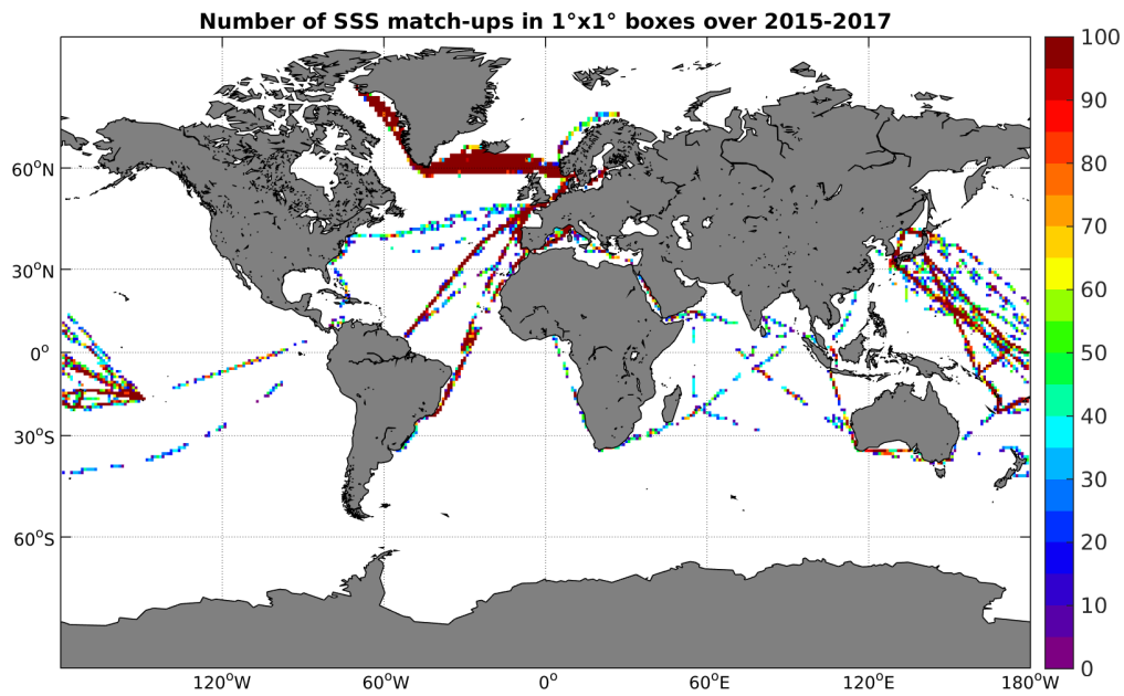
Figure 4: Number of SSS match-ups between TSG-LEGOS-DM SSS and the SMAP-L2-RSS-V2 SSS product for the Global Ocean Pi-MEP region over 1^\circ \times 1^\circ boxes and for the full satellite product period.
