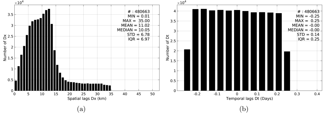
Figure 5: Histograms of the spatial (a) and temporal (b) lags between the time of the TSG-LEGOS-DM measurements and the date of the corresponding SMAP-L2-RSS-V2 SSS product.
