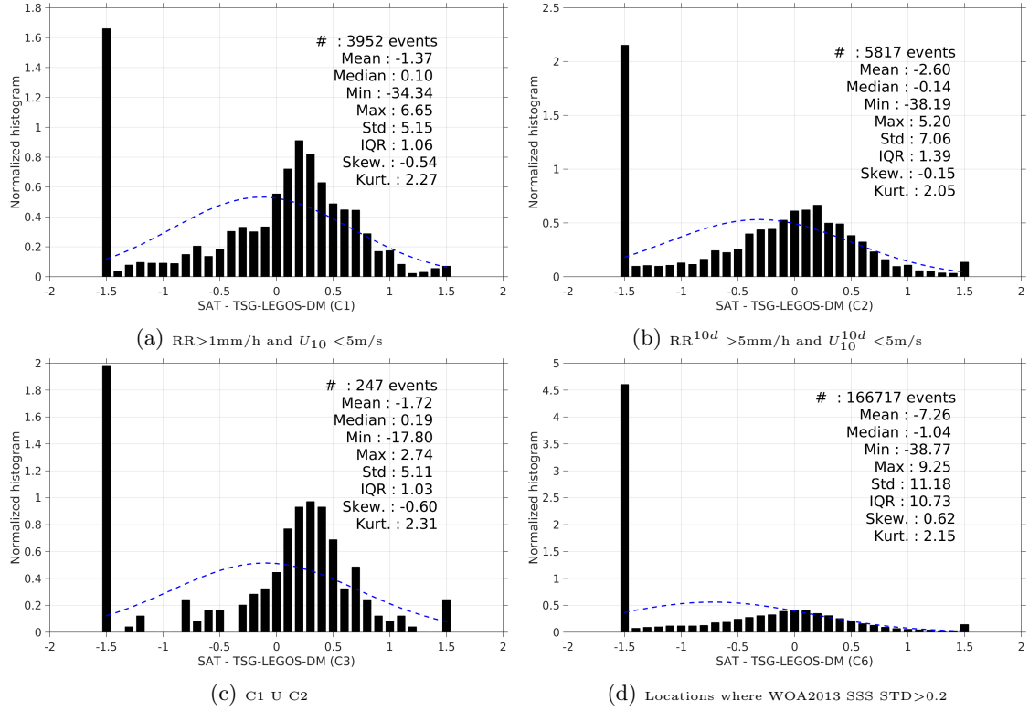
Figure 13: Normalized histogram of \Delta SSS (SMAP-L2-RSS-V2 - TSG-LEGOS-DM) for 6 different subdatasets corresponding to: RR > 1\text{mm/h} and U_{10} < 5\text{m/s} (a), RR^{10d} > 5\text{mm/h} and U_{10}^{10d} < 5\text{m/s} (b), C1 U C2 (c), Locations where WOA2013 SSS STD > 0.2 (d).
