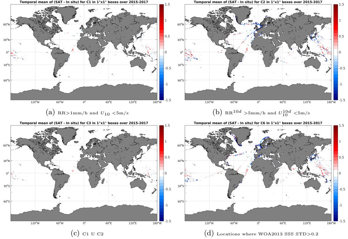
Figure 12: Temporal mean gridded over spatial boxes of size 1^\circ \times 1^\circ of \Delta SSS (SMAP-L2-RSS-V2 - TSG-LEGOS-DM) for 4 different subdatasets corresponding to: RR > 1\text{mm/h} and U_{10} < 5\text{m/s} (a), RR^{10d} > 5\text{mm/h} and U_{10}^{10d} < 5\text{m/s} (b), C1 U C2 (c), Locations where WOA2013 SSS STD > 0.2 (d).
