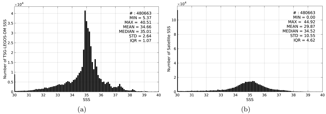
Figure 2: Histograms of SSS from TSG-LEGOS-DM (a) and SMAP-L2-RSS-V2 (b) considering all match-up pairs per bins of 0.1 over the Global Ocean Pi-MEP region and for the full satellite product period.
