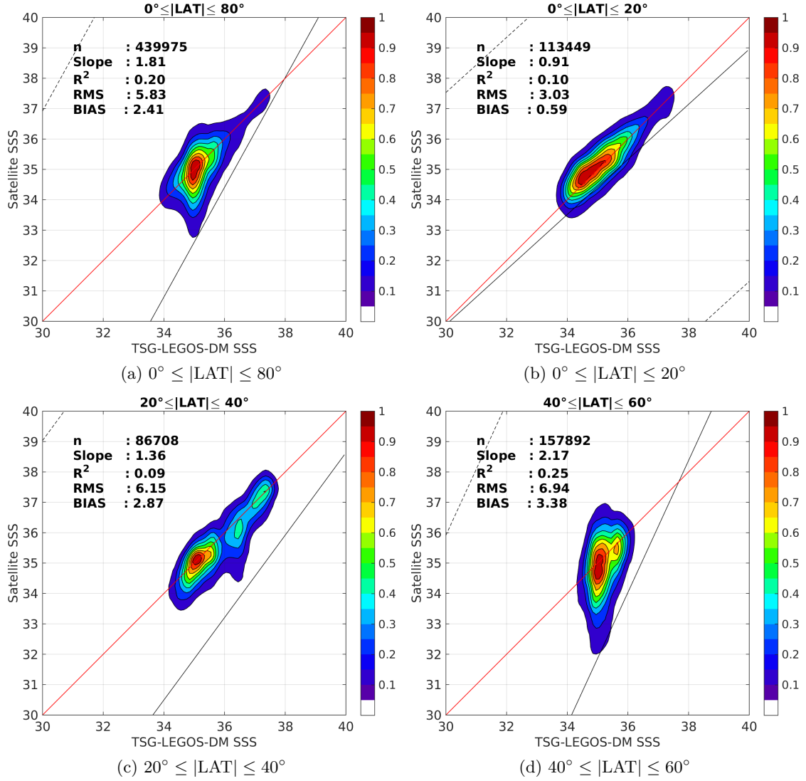
Figure 9: Contour maps of the concentration of SMAP-L2-RSS-V2 SSS (y-axis) versus TSG-LEGOS-DM SSS (x-axis) at match-up pairs for different latitude bands. For each plot, the red line shows x=y . The black thin and dashed lines indicate a linear fit through the data cloud and the \pm 95\% confidence levels, respectively. The number match-up pairs n , the slope and R^2 coefficient of the linear fit, the root mean square (RMS) and the mean bias between satellite and in situ data are indicated for each latitude band in each plots.
