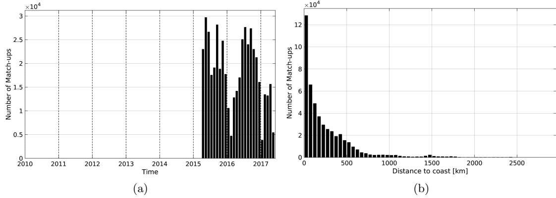
Figure 1: Number of match-ups between TSG-LEGOS-DM and SMAP-L2-RSS-V2 SSS as a function of time (a) and as function of the distance to coast (b) over the Global Ocean Pi-MEP region and for the full satellite product period.
