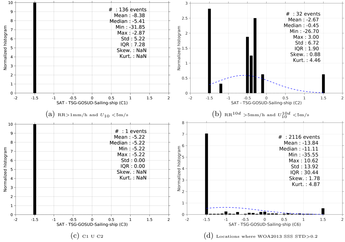
Figure 13: Normalized histogram of \Delta\text{SSS} (SMAP-L2-RSS-V2 - TSG-GOSUD-Sailing-ship) for 6 different subdatasets corresponding to: RR > 1mm/h and U_{10} < 5\text{m/s} (a), RR^{10d} > 5\text{mm/h} and U_{10}^{10d} < 5\text{m/s} (b), C1 U C2 (c), Locations where WOA2013 SSS STD > 0.2 (d).
