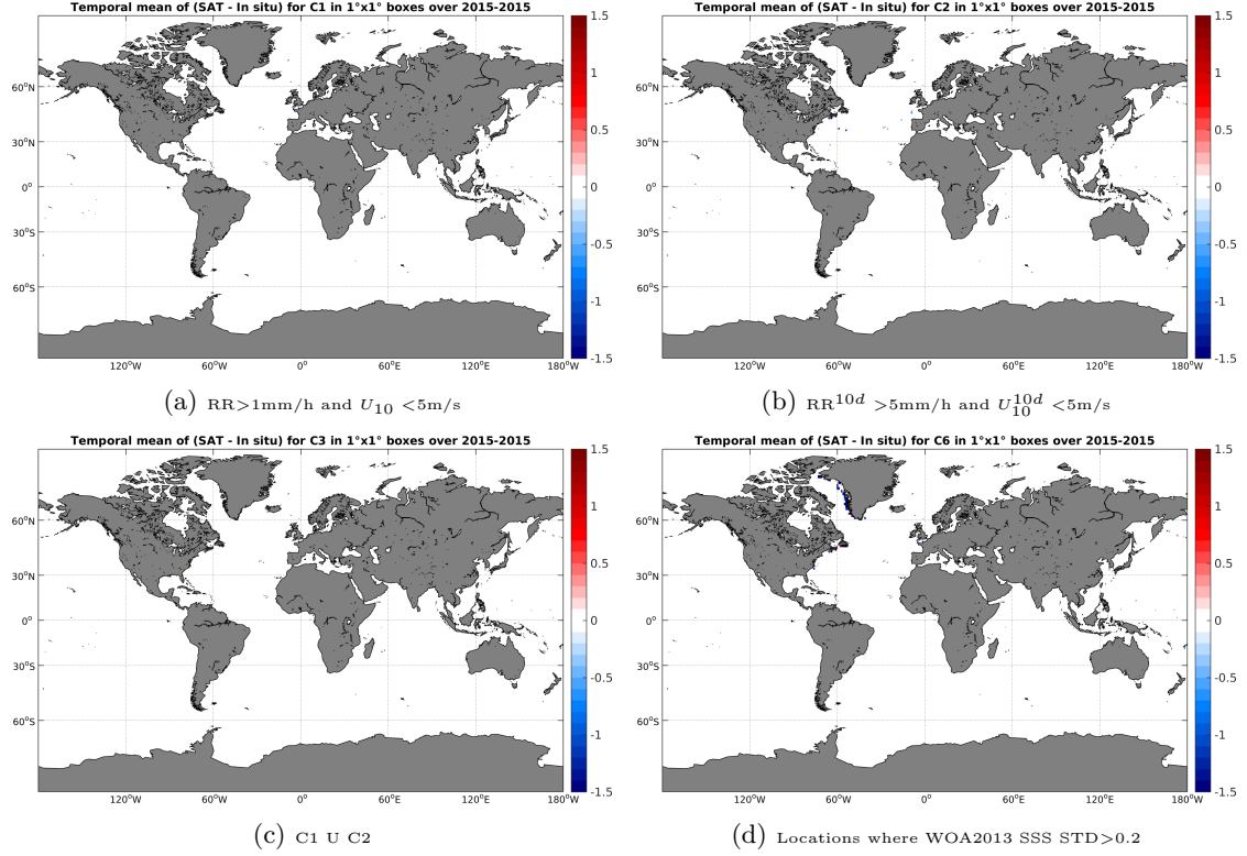
Figure 12: Temporal mean gridded over spatial boxes of size 1^\circ \times 1^\circ of \Delta SSS (SMAP-L2-RSS-V2 - TSG-GOSUD-Sailing-ship) for 4 different subdatasets corresponding to: RR > 1\text{mm/h} and U_{10} < 5\text{m/s} (a), RR^{10d} > 5\text{mm/h} and U_{10}^{10d} < 5\text{m/s} (b), C1 U C2 (c), Locations where WOA2013 SSS STD > 0.2 (d).
