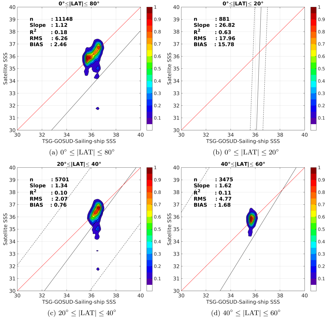
Figure 9: Contour maps of the concentration of SMAP-L2-RSS-V2 SSS (y-axis) versus TSG-GOSUD-Sailing-ship SSS (x-axis) at match-up pairs for different latitude bands. For each plot, the red line shows x=y . The black thin and dashed lines indicate a linear fit through the data cloud and the \pm 95\% confidence levels, respectively. The number match-up pairs n , the slope and R^2 coefficient of the linear fit, the root mean square (RMS) and the mean bias between satellite and in situ data are indicated for each latitude band in each plots.
