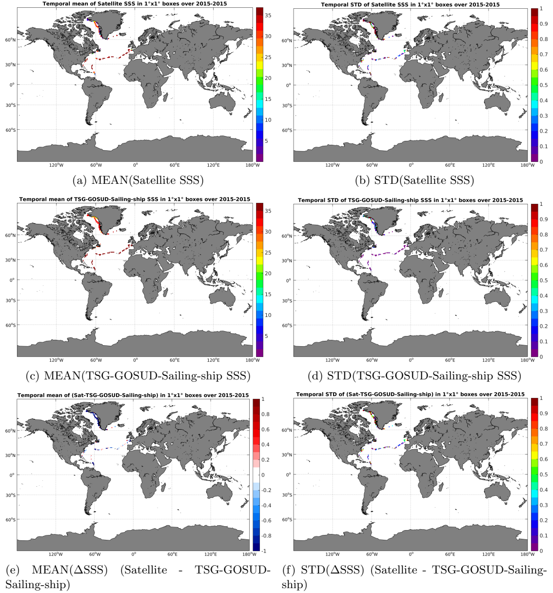
Figure 6: Temporal mean (left) and STD (right) of SSS from SMAP-L2-RSS-V2 (top), TSG-GOSUD-Sailing-ship (middle), and of \Delta SSS (Satellite - TSG-GOSUD-Sailing-ship). Only match-up pairs are used to generate these maps.
