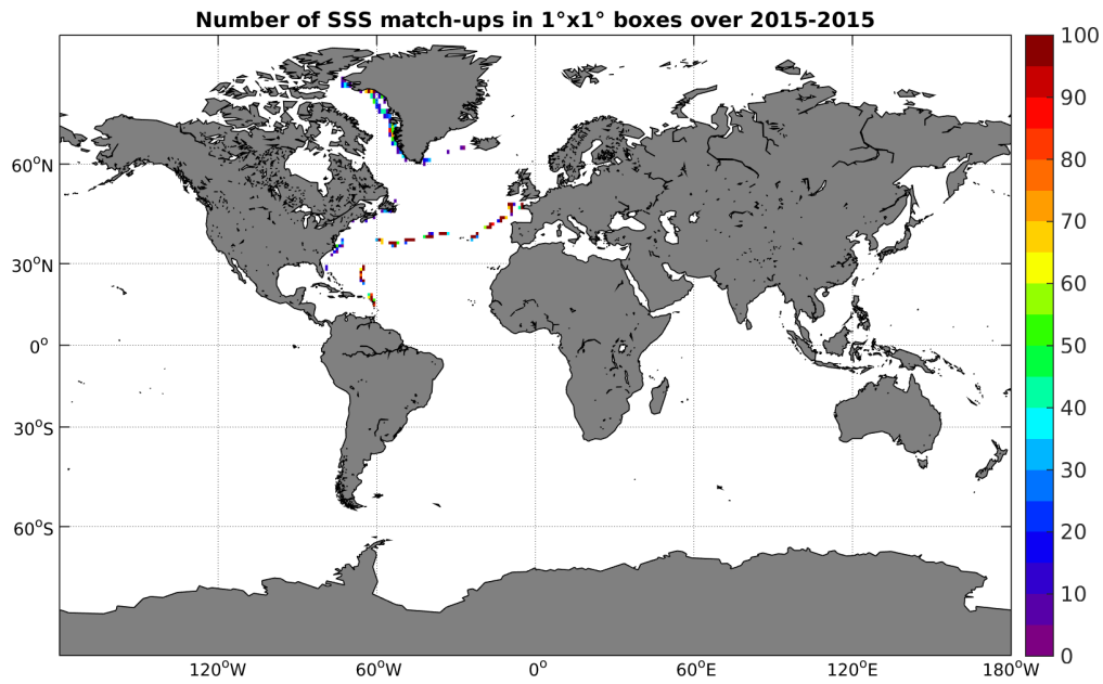
Figure 4: Number of SSS match-ups between TSG-GOSUD-Sailing-ship SSS and the SMAP-L2-RSS-V2 SSS product for the Global Ocean Pi-MEP region over 1^\circ \times 1^\circ boxes and for the full satellite product period.
