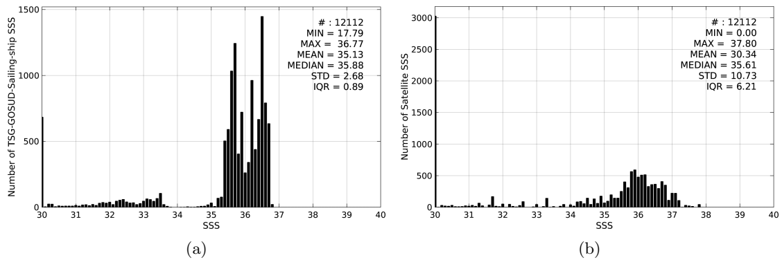
Figure 2: Histograms of SSS from TSG-GOSUD-Sailing-ship (a) and SMAP-L2-RSS-V2 (b) considering all match-up pairs per bins of 0.1 over the Global Ocean Pi-MEP region and for the full satellite product period.
