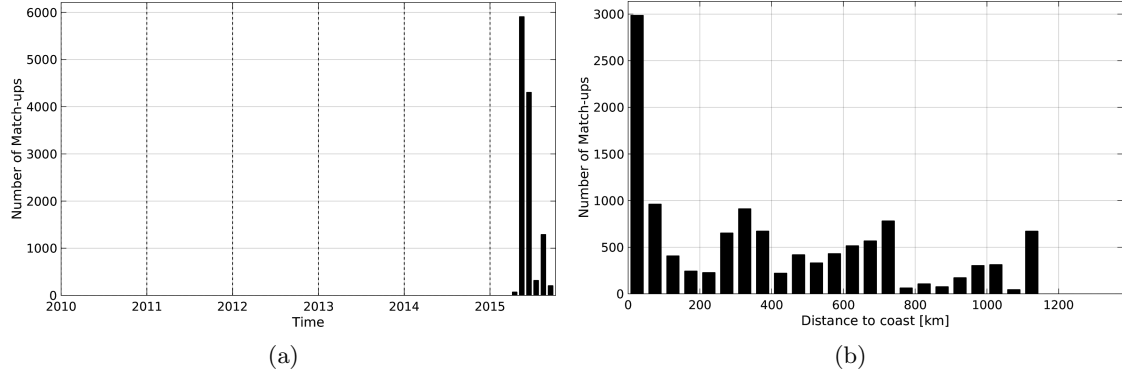
Figure 1: Number of match-ups between TSG-GOSUD-Sailing-ship and SMAP-L2-RSS-V2 SSS as a function of time (a) and as function of the distance to coast (b) over the Global Ocean Pi-MEP region and for the full satellite product period.
