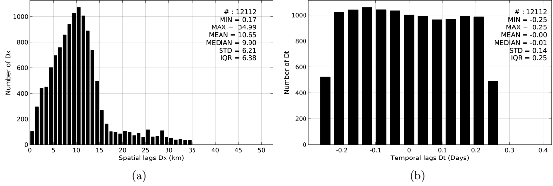
Figure 5: Histograms of the spatial (a) and temporal (b) lags between the time of the TSG-GOSUD-Sailing-ship measurements and the date of the corresponding SMAP-L2-RSS-V2 SSS product.
