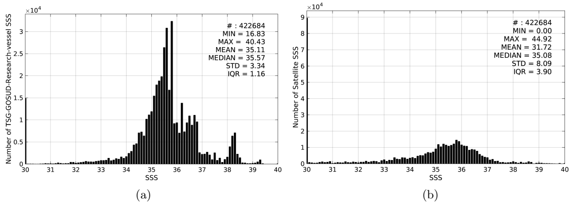
Figure 2: Histograms of SSS from TSG-GOSUD-Research-vessel (a) and SMAP-L2-RSS-V2 (b) considering all match-up pairs per bins of 0.1 over the Global Ocean Pi-MEP region and for the full satellite product period.
