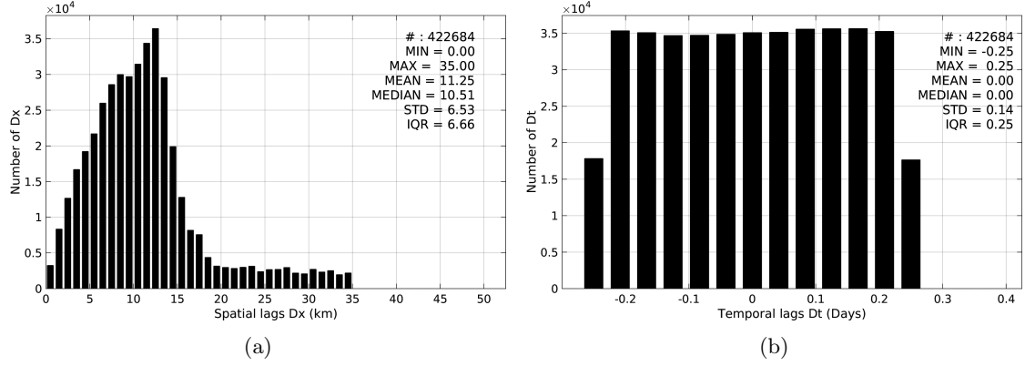
Figure 5: Histograms of the spatial (a) and temporal (b) lags between the time of the TSG-GOSUD-Research-vessel measurements and the date of the corresponding SMAP-L2-RSS-V2 SSS product.
