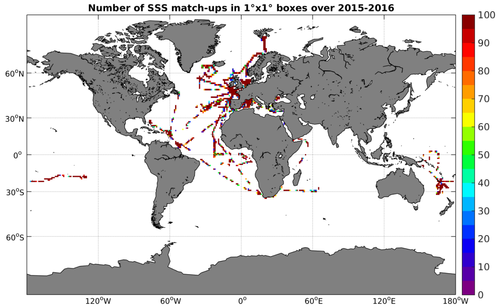
Figure 4: Number of SSS match-ups between TSG-GOSUD-Research-vessel SSS and the SMAP-L2-RSS-V2 SSS product for the Global Ocean Pi-MEP region over 1°x1° boxes and for the full satellite product period.
