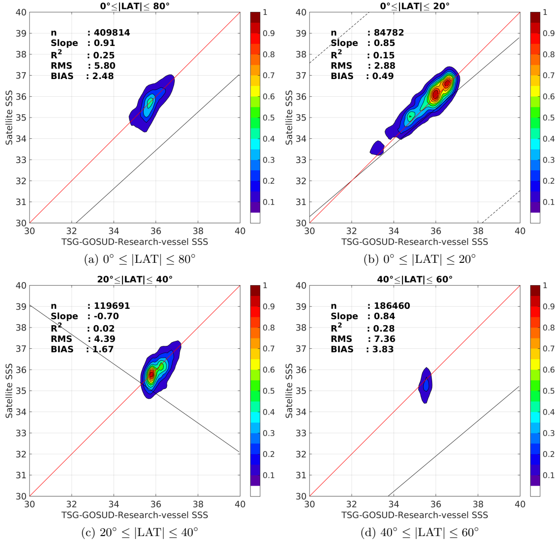
Figure 9: Contour maps of the concentration of SMAP-L2-RSS-V2 SSS (y-axis) versus TSG-GOSUD-Research-vessel SSS (x-axis) at match-up pairs for different latitude bands. For each plot, the red line shows x=y . The black thin and dashed lines indicate a linear fit through the data cloud and the \pm 95\% confidence levels, respectively. The number match-up pairs n , the slope and R^2 coefficient of the linear fit, the root mean square (RMS) and the mean bias between satellite and in situ data are indicated for each latitude band in each plots.
