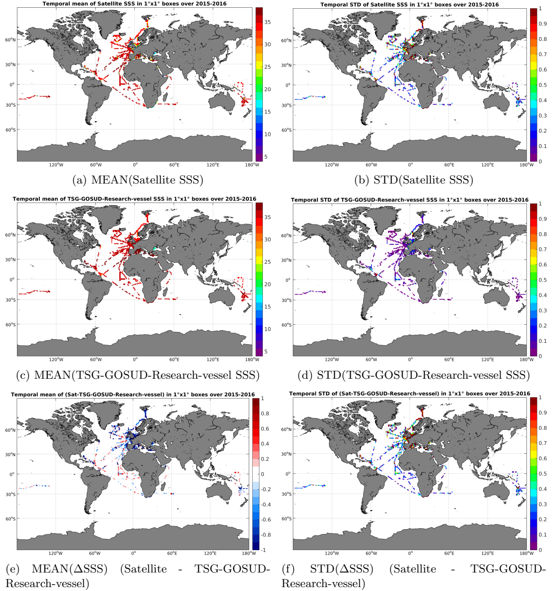
Figure 6: Temporal mean (left) and STD (right) of SSS from SMAP-L2-RSS-V2 (top), TSG-GOSUD-Research-vessel (middle), and of \Delta SSS (Satellite - TSG-GOSUD-Research-vessel). Only match-up pairs are used to generate these maps.
