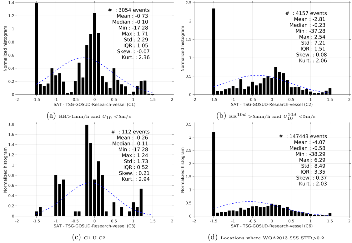
Figure 13: Normalized histogram of \Delta\text{SSS} (SMAP-L2-RSS-V2 - TSG-GOSUD-Research-vessel) for 6 different subdatasets corresponding to: \text{RR} > 1\text{mm/h} and U_{10} < 5\text{m/s} (a), \text{RR}^{10d} > 5\text{mm/h} and U_{10}^{10d} < 5\text{m/s} (b), \text{C1} \cup \text{C2} (c), Locations where WOA2013 SSS STD > 0.2 (d).
