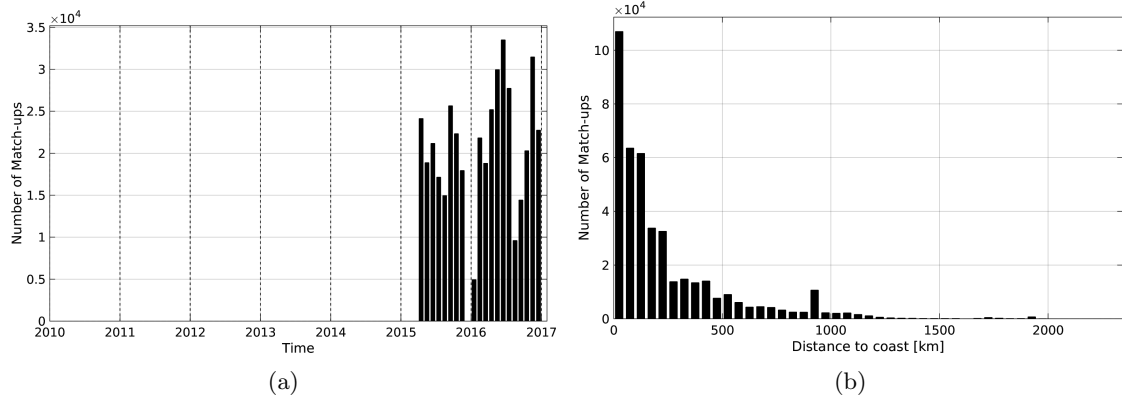
Figure 1: Number of match-ups between TSG-GOSUD-Research-vessel and SMAP-L2-RSS-V2 SSS as a function of time (a) and as function of the distance to coast (b) over the Global Ocean Pi-MEP region and for the full satellite product period.
