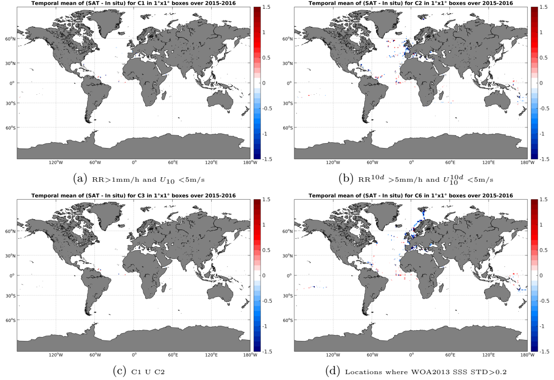
Figure 12: Temporal mean gridded over spatial boxes of size 1^\circ \times 1^\circ of \Delta SSS (SMAP-L2-RSS-V2 - TSG-GOSUD-Research-vessel) for 4 different subdatasets corresponding to: RR > 1\text{mm/h} and U_{10} < 5\text{m/s} (a), RR^{10d} > 5\text{mm/h} and U_{10}^{10d} < 5\text{m/s} (b), C1 U C2 (c), Locations where WOA2013 SSS STD > 0.2 (d).
