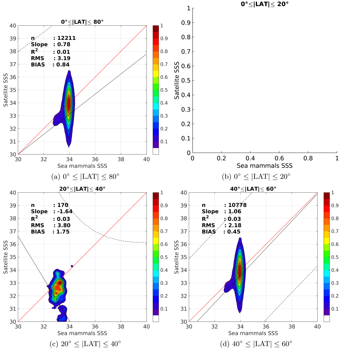
Figure 9: Contour maps of the concentration of SMAP-L2-RSS-V2 SSS (y-axis) versus Sea mammals SSS (x-axis) at match-up pairs for different latitude bands. For each plot, the red line shows x=y . The black thin and dashed lines indicate a linear fit through the data cloud and the \pm 95\% confidence levels, respectively. The number match-up pairs n , the slope and R^2 coefficient of the linear fit, the root mean square (RMS) and the mean bias between satellite and in situ data are indicated for each latitude band in each plots.
