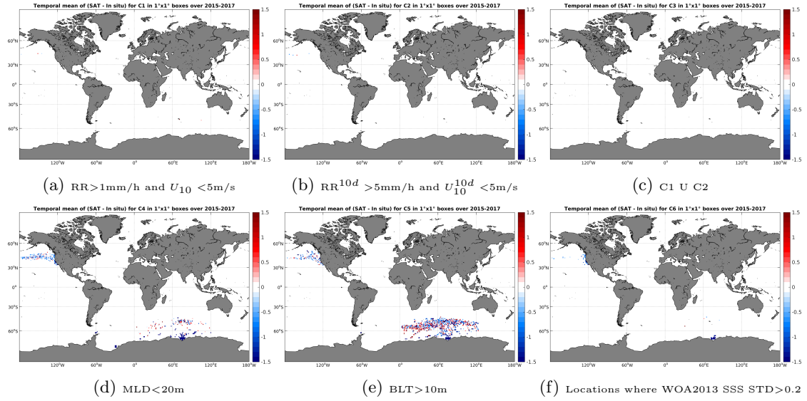
Figure 12: Temporal mean gridded over spatial boxes of size 1^\circ \times 1^\circ of \Delta SSS (SMAP-L2-RSS-V2 - Sea mammals) for 6 different subdatasets corresponding to: RR > 1\text{mm/h} and U_{10} < 5\text{m/s} (a), RR^{10d} > 5\text{mm/h} and U_{10}^{10d} < 5\text{m/s} (b), C1 U C2 (c), MLD < 20\text{m} (d), BLT > 10\text{m} (e), Locations where WOA2013 SSS STD > 0.2 (f).
