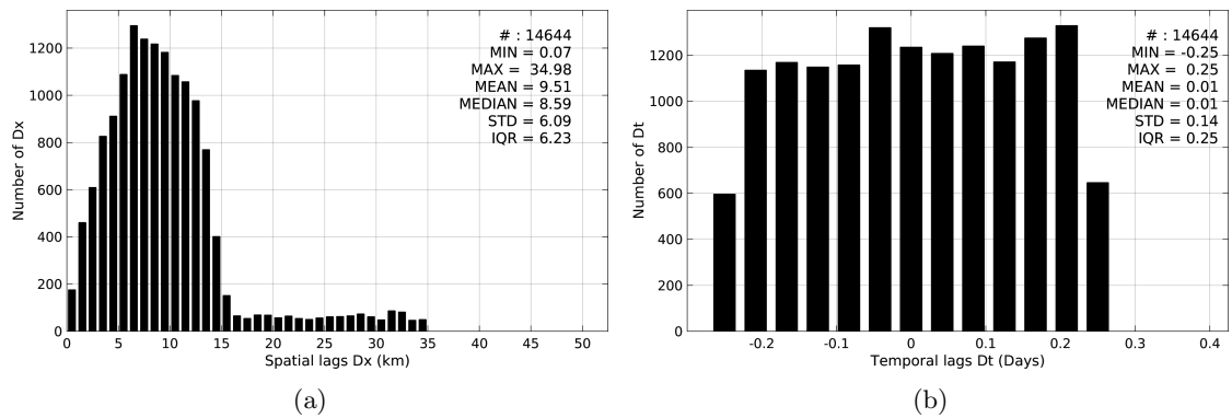
Figure 5: Histograms of the spatial (a) and temporal (b) lags between the time of the Sea mammals measurements and the date of the corresponding SMAP-L2-RSS-V2 SSS product.
