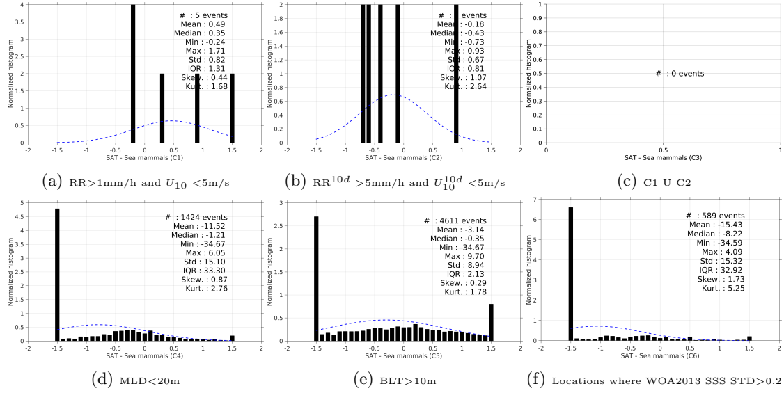
Figure 13: Normalized histogram of \Delta SSS (SMAP-L2-RSS-V2 - Sea mammals) for 6 different subdatasets corresponding to: RR > 1\text{mm/h} and U_{10} < 5\text{m/s} (a), RR^{10d} > 5\text{mm/h} and U_{10}^{10d} < 5\text{m/s} (b), C1 \cup C2 (c), MLD < 20\text{m} (d), BLT > 10\text{m} (e), Locations where WOA2013 SSS STD > 0.2 (f).
