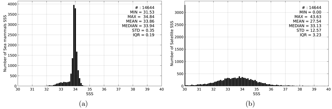
Figure 2: Histograms of SSS from Sea mammals (a) and SMAP-L2-RSS-V2 (b) considering all match-up pairs per bins of 0.1 over the Global Ocean Pi-MEP region and for the full satellite product period.
