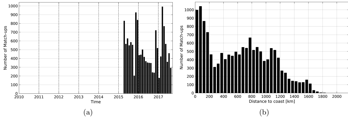
Figure 1: Number of match-ups between Sea mammals and SMAP-L2-RSS-V2 SSS as a function of time (a) and as function of the distance to coast (b) over the Global Ocean Pi-MEP region and for the full satellite product period.
