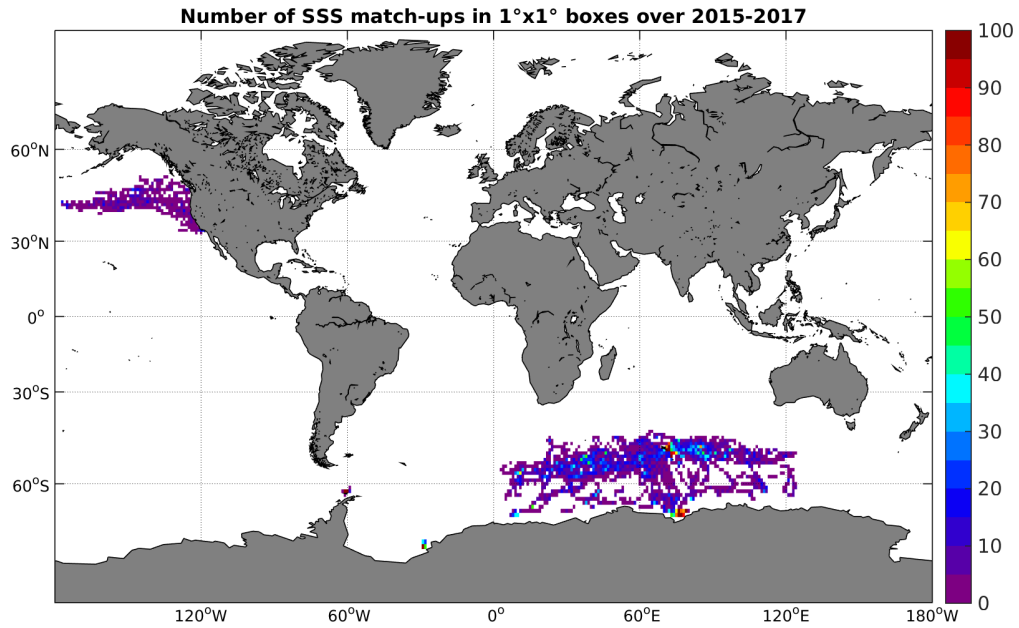
Figure 4: Number of SSS match-ups between Sea mammals SSS and the SMAP-L2-RSS-V2 SSS product for the Global Ocean Pi-MEP region over 1°x1° boxes and for the full satellite product period.
