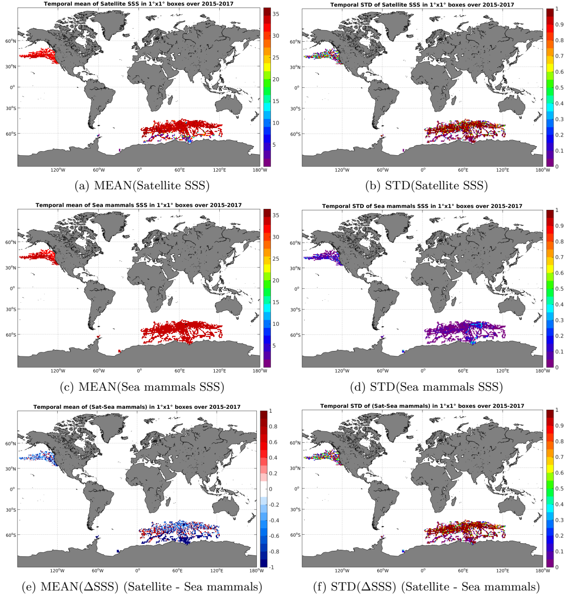
Figure 6: Temporal mean (left) and STD (right) of SSS from SMAP-L2-RSS-V2 (top), Sea mammals (middle), and of \Delta SSS (Satellite - Sea mammals). Only match-up pairs are used to generate these maps.
