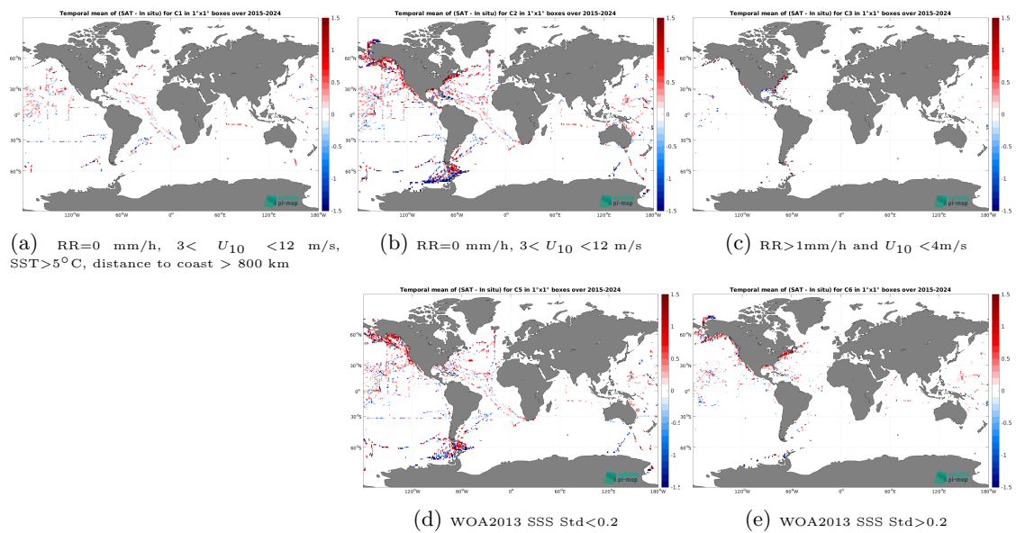
Figure 14: Temporal mean gridded over spatial boxes of size 1^\circ \times 1^\circ of \Delta\text{SSS} (SMAP SSS L2 v5.0 (JPL) - TSG (SAMOS)) for 5 different subdatasets corresponding to:RR=0 mm/h, 3 < U_{10} < 12 m/s, SST > 5^\circ\text{C} , distance to coast > 800 km (a), RR=0 mm/h, 3 < U_{10} < 12 m/s (b), RR > 1\text{mm/h} and U_{10} < 4\text{m/s} (c), WOA2013 SSS Std < 0.2 (d), WOA2013 SSS Std > 0.2 (e).
