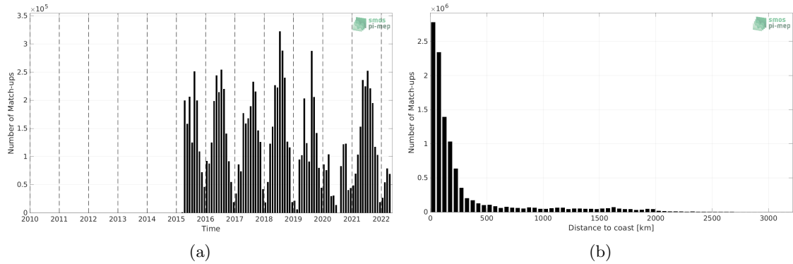
Figure 1: Number of match-ups between TSG (SAMOS) and SMAP SSS L2 v5.0 (JPL) SSS as a function of time (a) and as function of the distance to coast (b) over the Global Ocean Pi-MEP region and for the full satellite product period.
