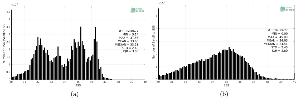
Figure 2: Histograms of SSS from TSG (SAMOS) (a) and SMAP SSS L2 v5.0 (JPL) (b) considering all match-up pairs per bins of 0.1 over the Global Ocean Pi-MEP region and for the full satellite product period.
