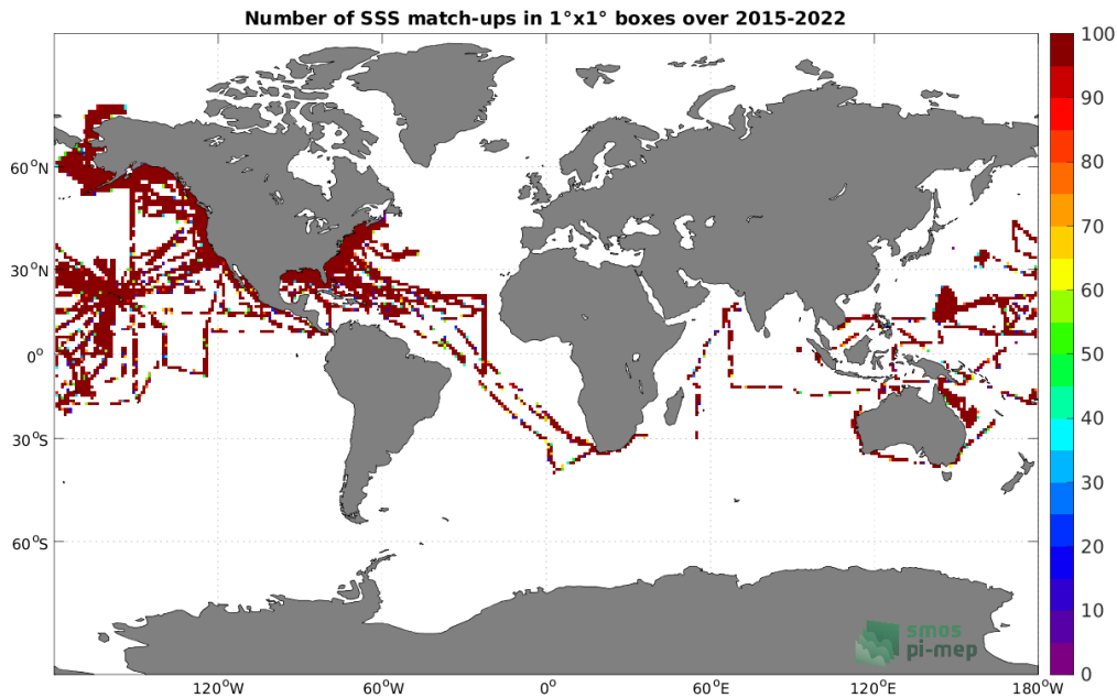
Figure 4: Number of SSS match-ups between TSG (SAMOS) SSS and the SMAP SSS L2 v5.0 (JPL) SSS product for the Global Ocean Pi-MEP region over 1^\circ \times 1^\circ boxes and for the full satellite product period.
