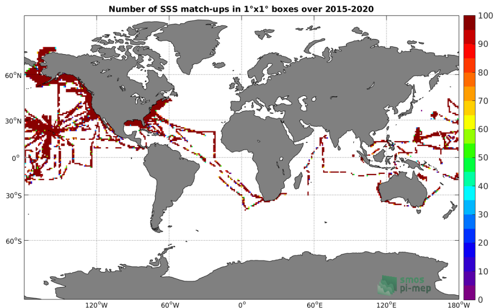
Figure 4: Number of SSS match-ups between TSG (SAMOS) SSS and the SMAP SSS L2 v5.0 (JPL) SSS product for the Global Ocean Pi-MEP region over 1°x1° boxes and for the full satellite product period.
