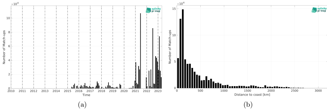
Figure 2: Number of match-ups between TSG (Polarstern) and SMAP SSS L2 v5.0 (JPL) SSS as a function of time (a) and as function of the distance to coast (b) over the Global Ocean Pi-MEP region and for the full satellite product period.
