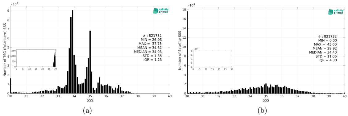
Figure 3: Histograms of SSS from TSG (Polarstern) (a) and SMAP SSS L2 v5.0 (JPL) (b) considering all match-up pairs per bins of 0.1 over the Global Ocean Pi-MEP region and for the full satellite product period.
