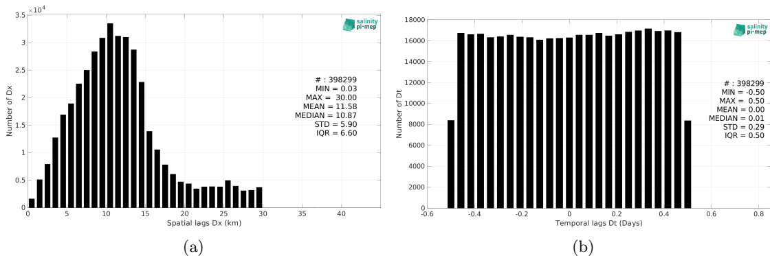
Figure 5: Histograms of the spatial (a) and temporal (b) lags between the location/time of the TSG (Polarstern) measurement and the date of the corresponding SMAP SSS L2 v5.0 (JPL) SSS pixel.
