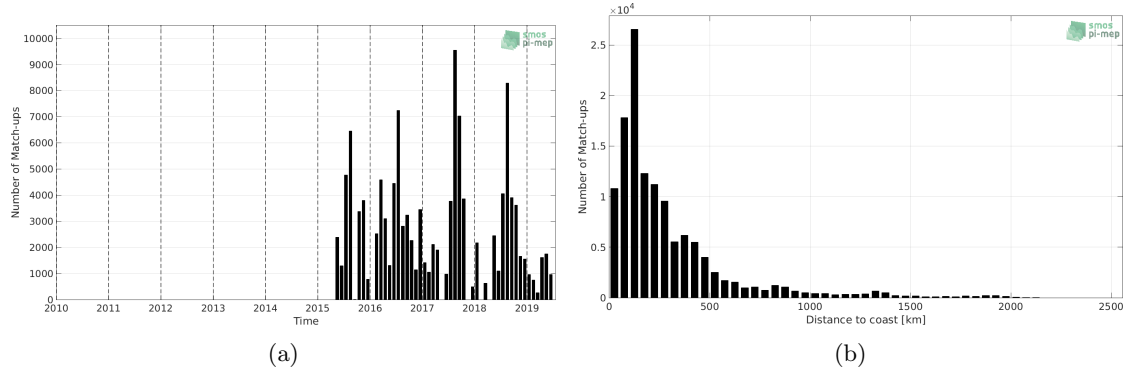
Figure 1: Number of match-ups between TSG (Polarstern) and SMAP SSS L2 v5.0 (JPL) SSS as a function of time (a) and as function of the distance to coast (b) over the Global Ocean Pi-MEP region and for the full satellite product period.
