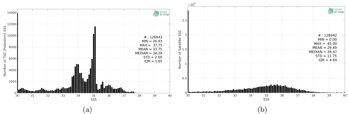
Figure 2: Histograms of SSS from TSG (Polarstern) (a) and SMAP SSS L2 v5.0 (JPL) (b) considering all match-up pairs per bins of 0.1 over the Global Ocean Pi-MEP region and for the full satellite product period.
