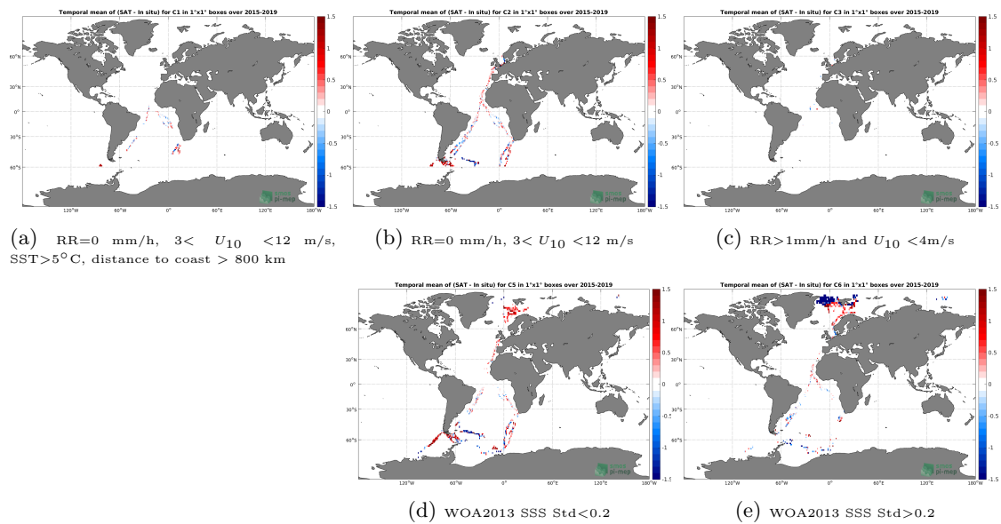
Figure 12: Temporal mean gridded over spatial boxes of size 1^\circ \times 1^\circ of \Delta SSS (SMAP SSS L2 v5.0 (JPL) - TSG (Polarstern)) for 5 different subdatasets corresponding to:RR=0 mm/h, 3 < U_{10} < 12 m/s, SST >5^\circ\text{C} , distance to coast > 800 km (a), RR=0 mm/h, 3 < U_{10} < 12 m/s (b), RR >1 mm/h and U_{10} < 4 m/s (c), WOA2013 SSS Std <0.2 (d), WOA2013 SSS Std >0.2 (e).
