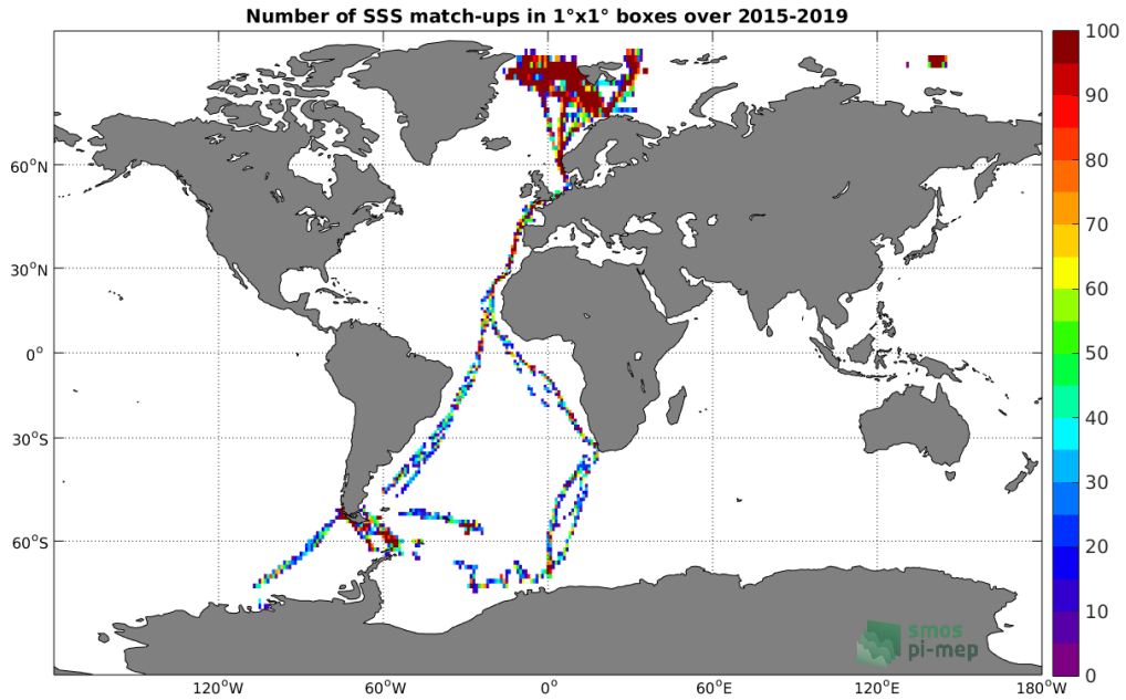
Figure 4: Number of SSS match-ups between TSG (Polarstern) SSS and the SMAP SSS L2 v5.0 (JPL) SSS product for the Global Ocean Pi-MEP region over 1°x1° boxes and for the full satellite product period.
