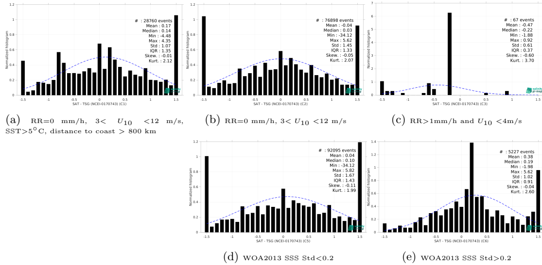
Figure 15: Normalized histogram of \Delta SSS (SMAP SSS L2 v5.0 (JPL) - TSG (NCEI-0170743)) for 5 different subdatasets corresponding to: RR=0 mm/h, 3 < U_{10} < 12 m/s, SST > 5°C, distance to coast > 800 km (a), RR=0 mm/h, 3 < U_{10} < 12 m/s (b), RR > 1mm/h and U_{10} < 4 m/s (c), WOA2013 SSS Std < 0.2 (d), WOA2013 SSS Std > 0.2 (e).
