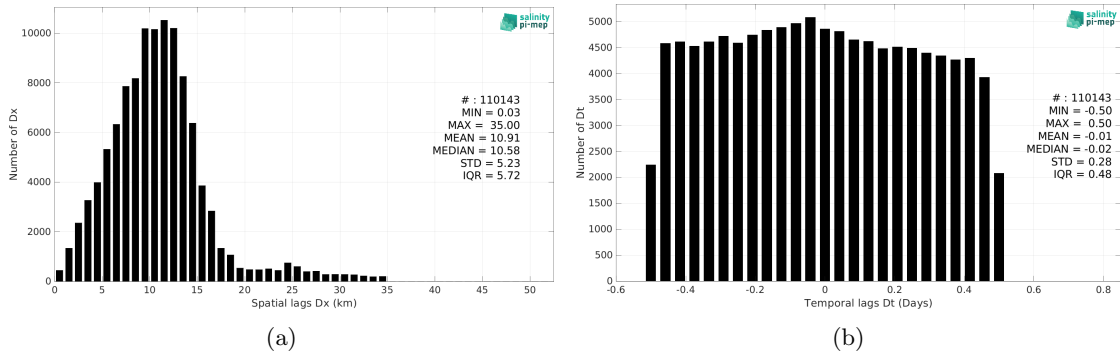
Figure 6: Histograms of the spatial (a) and temporal (b) lags between the location/time of the TSG (NCEI-0170743) measurement and the date of the corresponding SMAP SSS L2 v5.0 (JPL) SSS pixel.
