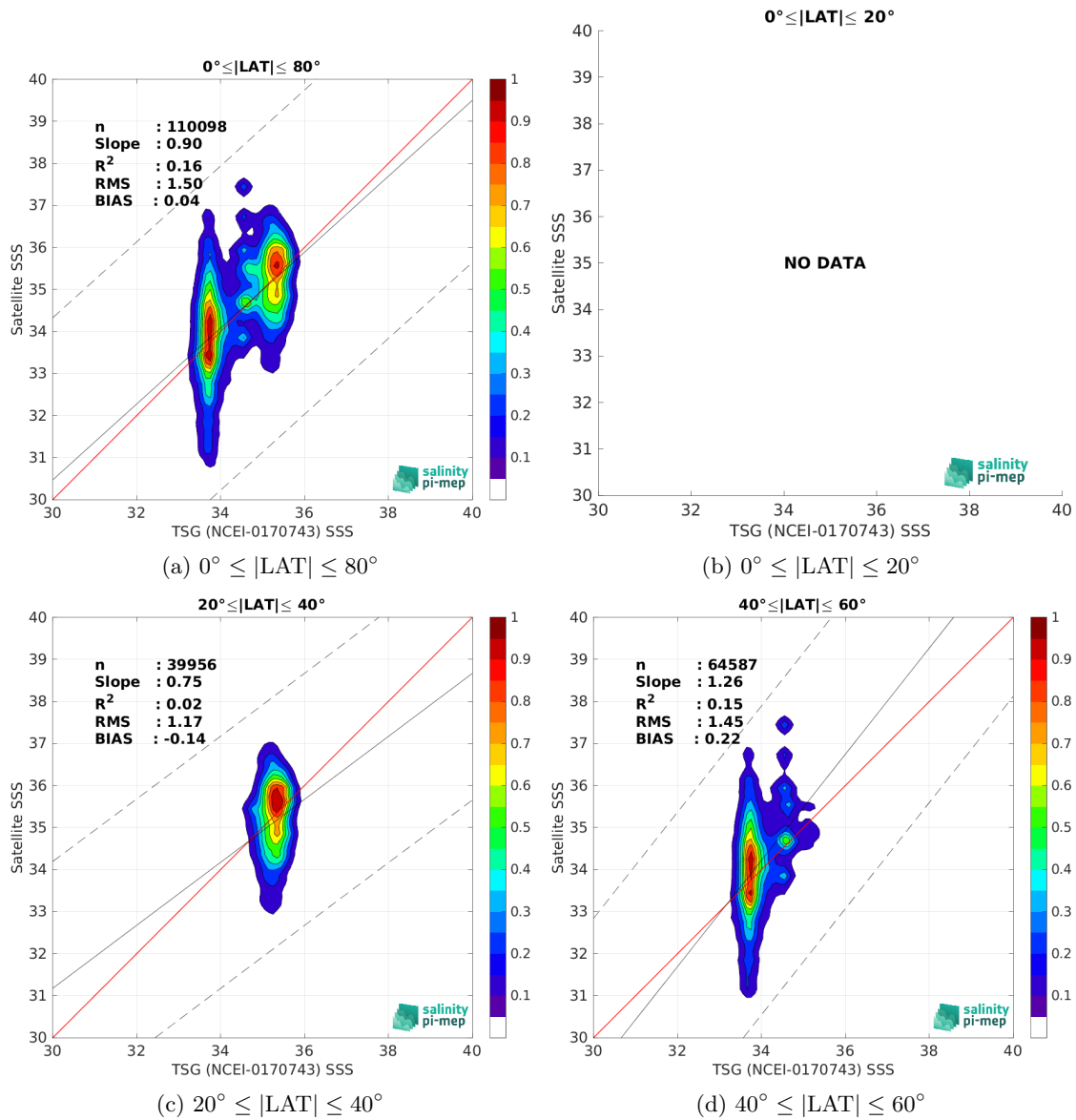
Figure 10: Contour maps of the concentration of SMAP SSS L2 v5.0 (JPL) SSS (y-axis) versus TSG (NCEI-0170743) SSS (x-axis) at match-up pairs for different latitude bands. For each plot, the red line shows x=y . The black thin and dashed lines indicate a linear fit through the data cloud and the \pm 95\% confidence levels, respectively. The number match-up pairs n , the slope and R^2 coefficient of the linear fit, the root mean square (RMS) and the mean bias between satellite and in situ data are indicated for each latitude band in each plots.
