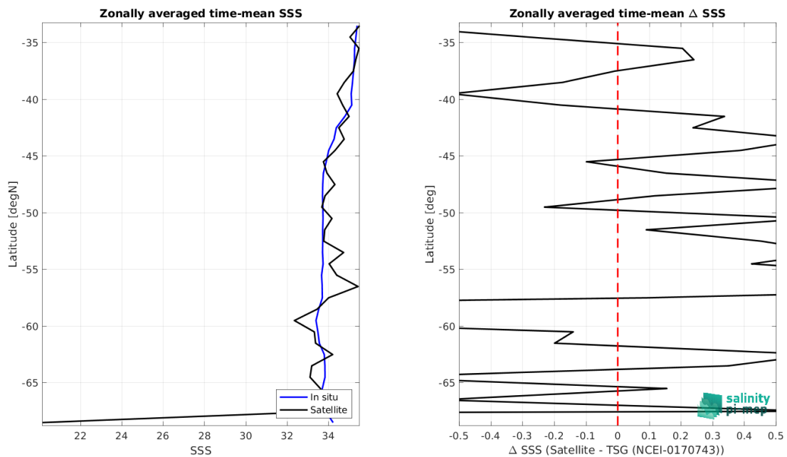
Figure 9: Left panel: Zonal mean SSS from SMAP SSS L2 v5.0 (JPL) satellite product (black) and from TSG (NCEI-0170743) (blue). Right panel: Zonal mean of \Delta SSS (Satellite - TSG (NCEI-0170743)) for all the collected Pi-MEP match-up pairs estimated over the full satellite product period.
