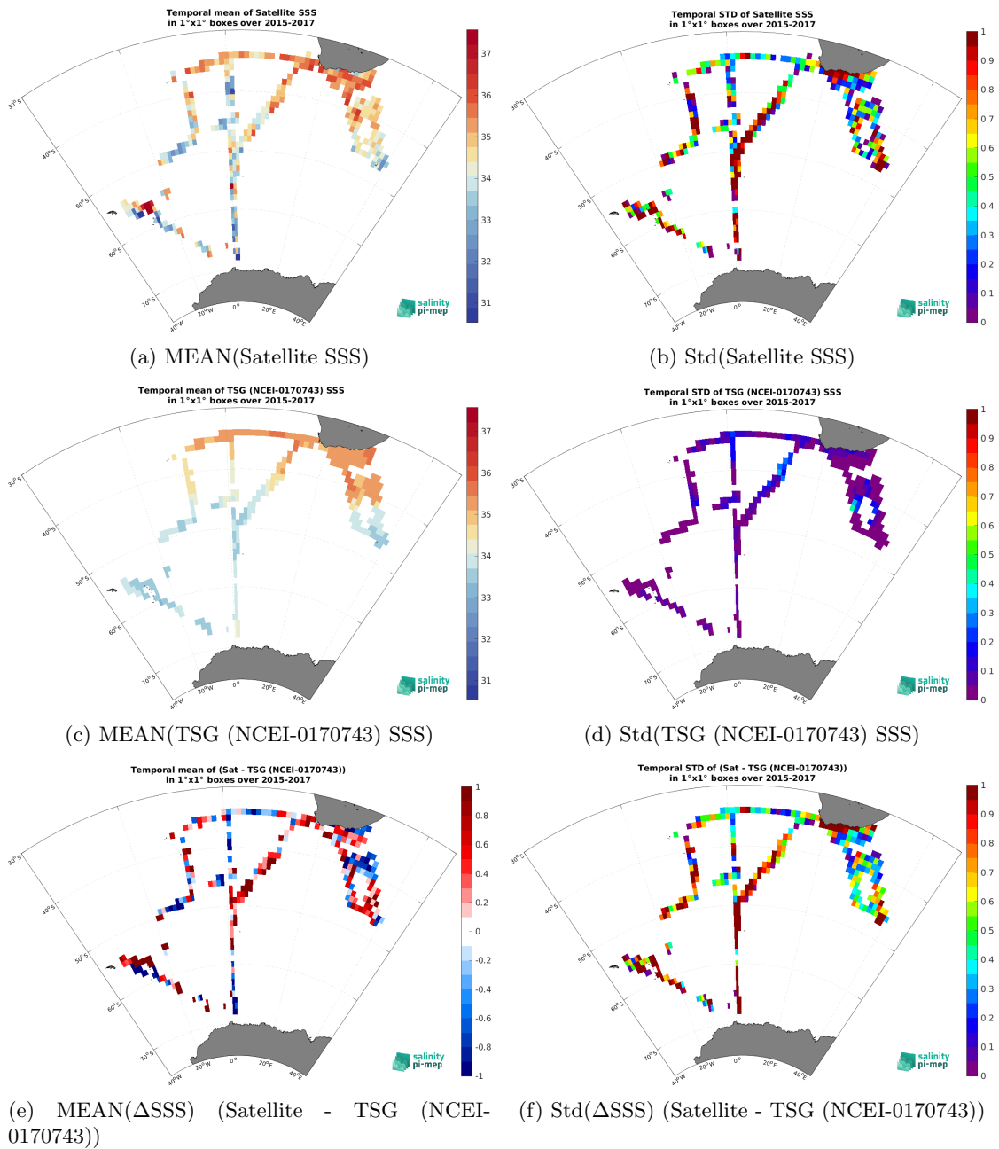
Figure 7: Temporal mean (left) and Std (right) of SSS from SMAP SSS L2 v5.0 (JPL) (top), TSG (NCEI-0170743) (middle), and of \Delta SSS (Satellite - TSG (NCEI-0170743)). Only match-up pairs are used to generate these maps.
