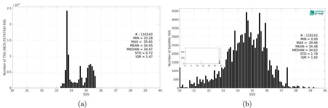
Figure 3: Histograms of SSS from TSG (NCEI-0170743) (a) and SMAP SSS L2 v5.0 (JPL) (b) considering all match-up pairs per bins of 0.1 over the Global Ocean Pi-MEP region and for the full satellite product period.
