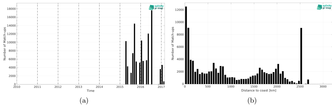
Figure 2: Number of match-ups between TSG (NCEI-0170743) and SMAP SSS L2 v5.0 (JPL) SSS as a function of time (a) and as function of the distance to coast (b) over the Global Ocean Pi-MEP region and for the full satellite product period.
