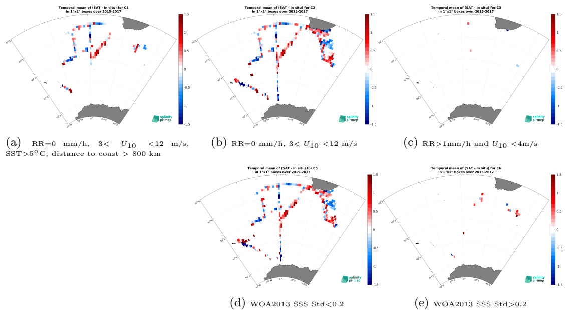
Figure 14: Temporal mean gridded over spatial boxes of size 1^\circ \times 1^\circ of \Delta SSS (SMAP SSS L2 v5.0 (JPL) - TSG (NCEI-0170743)) for 5 different subdatasets corresponding to:RR=0 mm/h, 3 < U_{10} < 12 m/s, SST >5^\circ\text{C} , distance to coast > 800 km (a), RR=0 mm/h, 3 < U_{10} < 12 m/s (b), RR >1 mm/h and U_{10} < 4 m/s (c), WOA2013 SSS Std <0.2 (d), WOA2013 SSS Std >0.2 (e).
