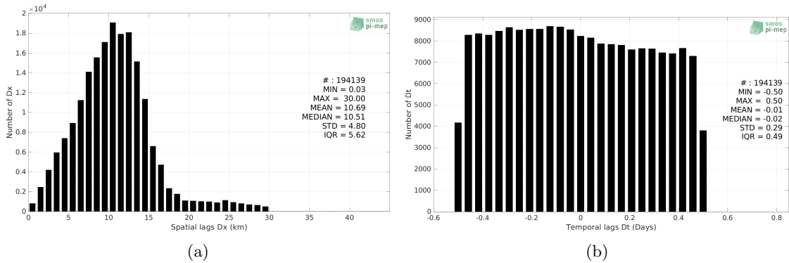
Figure 5: Histograms of the spatial (a) and temporal (b) lags between the location/time of the TSG (NCEI-0170743) measurement and the date of the corresponding SMAP SSS L2 v5.0 (JPL) SSS pixel.
