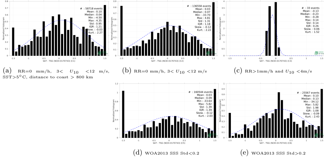
Figure 13: Normalized histogram of \Delta SSS (SMAP SSS L2 v5.0 (JPL) - TSG (NCEI-0170743)) for 5 different subdatasets corresponding to: RR=0 mm/h, 3 < U_{10} < 12 m/s, SST>5°C, distance to coast > 800 km (a), RR=0 mm/h, 3 < U_{10} < 12 m/s (b), RR>1mm/h and U_{10} < 4 m/s (c), WOA2013 SSS Std<0.2 (d), WOA2013 SSS Std>0.2 (e).
