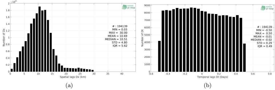
Figure 5: Histograms of the spatial (a) and temporal (b) lags between the time of the TSG (NCEI-0170743) measurements and the date of the corresponding SMAP SSS L2 v5.0 (JPL) SSS product.
