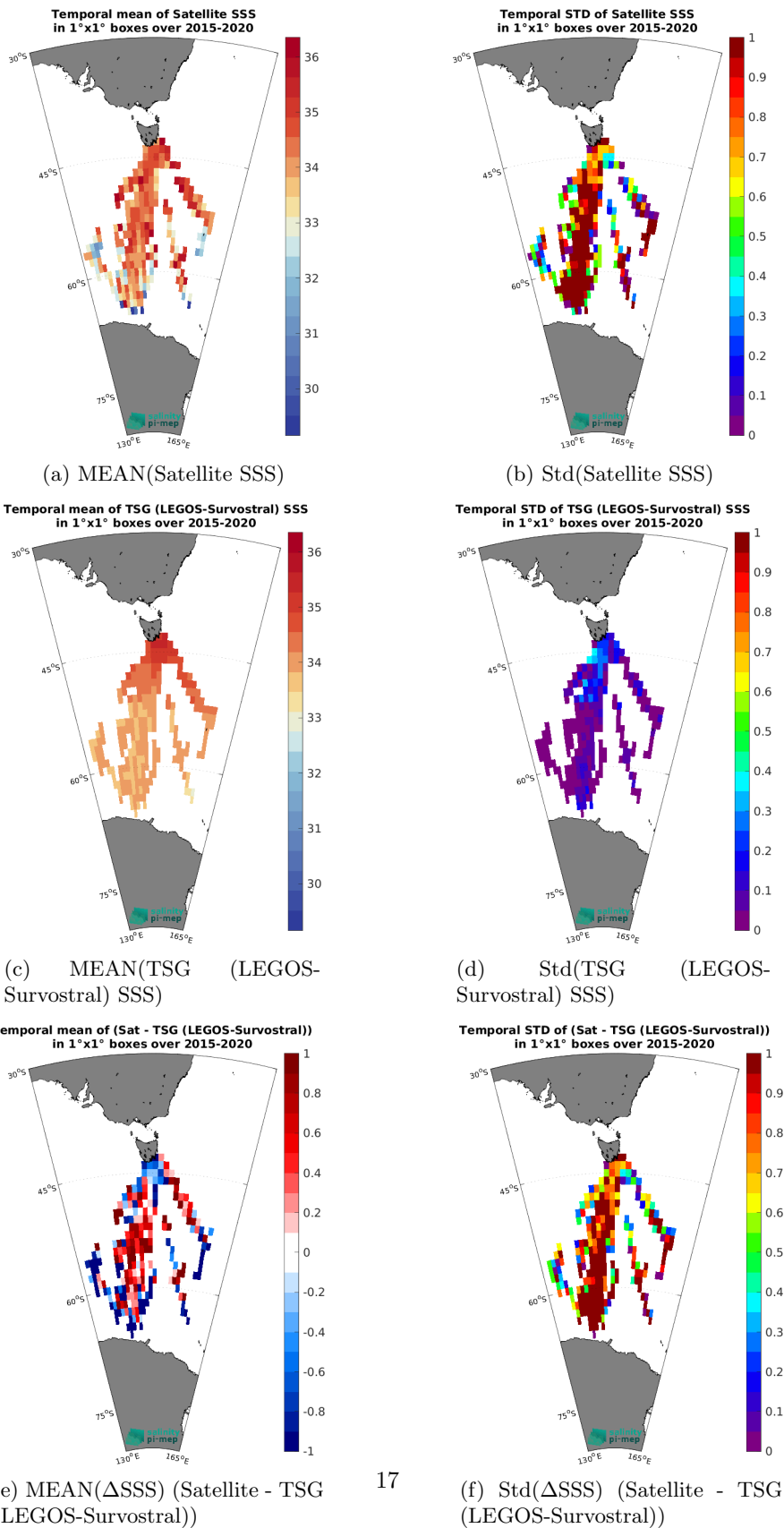
Figure 7: Temporal mean (left) and Std (right) of SSS from SMAP SSS L2 v5.0 (JPL) (top), TSG (LEGOS-Survostral) (middle), and of \Delta SSS (Satellite - TSG (LEGOS-Survostral)). Only match-up pairs are used to generate these maps.
