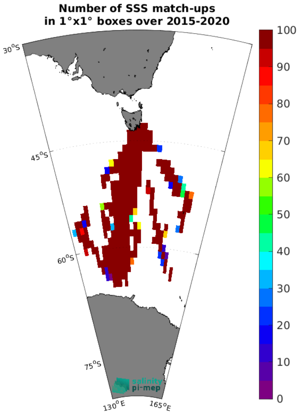
Figure 5: Number of SSS match-ups between TSG (LEGOS-Survostral) SSS and the SMAP SSS L2 v5.0 (JPL) SSS product for the Global Ocean Pi-MEP region over 1°×1° boxes and for the full satellite product period.
