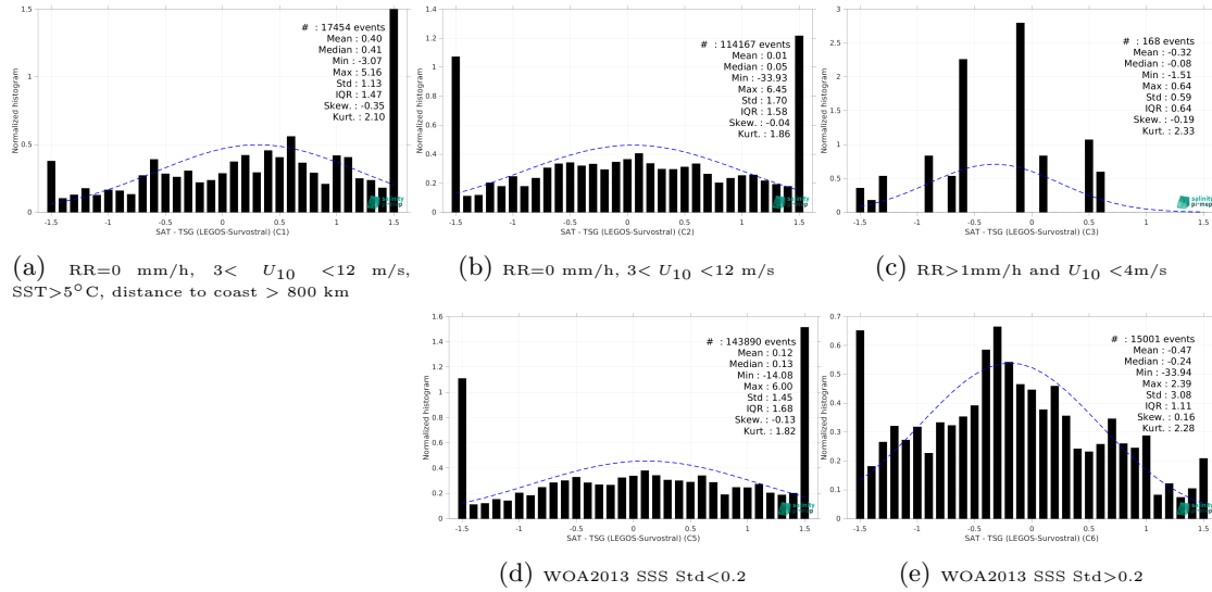
Figure 15: Normalized histogram of \Delta SSS (SMAP SSS L2 v5.0 (JPL) - TSG (LEGOS-Survostral)) for 5 different subdatasets corresponding to: RR=0 mm/h, 3 < U_{10} < 12 m/s, SST > 5°C, distance to coast > 800 km (a), RR=0 mm/h, 3 < U_{10} < 12 m/s (b), RR > 1mm/h and U_{10} < 4 m/s (c), WOA2013 SSS Std < 0.2 (d), WOA2013 SSS Std > 0.2 (e).
