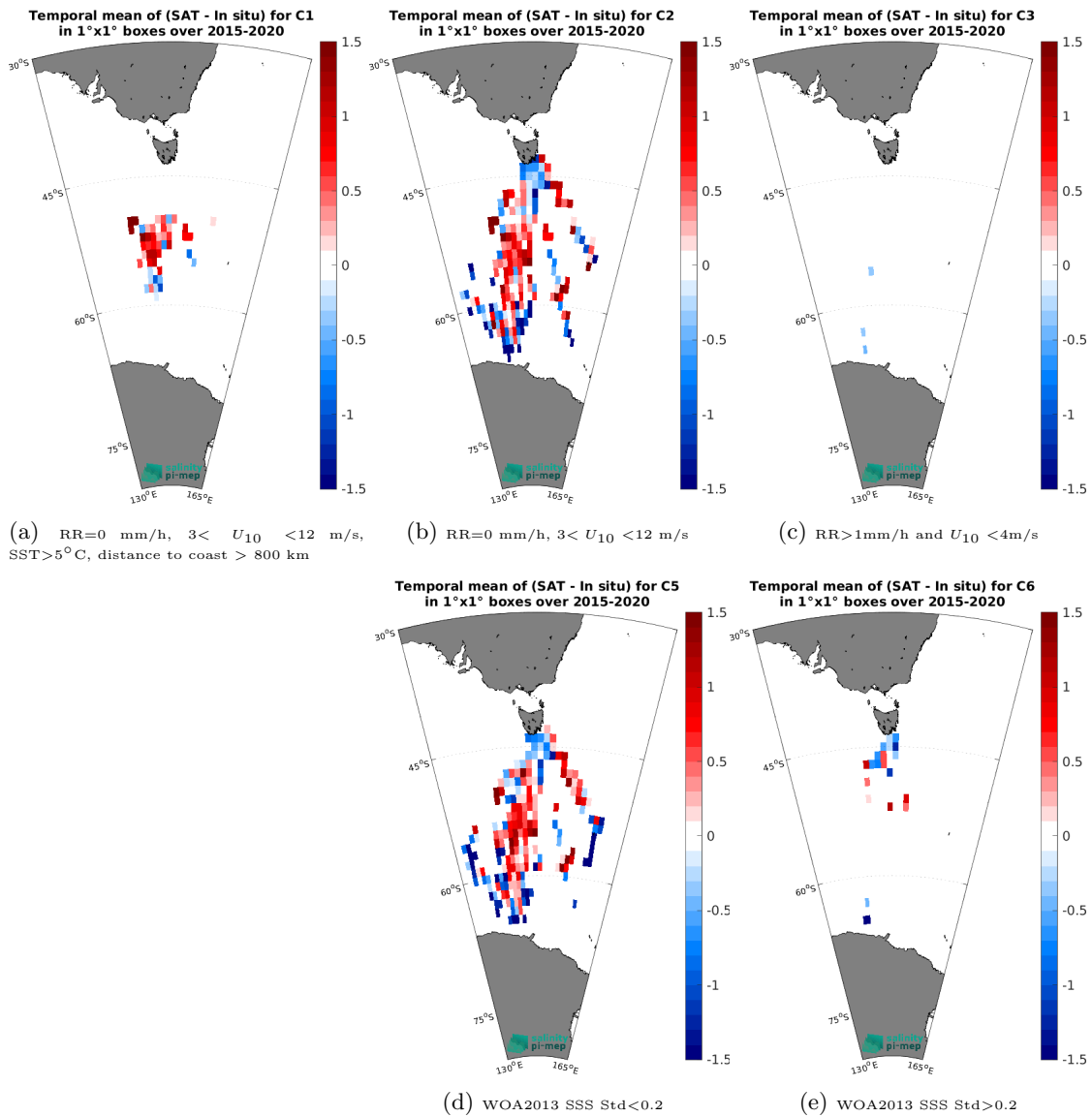
Figure 14: Temporal mean gridded over spatial boxes of size 1^\circ \times 1^\circ of \Delta SSS (SMAP SSS L2 v5.0 (JPL) - TSG (LEGOS-Survostral)) for 5 different subdatasets corresponding to:RR=0 mm/h, 3 < U_{10} < 12 m/s, SST>5°C, distance to coast > 800 km (a), RR=0 mm/h, 3 < U_{10} < 12 m/s (b), RR>1mm/h and U_{10} < 4 m/s (c), WOA2013 SSS Std<0.2 (d), WOA2013 SSS Std>0.2 (e).
