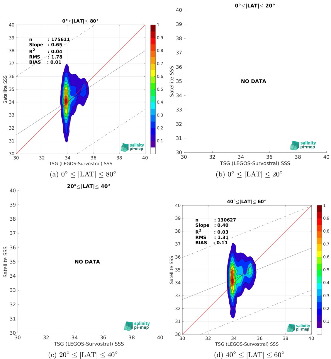
Figure 10: Contour maps of the concentration of SMAP SSS L2 v5.0 (JPL) SSS (y-axis) versus TSG (LEGOS-Survostral) SSS (x-axis) at match-up pairs for different latitude bands. For each plot, the red line shows x=y . The black thin and dashed lines indicate a linear fit through the data cloud and the \pm 95\% confidence levels, respectively. The number match-up pairs n , the slope and R^2 coefficient of the linear fit, the root mean square (RMS) and the mean bias between satellite and in situ data are indicated for each latitude band in each plots.
