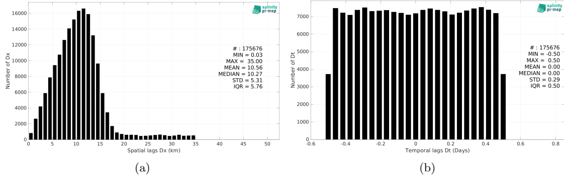
Figure 6: Histograms of the spatial (a) and temporal (b) lags between the location/time of the TSG (LEGOS-Survostral) measurement and the date of the corresponding SMAP SSS L2 v5.0 (JPL) SSS pixel.
