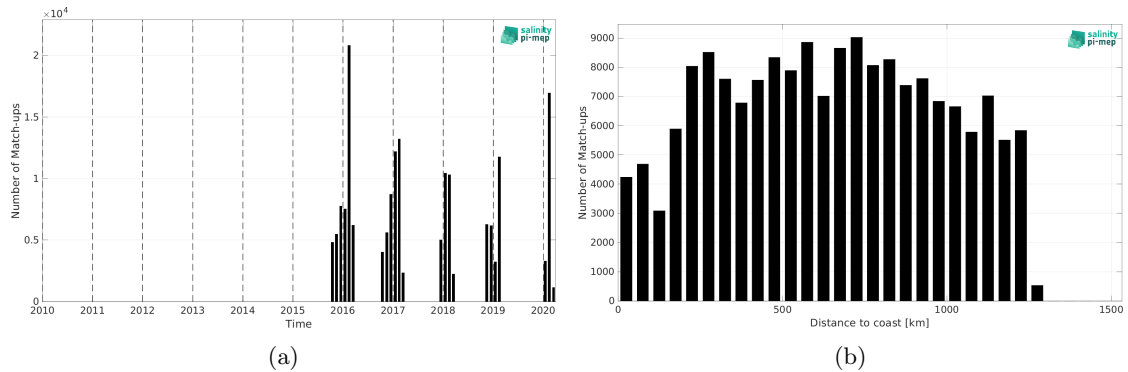
Figure 2: Number of match-ups between TSG (LEGOS-Survostral) and SMAP SSS L2 v5.0 (JPL) SSS as a function of time (a) and as function of the distance to coast (b) over the Global Ocean Pi-MEP region and for the full satellite product period.
