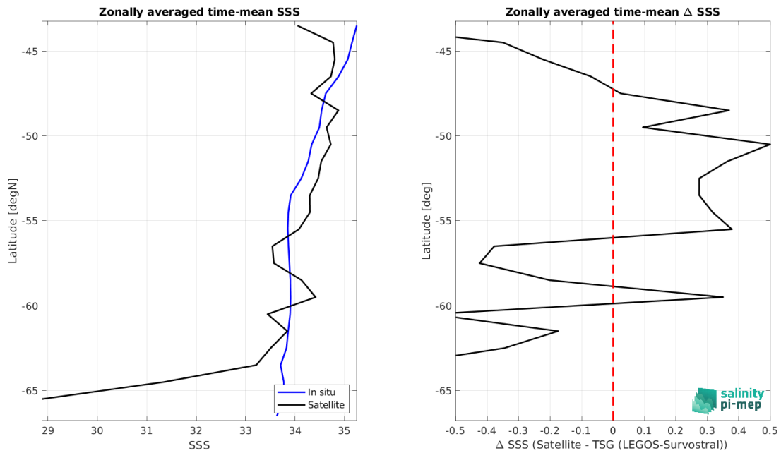
Figure 9: Left panel: Zonal mean SSS from SMAP SSS L2 v5.0 (JPL) satellite product (black) and from TSG (LEGOS-Survostral) (blue). Right panel: Zonal mean of \Delta SSS (Satellite - TSG (LEGOS-Survostral)) for all the collected Pi-MEP match-up pairs estimated over the full satellite product period.
