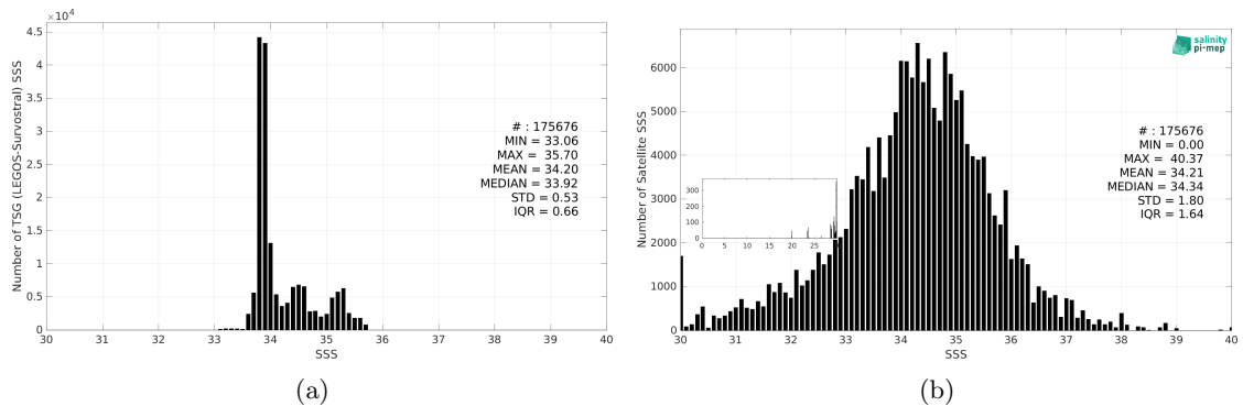
Figure 3: Histograms of SSS from TSG (LEGOS-Survostral) (a) and SMAP SSS L2 v5.0 (JPL) (b) considering all match-up pairs per bins of 0.1 over the Global Ocean Pi-MEP region and for the full satellite product period.
